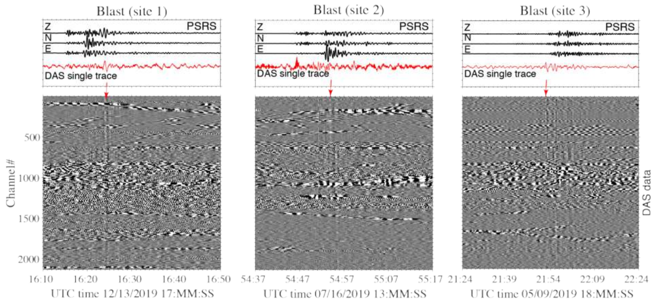
Figure 13. Seismic station (PSRS) and DAS recordings of three quarry blast signals from 3 mining sites (site 1, site 2, and site 3). Their magnitudes from Pennsylvania seismic network catalog are M1.3, M1.7, and M2.0. Red arrows indicate strong surface wave arrivals.
