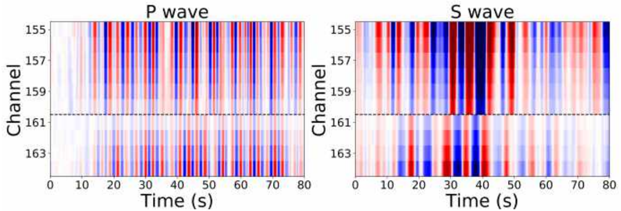
Figure 9. P wave and S wave traces observed in two orthogonal fibers (marked by dashed line in Figure 4a). There is a polarity flip of S wave.
