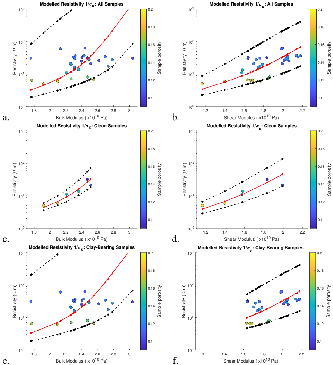
Figure 6: Core measurements (circles) of the Han data set (top row) and its clean (middle row) and clay-bearing (bottom row) sample subsets are modelled by inverting equations 20 and 21 (red diamonds) using optimal aspect ratios shown in Table 3. Resistivities 1/\sigma_K (left column) and 1/\sigma_\mu (right column) are modelled using parameters \alpha_K^* and \alpha_\mu^* respectively. The 95% confidence intervals on initial EPAR estimates are propagated (black points). Measured sample porosity (marker colour) is also shown for context. Lines connect individual inversion results to obviate possible trends.
