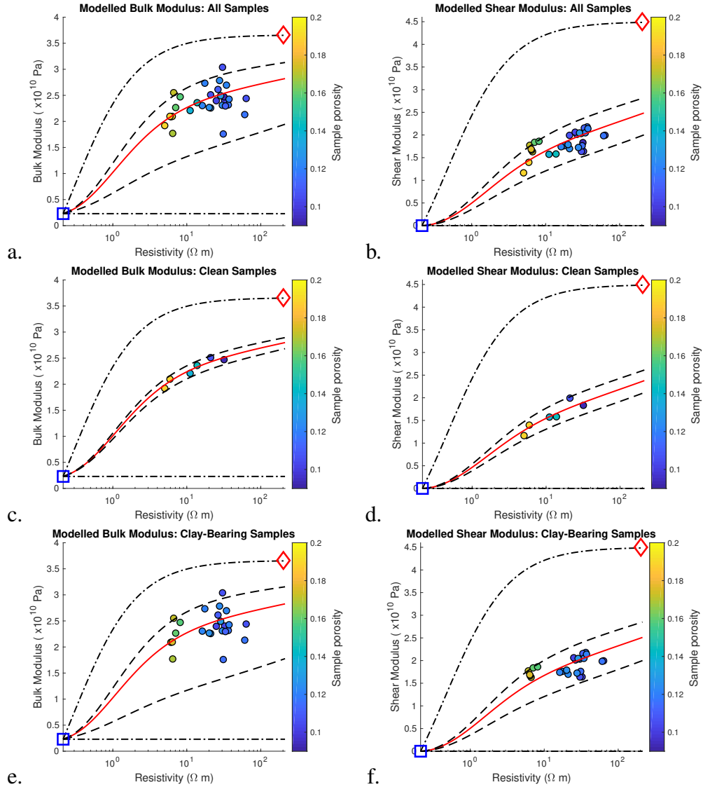
Figure 4: The elastic measurements (circles) of the Han data set and its clean and clay-bearing sample subsets are modelled by solving equations 20 and 21 (red trends) using optimal aspect ratios shown in Table 3. Bulk modulus (left column) and shear modulus (right column) are modelled using parameters \alpha_K^* and \alpha_\mu^* respectively. The 95% confidence intervals on initial EPAR estimates, shown in Figures 2 and 3, are forward modelled (dashed curves). The electrical-elastic upper and lower Hashin-Shtrikman bounds are displayed (dot-dashed curves). The electrical-elastic model converges exactly to the properties of water (blue square) at 100% porosity and \sigma^* = \sigma_2 . It also converges to the properties of matrix material when \sigma^* = \sigma_1 and porosity is zero (asymptotic modulus value shown by red diamond). Measured sample porosity (marker colour) is also shown for context.
