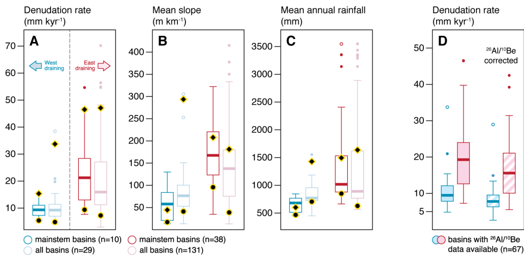
Figure 5: ^{10}\text{Be} -derived denudation rates, mean slope, and mean annual rainfall, east and west of the continental divide. (A-C) Black diamonds and black circles represent the median of denudation rate, mean slope, and mean annual for basins with the 10% highest (diamonds) and 10% lowest (circles) denudation rates, respectively. Slope was extracted from a 90 m resolution SRTM DEM. (D) ^{10}\text{Be} -derived denudation rates (solid fill) and ^{26}\text{Al}/^{10}\text{Be} burial corrected denudation rates (striped pattern) east and west of the continental divide for samples where both ^{26}\text{Al} and ^{10}\text{Be} data are available. See text for more details.
