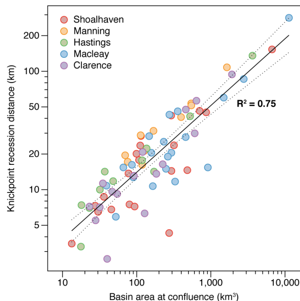
Figure 11: Relationship between knickpoint recession distance measured from confluence and basin area at confluence. Data includes both tributary and mainstem rivers east of the continental divide from five basins characterised by embayed escarpments and large-scale knickpoints along both mainstem and tributary rivers. For mainstem rivers both distance and area are calculated from the outlet defined by the present sea level. Knickpoints were identified based on distance-slope (DS) plots [Goldrick & Bishop, 2007] using a 30 m SRTM DEM.
