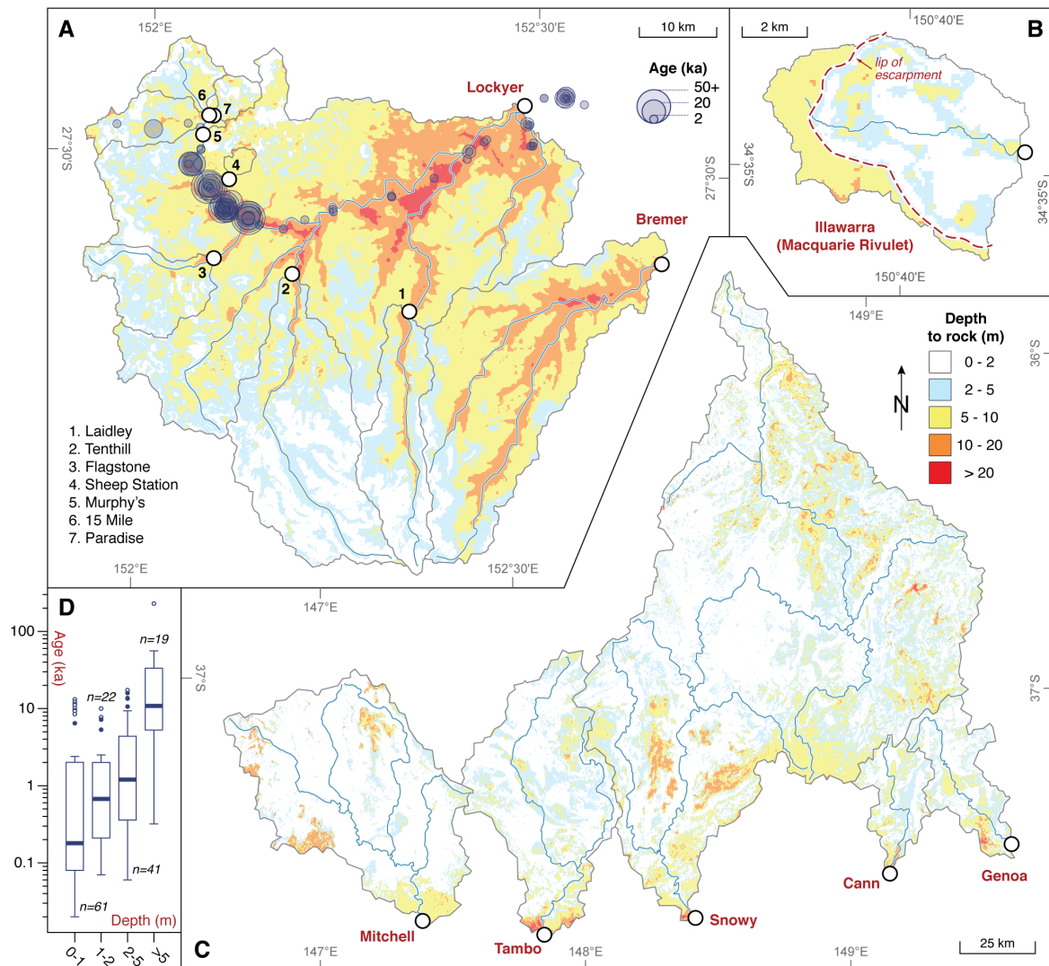
Figure 12: Depth-of-regolith maps for selected basins. (A) to (C) Maps showing the distribution of regolith thickness in basins from south-east Queensland (A), Illawarra (B), and southern Victoria (C) calculated using Wilford et al.'s [2015] depth-of-regolith data. (D) Box plots showing optically stimulated luminescence (OSL) ages of alluvial units vs. their depth from the Lockyer River. Data from Croke et al. [2016] and Daley et al. [2017]. Location of samples and spatial distribution of ages are shown in (A).
