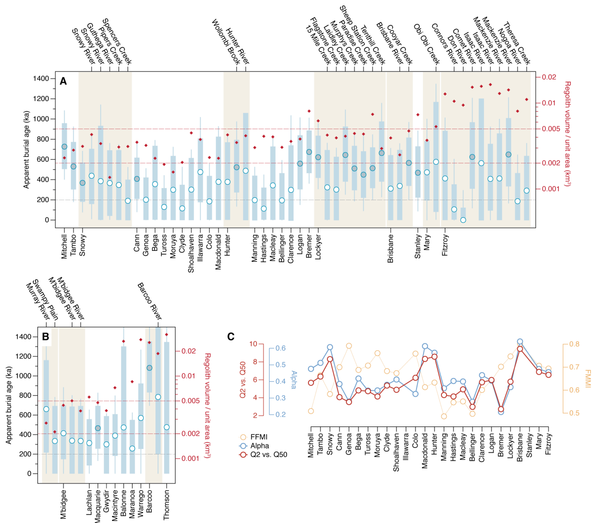
Figure 8: ^{26}\text{Al}/^{10}\text{Be} apparent burial ages. (A) and (B) Apparent burial ages (circles) for samples east (A) and west (B) of the continental divide, respectively. Whiskers indicate age uncertainties at the 95% confidence level and darker blue boxes indicate age uncertainties at the 68% confidence level. Blue circles are apparent burial ages that are distinguishable from zero at the 95% confidence level. Red diamonds represent regolith volume per unit basin area, calculated using Wilford et al.'s [2015] depth-of-regolith data. Ivory vertical bands group samples belonging to the same mainstem basin such that basin names on bottom x-axis are mainstem samples only. Red and grey dashed lines are to guide the eye. (C) Flood variability metrics for basins east of the continental divide calculated using data from Rustomji et al. [2009]. FFMI: mean flash flood magnitude index calculated using the monthly peaks-over-threshold flood series; Alpha: mean power law scaling coefficient; Q2 vs. Q50: mean flood quantile ratio. Alpha and Q2 vs. Q50 are the recommended metrics by Rustomji et al. [2009], and FFMI is shown only for completeness.
