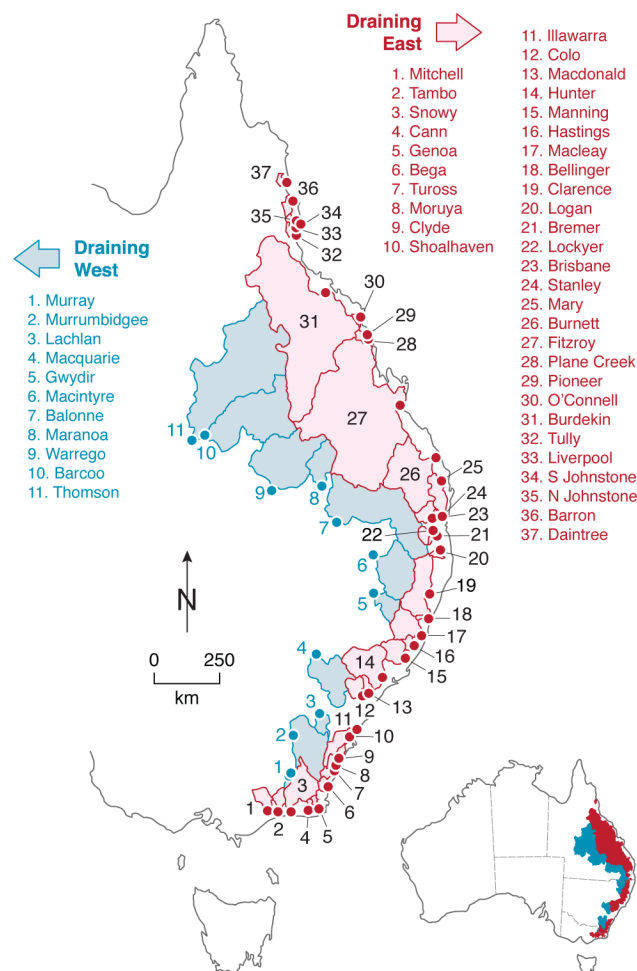
Figure 2: Distribution of east and west draining basins included in this study. The study area stretches about 3,000 km along the East Australian margin and basins range in area between 35 – 139,000 km 2 (east) and 3,300 – 150,000 km 2 (west). See Figure 3 for map of tributary basins and Table S1 for further detail.
