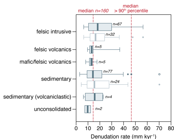
Figure 10: 10 Be-derived denudation rates grouped by dominant lithology. Dashed vertical lines indicate the median of all denudation rates and the median of denudation rates above the 90 th percentile, respectively. White box plots show only data for basins < 150 km 2 . Predominant rock-type in each basin was calculated using the Geoscience Australia 1:2.5 million scale Surface Geology of Australia digital dataset [Raymond et al., 2012].
