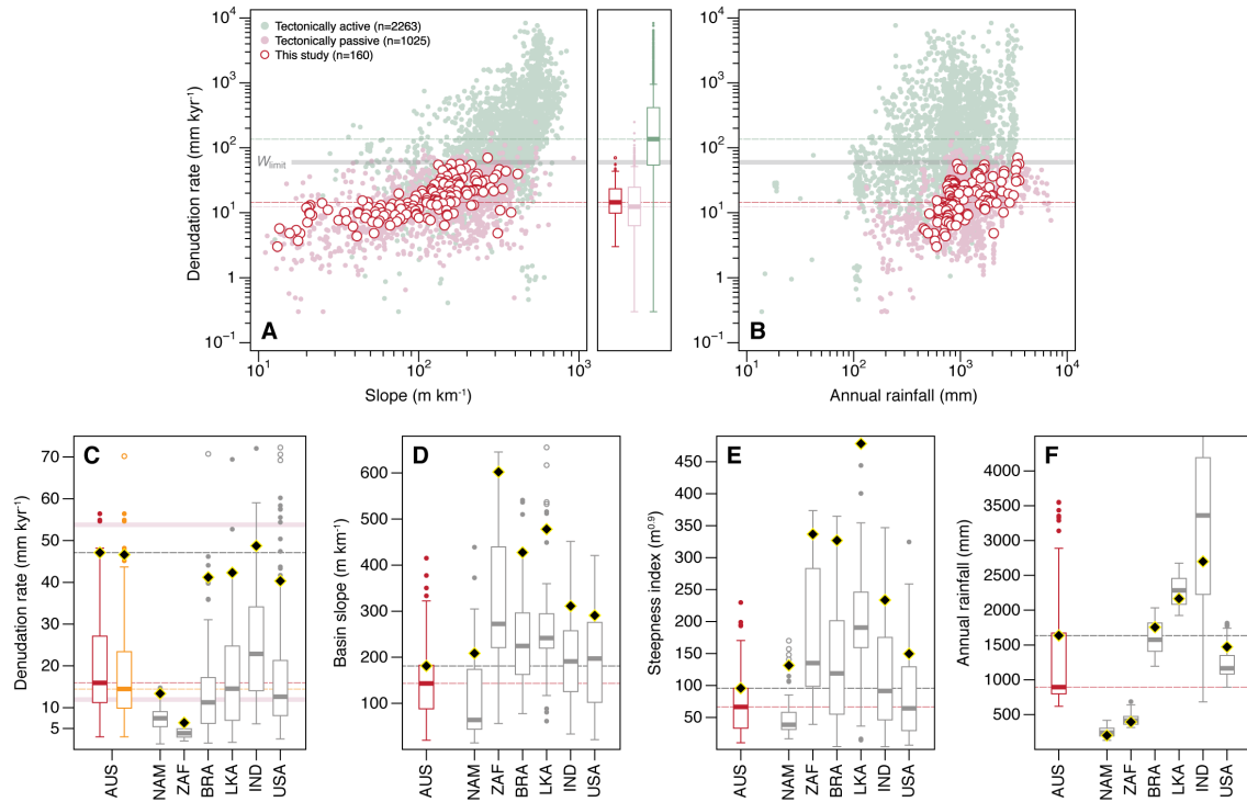
Figure 9: East Australian denudation rates in a global context. (A) and (B) ^{10}\text{Be} -derived denudation rate vs. mean basin slope (A) and mean annual rainfall (B), comparing data from the East Australian margin with the global denudation rates from the OCTOPUS database. Dashed horizontal lines are median values: light magenta – basins from tectonically passive settings, light green – basins from tectonically active settings, red – this study. Horizontal grey band ( W_{\text{limit}} ) represents the silicate weathering speed limit (i.e., 151 \text{ t km}^{-2} \text{ yr}^{-1} or approx. 58 \text{ mm kyr}^{-1} ) from Dixon & von Blanckenburg [2012]). (C) – (F) Box plots showing ^{10}\text{Be} -derived denudation rates (C), mean basin slope (D), mean normalised channel steepness ( k_{sn} ) (E), and mean annual rainfall (F) for basins from this study (AUS) and other passive continental margin settings: Namibia (NAM), South Africa (ZAF), Eastern Brazil (BRA), Sri Lanka (LKA), Western Ghats (IND), and the Appalachian Mountains (USA). Red box plots show data for Australian basins to the east of the continental divide and orange box plot includes data from both sides of the divide. Black diamonds represent the median of denudation rate, mean slope, mean k_{sn} , and mean annual precipitation, respectively, for basins with the 10% highest denudation rates. Red (and orange) horizontal dashed lines represent median values for all Australian datapoints and black horizontal dashed lines represent median values calculated only for Australian basins with the 10% highest denudation rates. Light magenta horizontal bands in (C) represent median denudation rate values for all tectonically passive basins (lower band) and for those with the 10% highest denudation rates (upper band). Topographic metrics were extracted from a 90 m resolution SRTM DEM. See text for more details.
