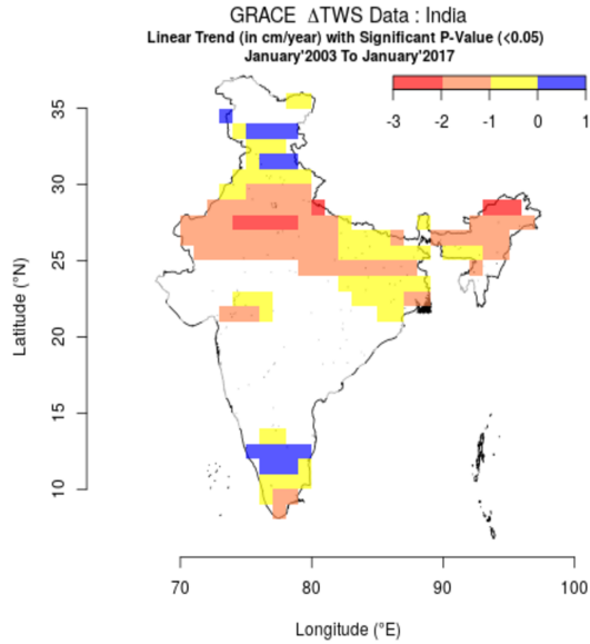
(a) Grid points with significant linear trend in \Delta TWS (2003-2017)
