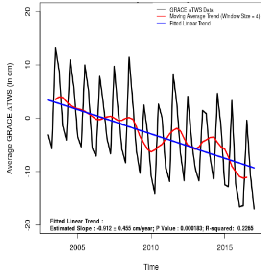
(b) Quarterly average \Delta TWS for Ganga-Brahmaputra river basin & North-West India (2003-2017)
