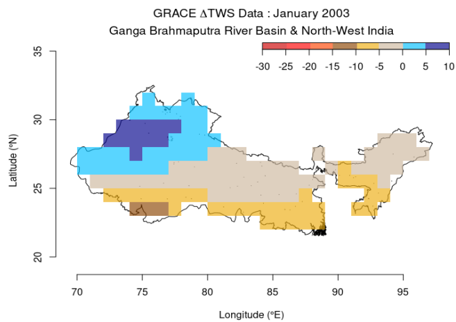
(a) \Delta TWS : January 2003
