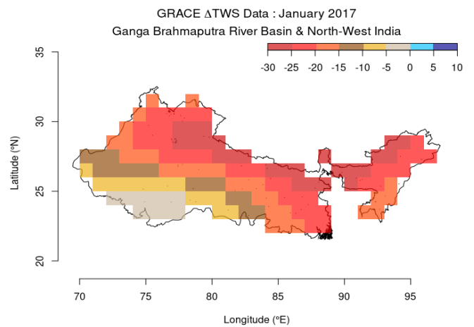
(b) \Delta TWS : January 2017
