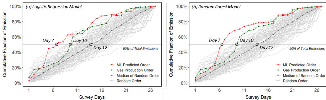
Figure 2: Time evolution of cumulative fraction of emissions detected across the three survey scenarios. The x-axis shows number of days and the y-axis shows the cumulative fraction of emissions covered.
