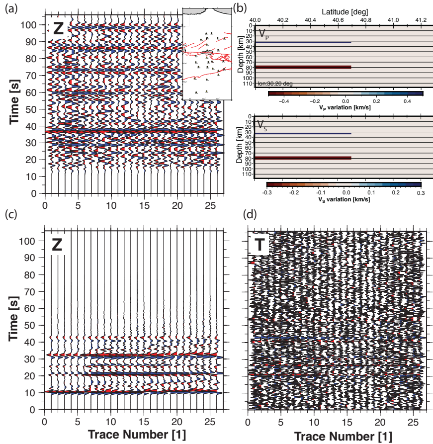
Figure 4. Example data and synthetics. (a) Recorded data example of vertical component of event 20123211812 (insert shows station configuration). Data are cut to 100 s and tapered. The direct P-arrival is suppressed. (b) North-South slices through perturbation model to calculate synthetics. (c) Noiseless synthetics (vertical) through perturbation model shown in b), including all scattering events from direct wave and free surface reflections. Synthetics represent the event-station configuration of the quality-controlled receiver functions for event 20123211812 shown in a). Although the perturbation is not continuous throughout the model, the scattered wavefield can be recorded across the network with distinctive moveout allowing the localisation of the perturbation. (d) Transverse component of the synthetic data calculated for model shown in (b) with added noise. We add Gaussian noise with a 10% standard deviation relative to the maximum signal amplitude to the synthetic data.
