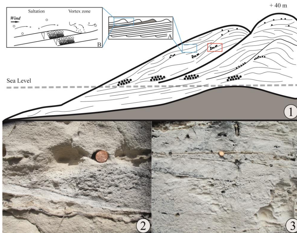
Figure 3: 1—Changing morphology of fenestrae-rich beds within chevron dunes, going from abundant tabular to slight discontinuous packages with increasing distance and elevation from shore (modified after (Hearty and Tormey, 2017). Red square indicates the position of 2 and 3. A—Subcritically translant strata (SCTS) forming when the angle of ripple climb is lower than the inclination of ripple stoss slope (modified after Hunter, 1977). B—Formation mechanism of pine stripe laminations showing inverse grain size gradient by concentration of finer particles in the existing trough between two ripples (modified after (Fryberger and Schenk, 1988). 2 and 3—Photographs of fenestrae-rich beds of a dozen cm thick within an eolianite subparallel to the coast. Note the more pronounced pinstripe laminations within the bed rich in fenestrae in 2.
