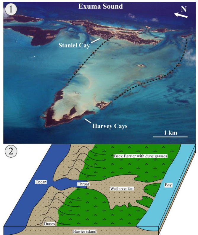
Figure 7: 1— Aerial photograph of a partially eroded chevron near Staniel Cay in the Exumas, Bahamas (photo from P. Kindler). 2— Comparison with a typical washover fan morphology on a barrier island (modified after (Donnelly et al., 2006).
