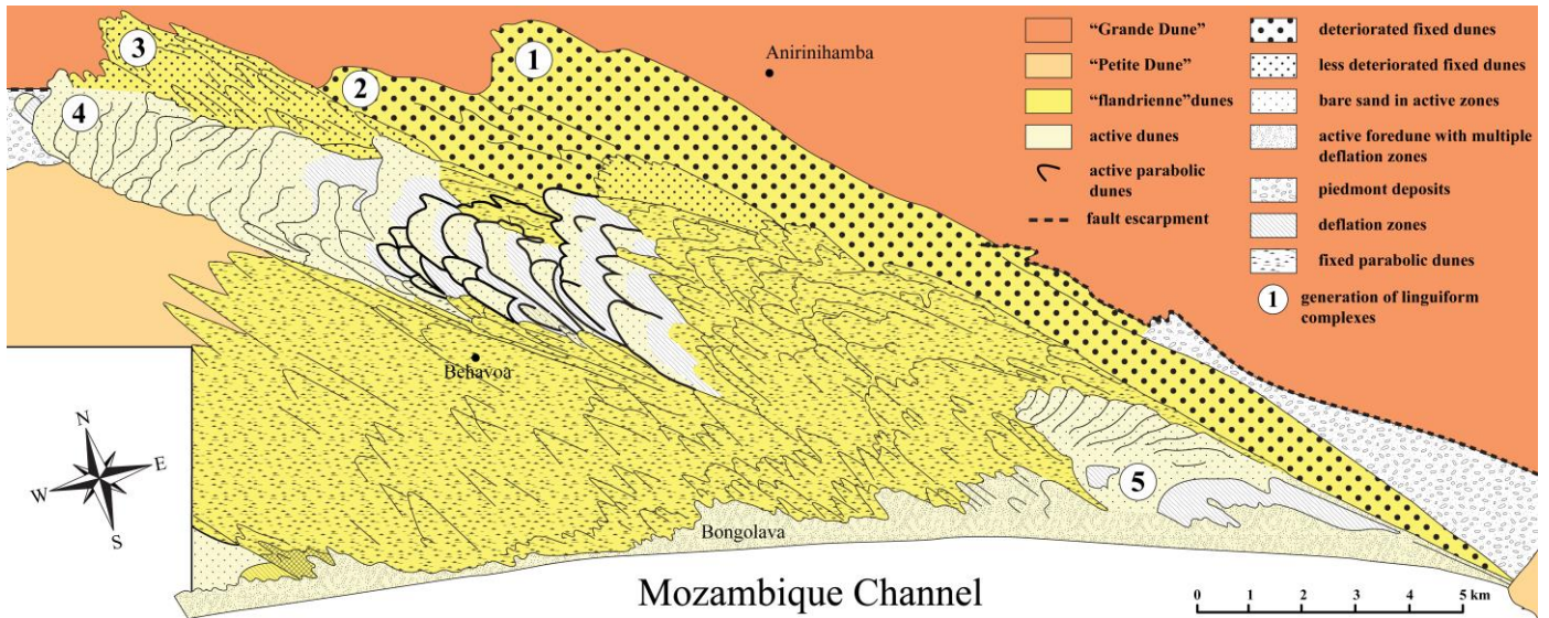
Figure 4: Geomorphological features and stratigraphic relationships of the different units composing the Fenambosy chevron (modified after Battistini, 1964). The “Grande Dune” is the oldest sandy unit in S-Madagascar coastline environment, correlated to the ancient “Aepyomien” (from 2.2 Myrs to 160’000 yrs BP). The “Petite Dune” unit corresponds to the “karimbolien” deposits (120’000-45’000 yrs BP). The “flandrienne” dunes are Holocene (6’000 yrs BP) transgression-related sandy deposits that form the chevrons in the region. The active recent dunes are depositing as foredunes on which few nebkhas can be observed. The numbers represent the different phases of deposition from the oldest (generation 1) to the youngest (generation 5).
