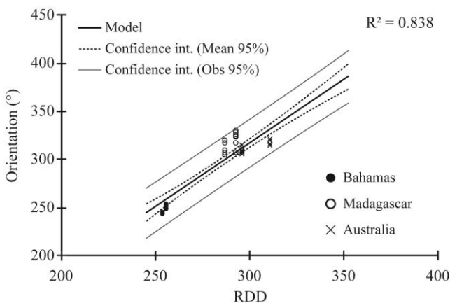
Figure 10: Linear regression model for chevrons azimuths on RDD showing a strong correlation between the two variables.
