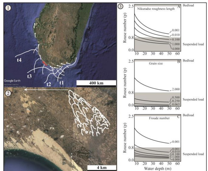
Figure 5: 1— Satellite photograph of the southern part of Madagascar. The arrows show the chevrons orientations, and specifically the Ampalaza chevron (red arrow). The timelines of wave crests modeled by Bourgeois and Weiss (2009) are represented by the uniform white lines, and angles of wave approach by arrowed ones. 2— Enhancement of the Ampalaza chevron with the main ridges outlined in white (Bourgeois and Weiss, 2009), showing the general orientation subparallel to the coast. 3— Plots of Rouse number (p) versus water depth to show the type of sediment transport under varying k_s (A), D (B) and Fr (C) represented by the lines (Bourgeois and Weiss, 2009). Grain size is kept constant ( D = 1 mm) in A for all cases; as Fr = 1.0 and k_s = 1 m in B; plus D = 1 mm and k_s = 1 m in C.
