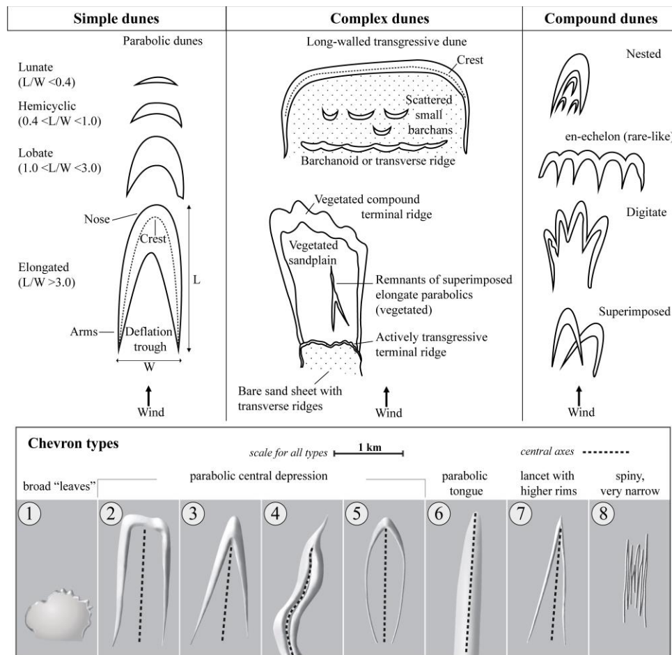
Figure 2: The three types of dunes defined by McKee (1979) and the subclassification of simple dunes according to their length:width ratio (Pye, 1993). Comparison with the eight types of chevron morphology observable around the world (modified after Scheffers et al., 2008).
