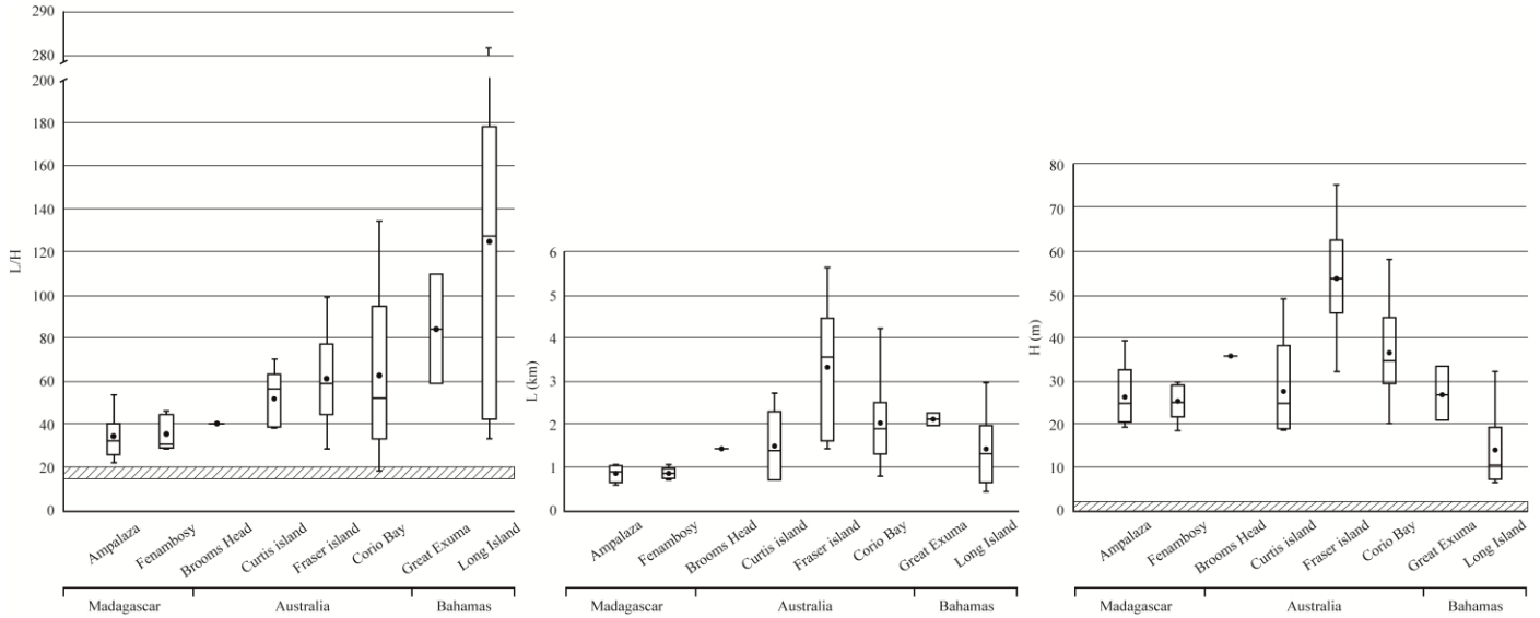
Figure 8: Distribution of L, H and L/H ratios for each location of the three studied regions where stripped zones indicate the range of subaqueous dunes, after Bourgeois and Weiss (2009), for each parameter. It does not appear on the L graph because of a much smaller order of magnitude.
