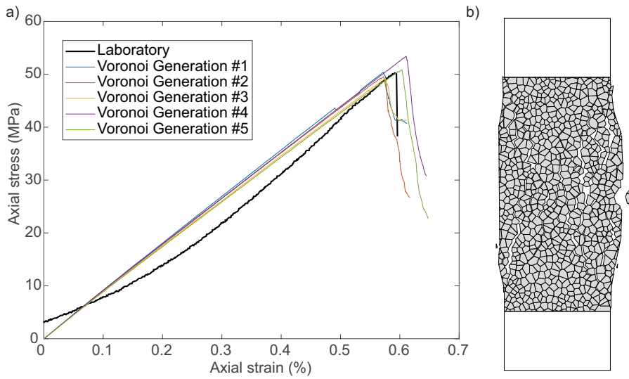
Fig. 7 a) Axial stress strain data from unconfined compression tests on five different Voronoi generations of UDEC GBM models calibrated to the properties of the Thornhill Rock, compared to a laboratory unconfined compression test on a specimen of Thornhill Rock. b) UDEC GBM model after an unconfined compression test showing the formation of conjugate shear planes and axial splitting.
