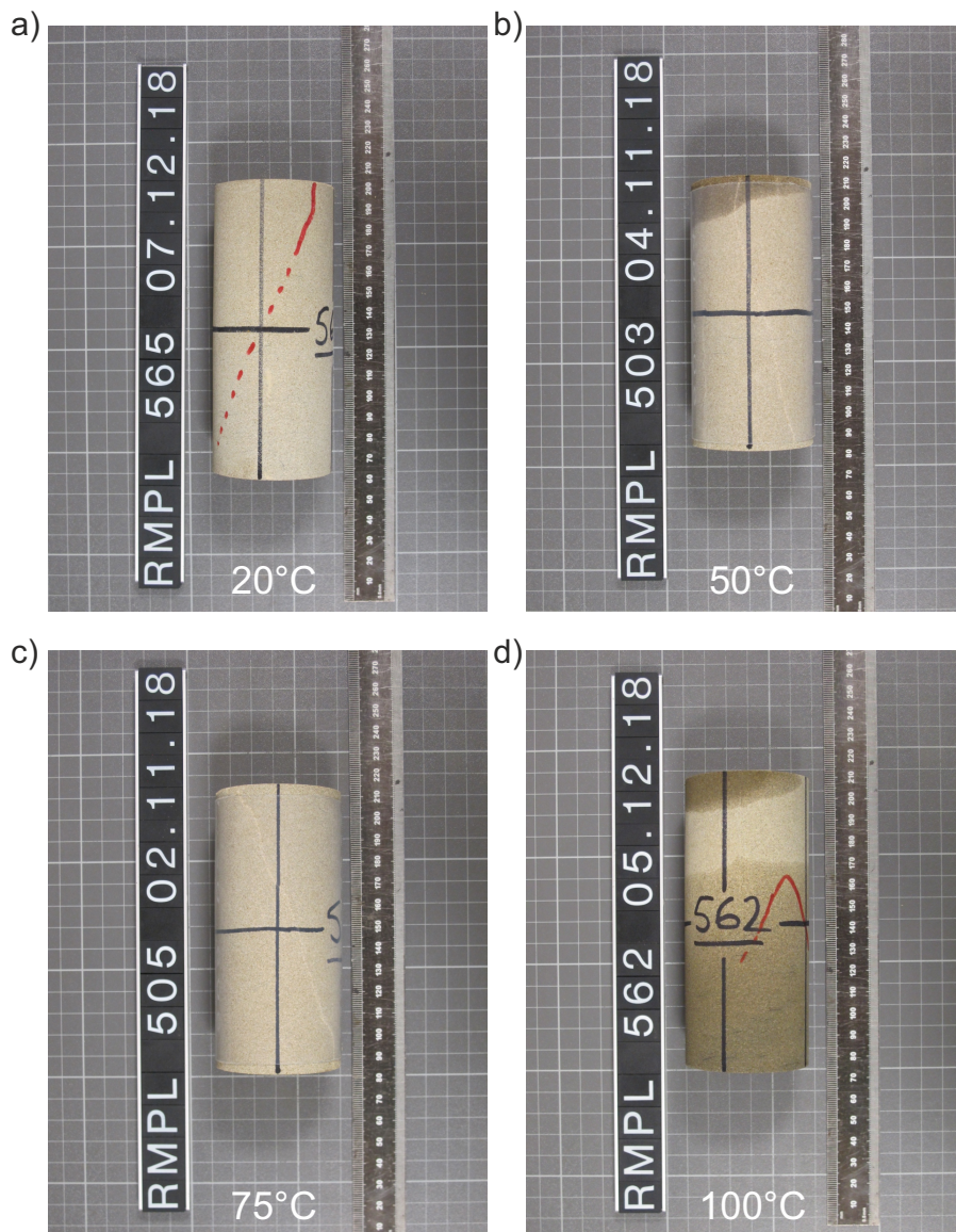
Fig. 4 Photographs of specimens of Thornhill Rock after thermo-mechanical triaxial testing, all tests were undertaken at 5 MPa \sigma_3 . Note slight oil ingress to specimens b) & d).
