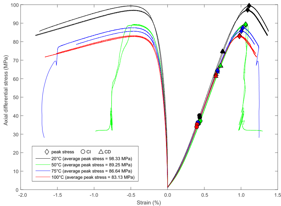
Fig. 3 Axial stress vs. radial and axial strain data for triaxial tests on specimens of Thornhill Rock, carried out at 5 MPa \sigma_3 and temperatures of 20 °C, 50 °C, 75 °C and 100 °C. (CI = crack initiation. CD = crack damage).
