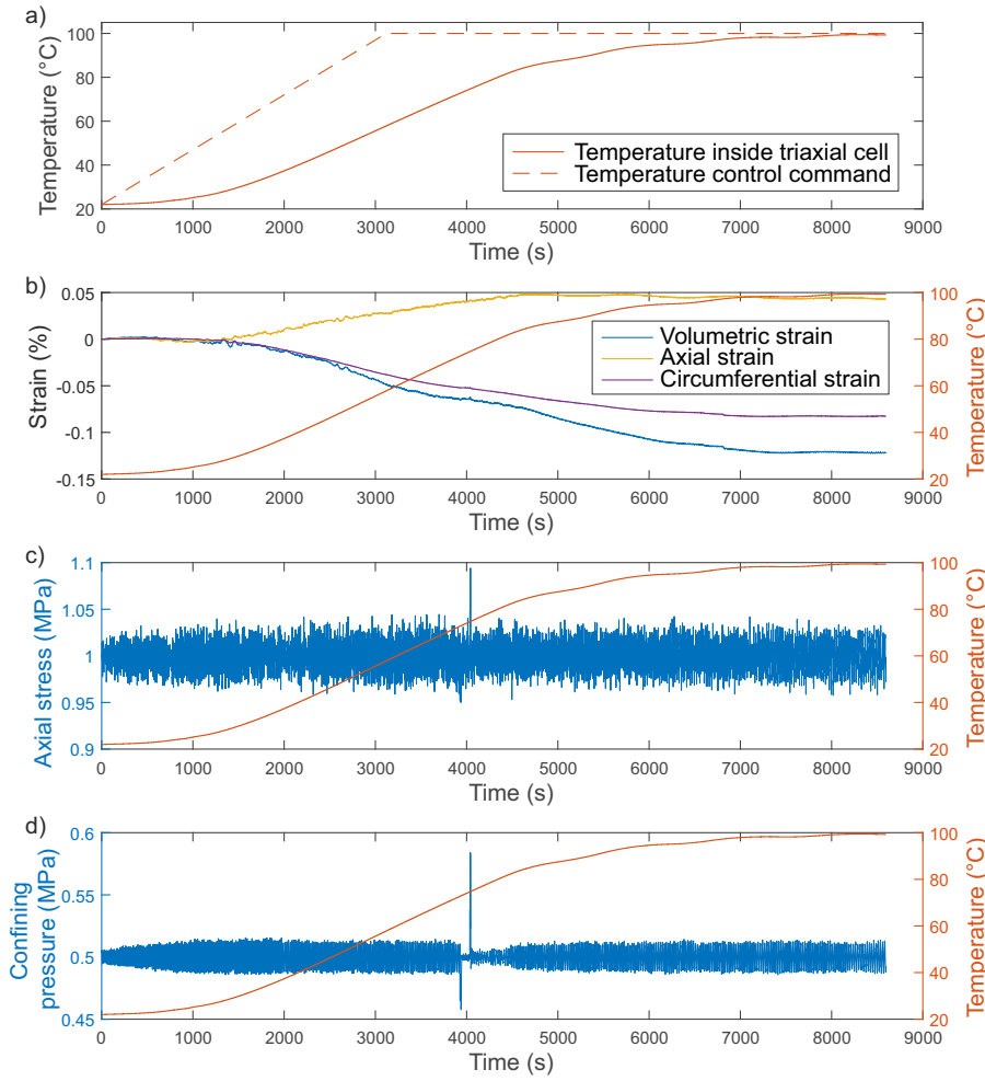
Fig. 2 a) Thermocouple data on the heating of Specimen # 562 within the triaxial pressure vessel, compared with the 1.5\text{ }^{\circ}\text{C min}^{-1} heating command. b) Volumetric, axial and circumferential deformation of the specimen during heating due to thermal expansion. c) Constant axial stress of 1 MPa maintained during thermal loading. d) Constant confining pressure of 0.5 MPa maintained during thermal loading.
