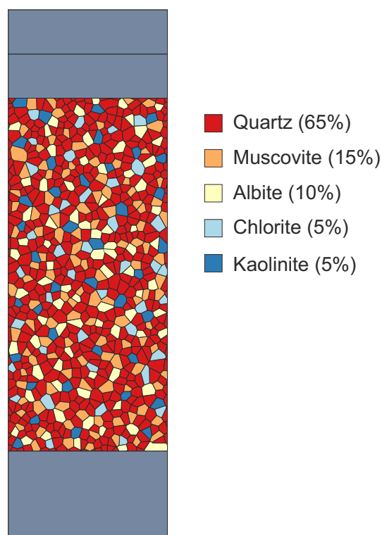
Fig. 8 UDEC GBM with thermal material properties applied to Voronoi blocks in mineral percentages for the Thornhill Rock.
