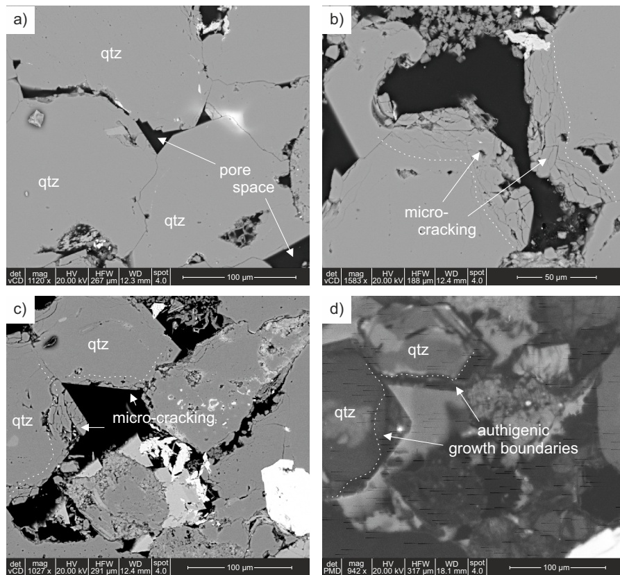
Fig. 13 a) BSE image of Specimen # 601 (oven dried at 40 °C). b) BSE image of Specimen # 602 (thermally loaded to 100 °C). c) BSE image of Specimen # 602 (thermally loaded to 100 °C). d) SEM-CL image of Specimen #602 (the same view as BSE image shown in c)).
