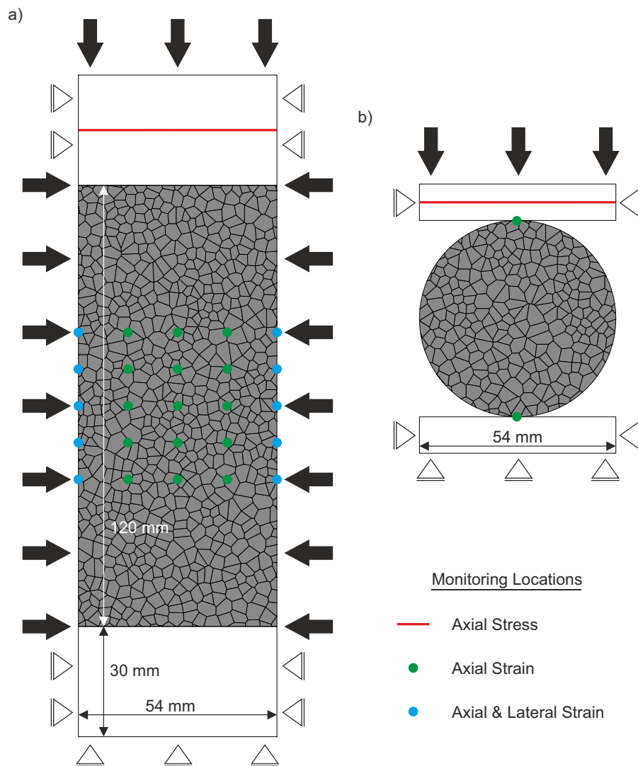
Fig. 6 Model dimensions, boundary conditions and monitoring locations for numerical simulations. a) Uniaxial and triaxial compression testing simulations. b) Indirect tension Brazilian disc testing simulations.
