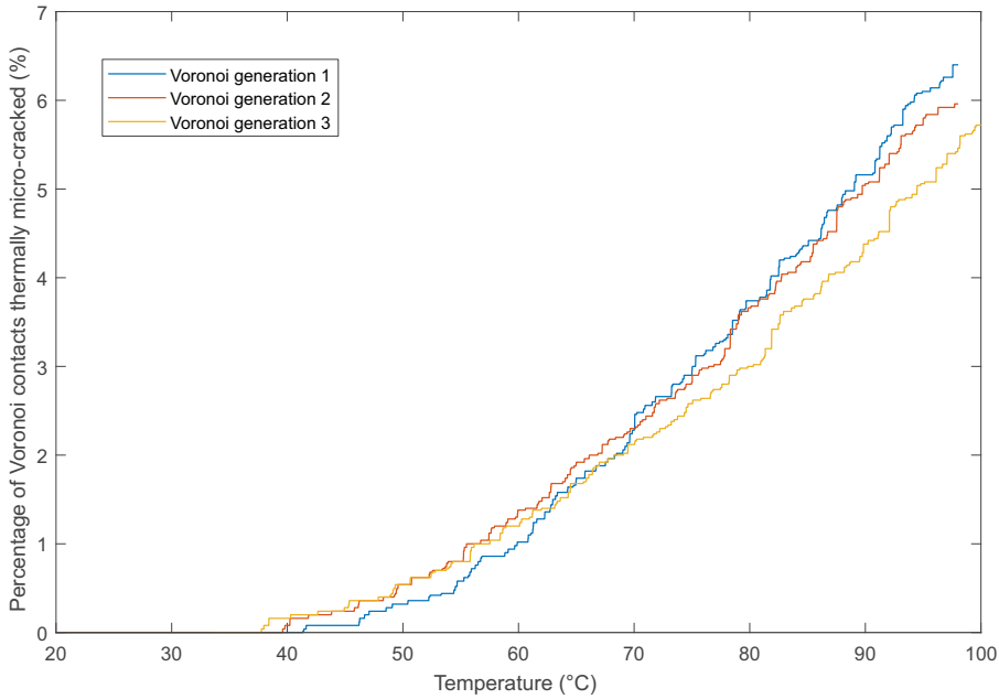
Fig. 11 Percentage of thermally micro-cracked Voronoi contacts with increasing thermal loading. Simulations were run with three different random Voronoi generations.
