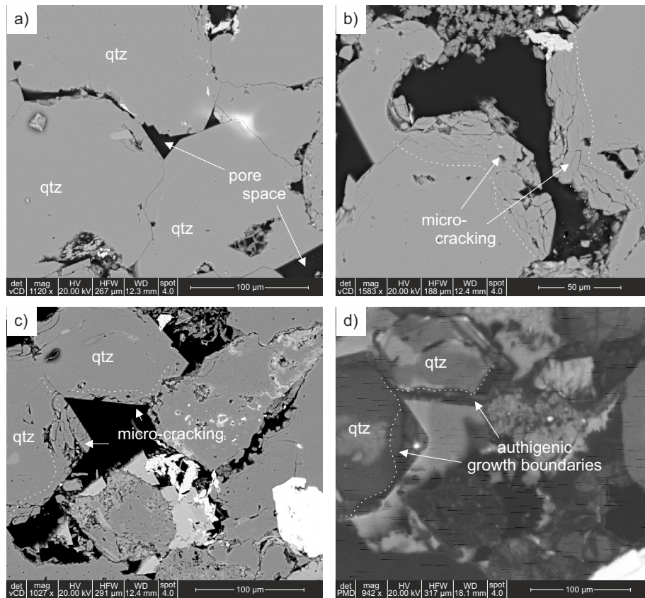
Figure 13: a) BSE image of Specimen # 601 (oven dried at 40 °C). b) BSE image of Specimen # 602 (thermally loaded to 100 °C). c) BSE image of Specimen # 602 (thermally loaded to 100 °C). d) SEM-CL image of Specimen #602 (the same view as BSE image shown in c)).
