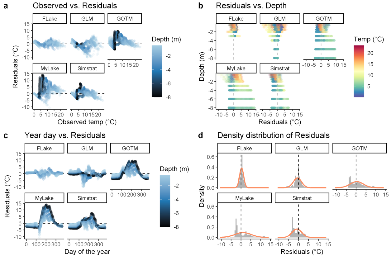
Figure B2. Water temperature residual diagnostic outputs from the calibrated ensemble run for Langtjern in the years 2014-2015 using hourly forcing data. a Observed water temperature vs. residuals; b residuals vs depth; c day of the year vs residuals and d distribution of the residuals.
