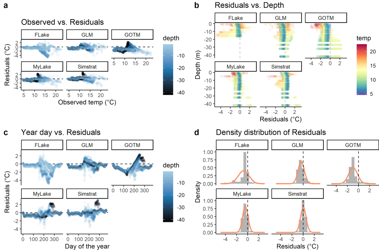
Figure 3. Water temperature residual diagnostic outputs from the calibrated ensemble run for Lough Feeagh in the year 2013 using daily forcing data. a Observed water temperature vs. residuals; b residuals vs depth, with the absolute simulated temperature in °C; c day of the year vs residuals and d distribution of the residuals.
