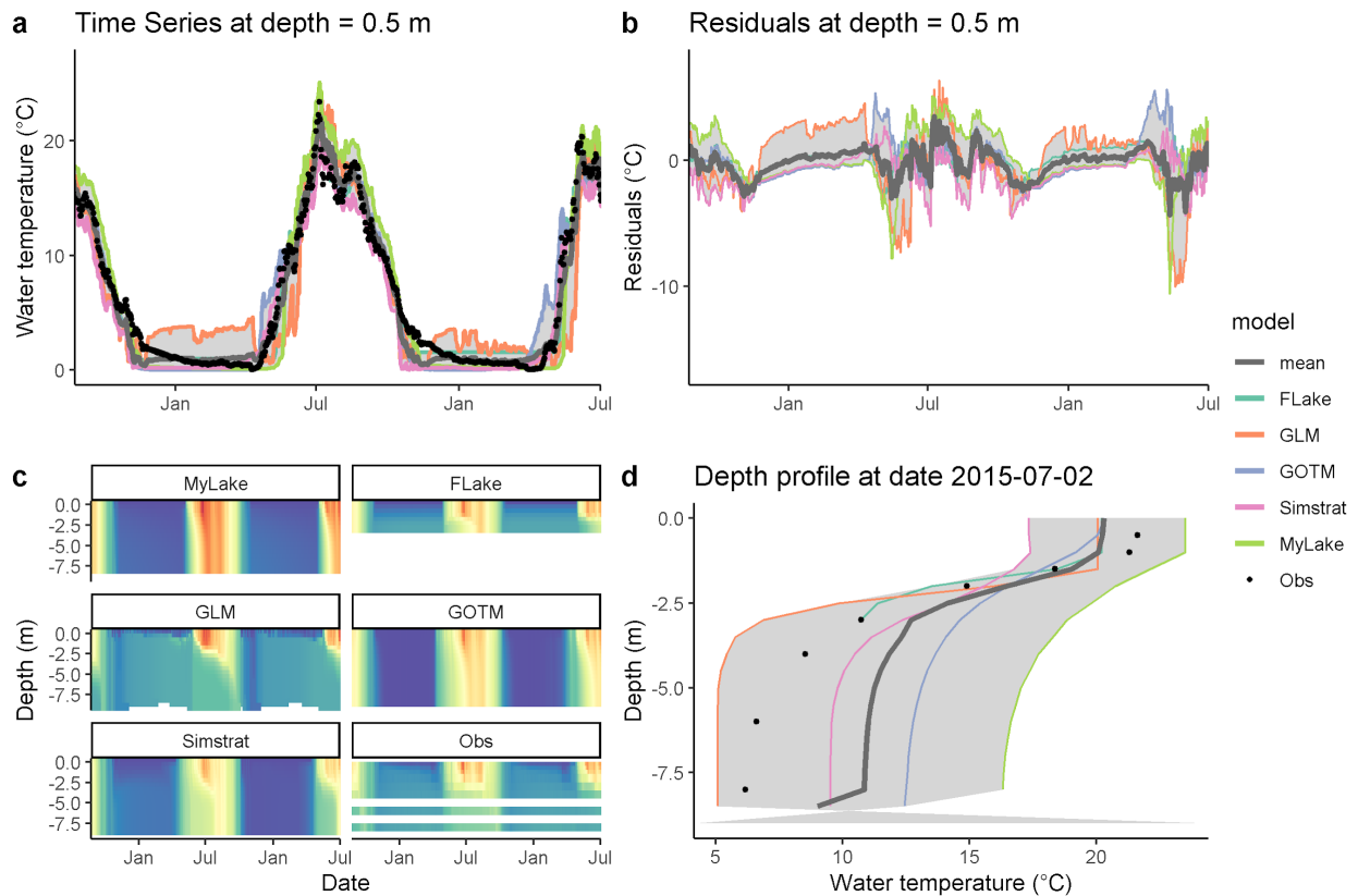
Figure B1. Calibrated ensemble output for simulated water temperature in 2014-2015 for Langtjern using hourly forcing data, showing: a time series of model output at 0.5 m depth for all
