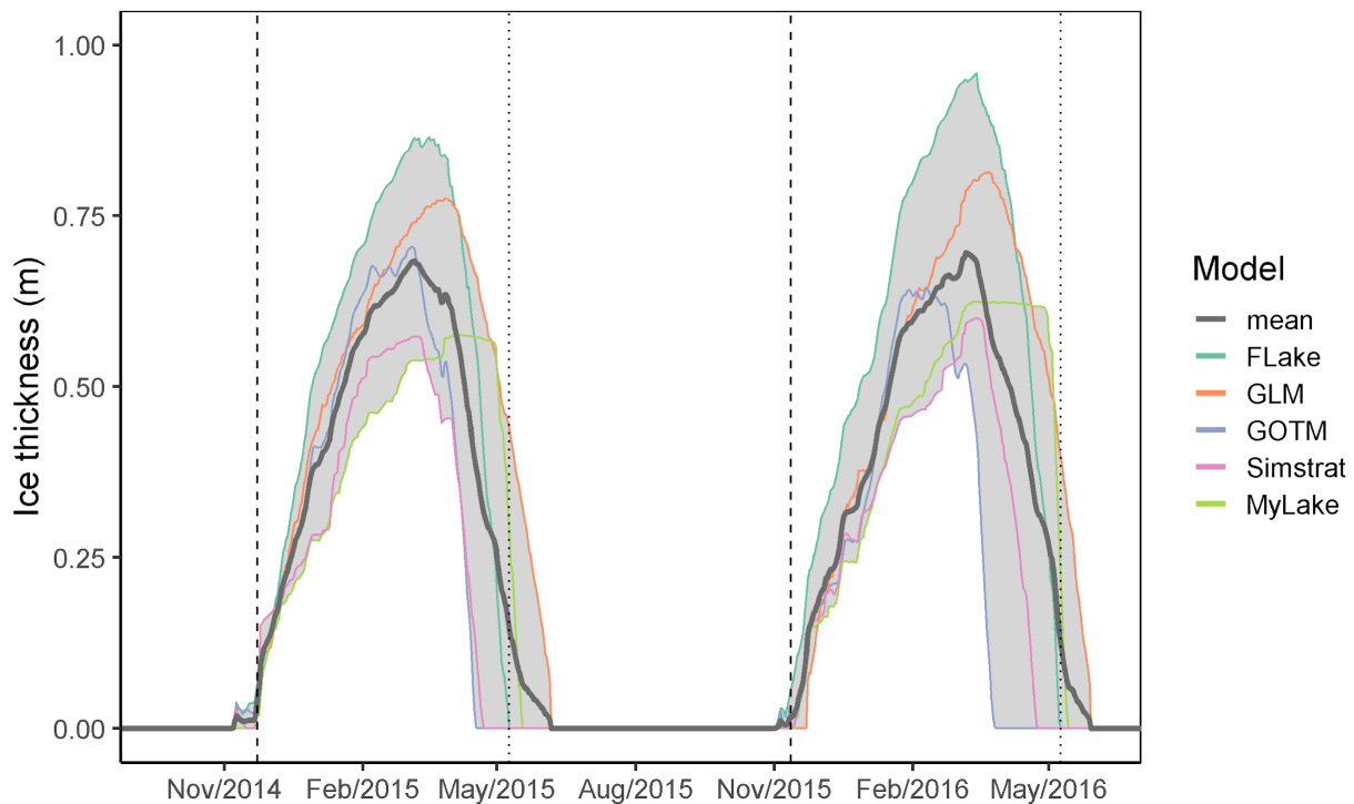
Figure 4. Calibrated ensemble model time series output for ice thickness for Langtjern, Norway. Dashed line indicates the observed onset of ice and dotted line indicates the observed offset of ice cover.
