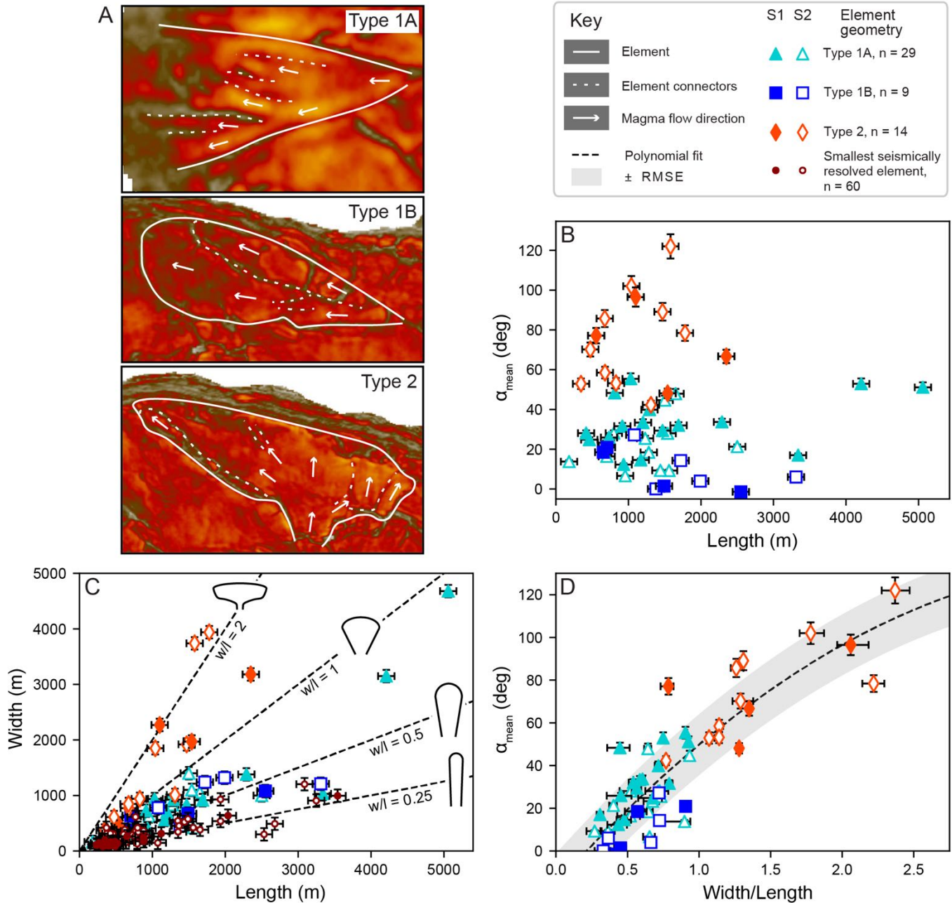
Figure 10: (A) Absolute-peak-amplitude maps showing different element geometries (i.e., Type 1A, 1B, 2). Dashed white lines highlight element connectors and white arrows indicate magma flow pathways. (B) Cross-plot of the maximum element length and the angle \alpha_{\text{mean}} (cf. Fig. 4B). (C) Cross-plot of the maximum element length and width. Black trend lines showing the ratio between the width and the length (i.e., w/l = 0.25 , w/l = 0.5 , w/l = 1 , w/l = 2 ), with aspect ratios < 1 indicating elongate geometries, and aspect ratios > 1 indicating wider geometries, highlighted by cartoons (solid black lines). (D) Cross-plot of width/length aspect ratios (C) and \alpha_{\text{mean}} angles.
