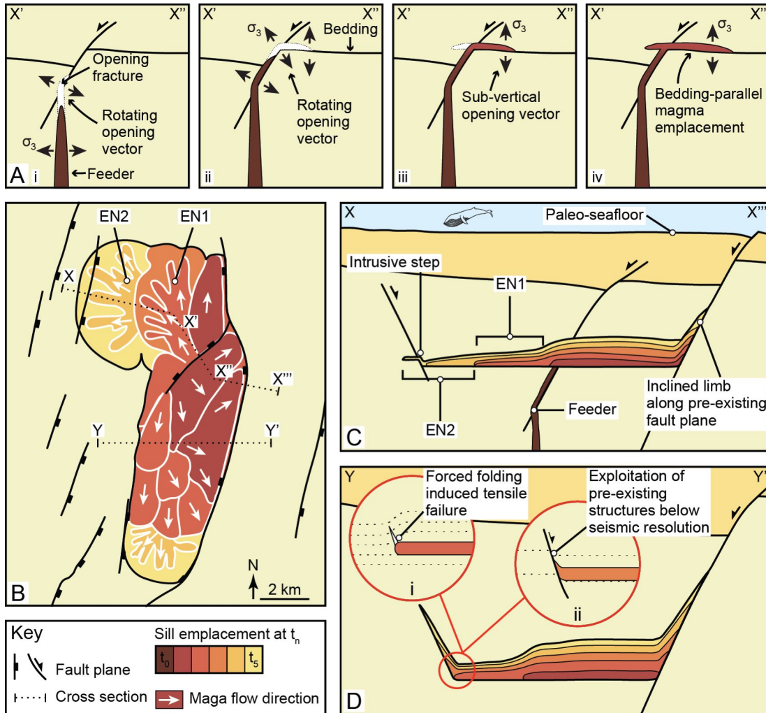
Figure 12: Schematic diagram showing how a potential feeding tube interacts with a pre-existing fault plane and subsequently transitions into a bedding-concordant sill. Localized rotation of the opening vector ( \sigma_3 ) to an orientation perpendicular to the fault plane (i) and the bedding (ii) may have caused the magma to propagate sub-horizontally, along a bedding plane. (B–D) Schematic diagrams showing the emplacement history of sill S2 in map view (B) and cross-section (C), (D), with different emplacement timesteps color-coded. It is to note that color-coded areas in (B) indicate the outer margin of propagating magma at given timesteps; i.e., even though younger magma pulses seem to be accreted to the edges of the intrusion, they also contributed to sill inflation as highlighted in cross section (C), (D). Cross section locations of (A), (C), and (D) are indicated in (B). Schematic cross-sections are not to scale. Please refer to ‘Sill Emplacement History and Magma Flow Pathways’ for a detailed discussion.
