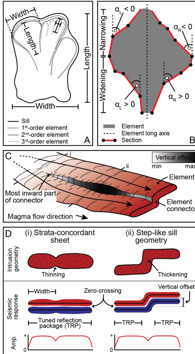
Figure 4: (A) Schematic diagram of a sill indicating comprising elements and according width and length measurements. (B) Schematic diagram of an element and measured angles \alpha . The element outline is partitioned into small sections to quantify how \alpha varies in long-axis direction. Angles are measured between the section and the element long-axis at the node of each section. The sum of angles measured for the left-hand side ( \alpha_L ) and right-hand side ( \alpha_R ) at the same location on the element long axis equals the total angle \alpha . A positive angle \alpha represents an element widening (i.e., increase in width), whereas a negative angle \alpha represents an element narrowing (i.e., decrease in width). (C) Schematic diagram showing two vertically offset elements that are connected via an
