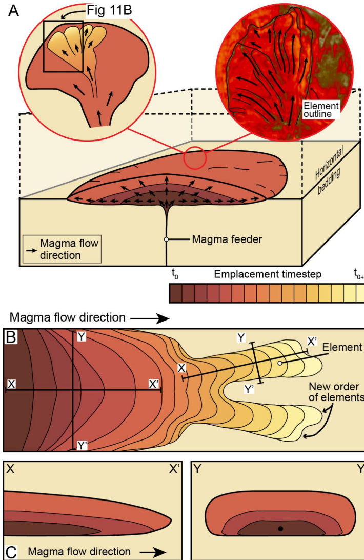
Figure 11: Conceptual flow and inflation model of (A) a sill and (B) elements in 3D view and map view, respectively ((A) modified after Ferré et al., 2002). Zoom in (A) shows an element network and containing elements at the propagating sill tip in map view. (B) Magma propagation of an element that breaks down into elongate elements over time. Note that a new order of elements is starting to emerge at the element tips. Contours are based on a numerical study on viscous fingering (modified from Ebrahimi et al., 2016). (C) Cross-section through a feeding tube and emerging elongate elements, parallel (X-X') and perpendicular (Y-Y') to the element long axis. Schematic diagrams are not to scale.
