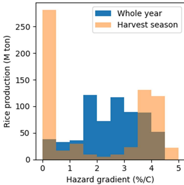
Figure 6: Histograms showing the distribution of hazard gradient across harvest seasons and locations. The effect of seasonal weighting assumptions on the hazard gradient is shown: the blue histogram represents the assumption that the whole year is equally weighted, while the orange histogram shows the result if only the rice harvest season is included. The histograms are weighted by the harvest weight in millions of tonnes.
