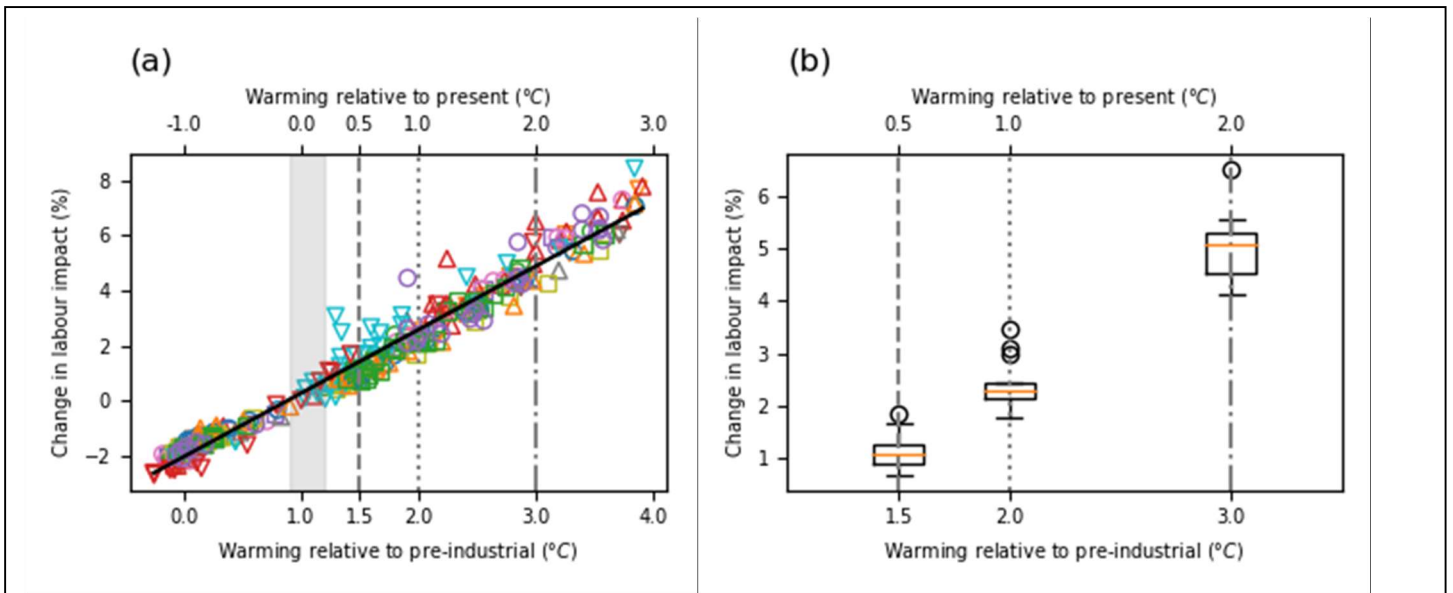
Figure 5: Relationship between rice labour impact and GSAT change in the 14 analysed CMIP6 climate models; Changes are relative to 1.0 C of warming relative to 1850-1900, which is assumed to represent the present. Three levels of warming relative to 1850-1900 and relative to the present are shown for context. The present estimated range of warming is shown by the grey shading. (a) Change in labour impacts against GSAT for 20 year periods; each shape/colour corresponds to a different model The black trend line is illustrative only: fit statistics mentioned in the text are based on fitting each climate model individually. (b) Change in labour impacts at three levels of warming, with box plot to show climate model spread. Points are linearly interpolated to the three levels of warming. Boxes show 1st (Q1) and 3rd quartile (Q3); orange line at the median; lower whiskers at lowest point above Q1 - 1.5 * (Q3 - Q1) , upper whiskers highest point below Q1 + 1.5 * (Q3 - Q1) ; circles are points outside the whisker range. We define hazard gradient as the gradient between GSAT and local labour impact.
