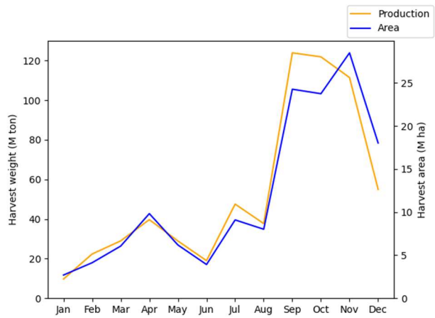
Figure 2: Rice harvest weight and area in Asia, plotted against month. Data from RiceAtlas.
