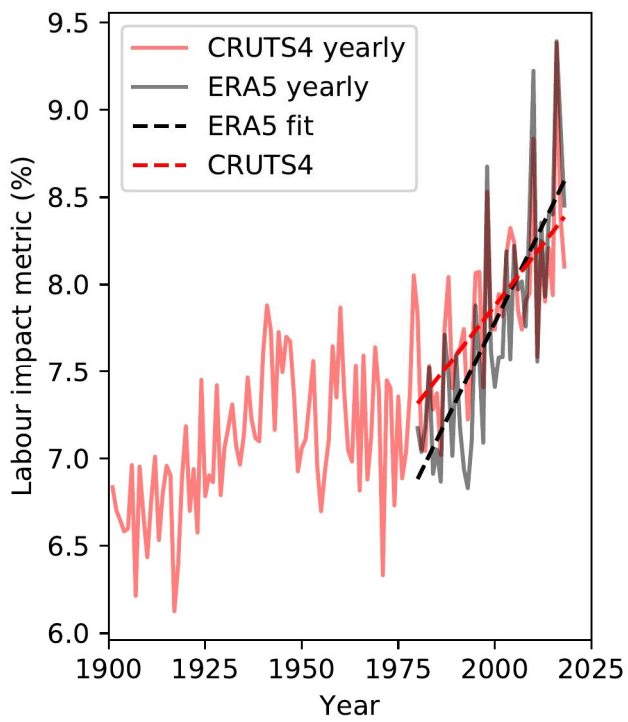
Figure 4: Annual Asia-wide mean labour impact, weighted by total rice production, calculated from CRU-TS 4.03 (red lines) and ERA5 (black line), with trend lines (dashed) shown for the period 1980-2018.
