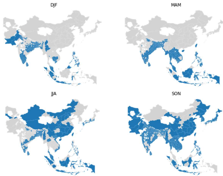
Figure 3: Locations of a rice harvests by season. Areas with a rice harvest in a given season are shown in blue. Data from RiceAtlas.
