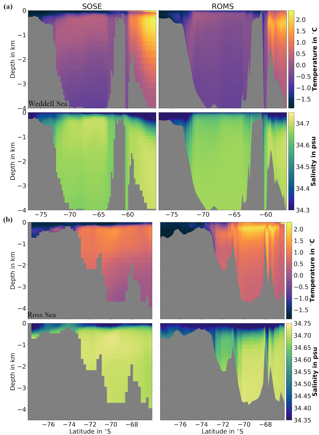
Figure 7. Temperature-Salinity distribution in (a) the Weddell Sea along 45°W, (b) Ross Sea along 180°W, (c) Bellingshausen Sea along 75°W and (d) Prydz Bay along 70°E. Transect locations are shown in Figure 1.
