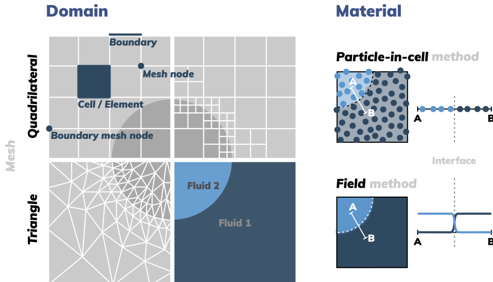
Figure 4. Examples of two-dimensional domain discretisation. The domain discretisation on the left illustrates different types of meshes. The top half mesh is build on a quadtrees with several levels of mesh refinement (top right) so as to better capture the interface of the circle. The bottom left quarter is based on an unstructured triangular mesh built so that element edges are aligned with the (quarter) circle perimeter. The material discretisation on the right illustrates different methods of material tracking based on the particle-in-cell method (top) and grid-based advection (bottom) for the material contrasts shown in the bottom right right quarter of the material discretisation.
