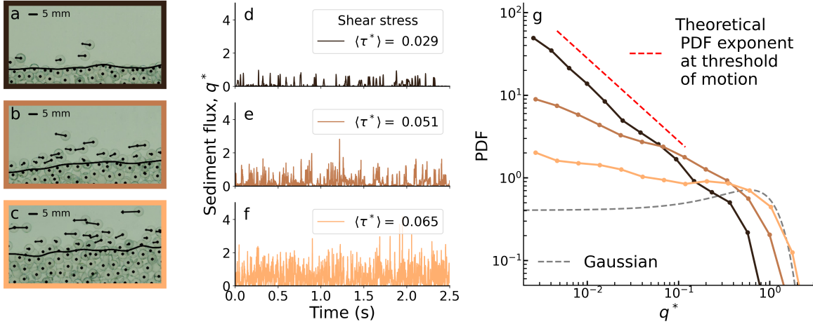
Figure 2. Intermittent bed load sediment flux. Sample data from three flume experiments using glass spheres, representing typical runs with low sediment flux (a and d), intermediate sediment flux (b and e), and high sediment flux (c and f). a-c, High-speed video frames showing grain centers and velocities and the location of the bed, as in Figure 1b. d-f, Samples of the corresponding sediment flux time series. g, Probability density function (PDF) calculated from the sediment flux time-series. The red dashed line shows the theoretical exponent of the PDF tail, -1 , at the threshold of motion. The grey dashed line shows a Gaussian distribution with the same mean and variance as the high sediment flux case.
