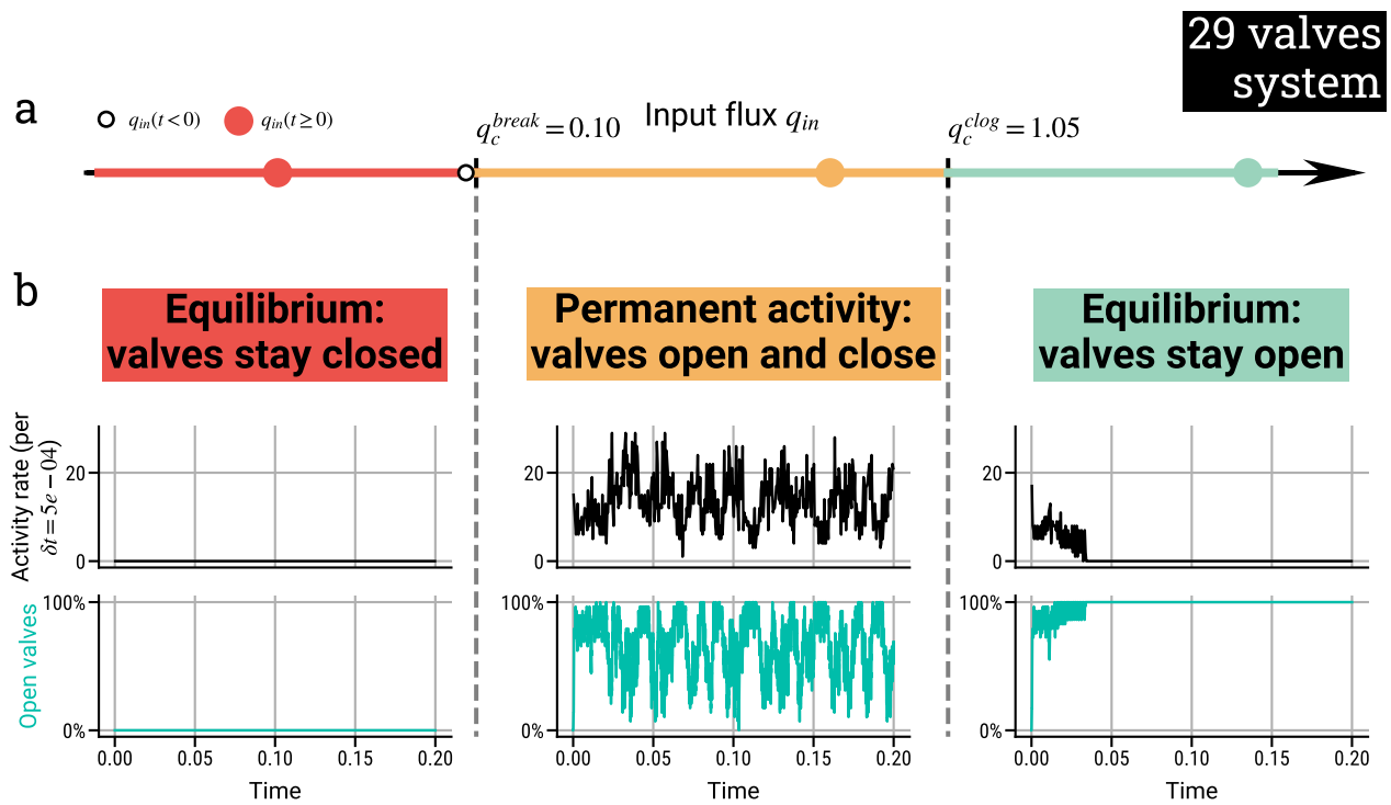
Figure 9: Influence of the input flux q_{in} in a representative system with 29, randomly distributed valves. (a) Three intervals of input flux q_{in} are delimited by two threshold values q_c^{clog} and q_c^{break} . (b) Examples of activity rate (number of events per \delta t = 5 \times 10^{-4} , scaled unit, in black) and proportion of open valves (in cyan) as a function of time, starting at t = 0 with all valves closed. Valve distribution represented in Figure 2, valve parameters are listed in Table 2.
