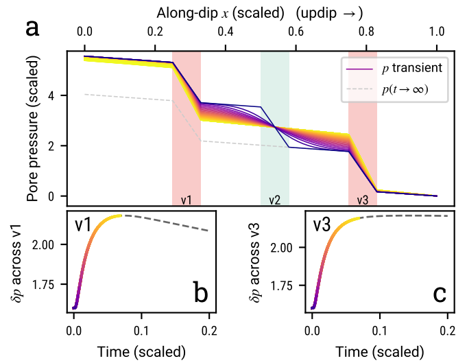
Figure 6: Interactions between three neighboring valves. (a) Transient evolution of pore pressure from an initial equilibrium profile with all valves closed towards a profile with valves v1 and v3 closed and valve v2 open. Panels (b) and (c): pore pressure difference evolution across valves v1 and v3 .
