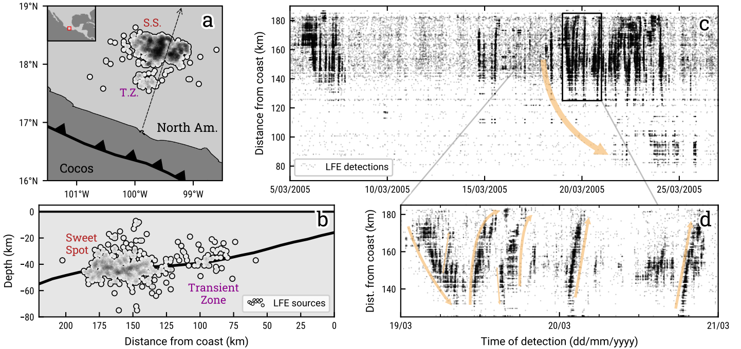
Figure 1: The Guerrero (Mexico) tremor zone in (a) map view and (b) vertical cross-section. Each dot represents a low-frequency earthquake family from Frank et al. [2014]. Thick black lines outline the trench and the subduction interface (data from Hayes [2018]). (c) and (d), LFE activity in a time-location chart from the Frank et al. [2014] catalog. Activity occurs in two patches centered on the subduction interface, a dense downdip one called the sweet spot and a sparser updip one called the transient zone . Tremor activity migrates along the subduction interface in both the updip and downdip directions, as shown by the orange arrows.
