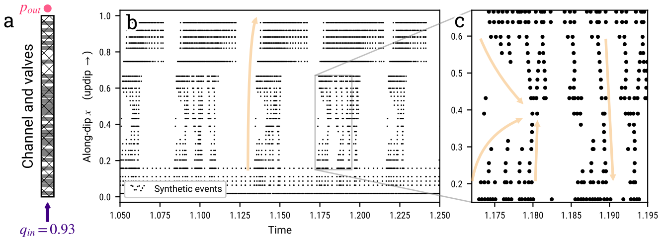
Figure 11: Synthetic tremor activity patterns. (a) Distribution of valves in the permeable channel. This distribution was generated randomly and contains three large clusters. (b) Activity patterns in space and time. Black dots stand for valve opening events. The lower valve cluster ( x = 0 - 0.18 ) is active almost continuously. The middle and upper clusters ( x = 0.2 - 0.65 and x = 0.7 - 1 ) is activated sequentially in bursts. Within a burst, activity is intermittent too. (c) focus on the activity in the middle valve cluster showing fast, short-scale migrations in both the updip and downdip directions. Valve distribution represented in Figure 2, valve parameters are listed in Table 2.
