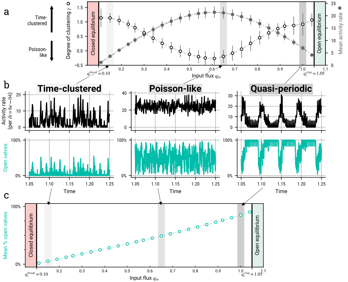
Figure 10: Different permanent activity styles as a function of the input fluid flux, averaged for 30 different 29-valve systems. (a) In white, the level of time clustering \gamma : the spectral slope of autocorrelation of event counts (see text) ; in gray, mean activity rate: number of events per unit time, both as a function of input flux q_{in} . For \gamma close to 0, activity is Poisson-like with no time clustering. The higher \gamma is, the more clustered and episodic activity is. (b) Activity rate (in black) and proportion of open valves (in cyan) as a function of time for particular simulations within the different regimes. (c) Time-averaged proportion of open valves in simulations, as a function of input flux. In (a) and (c), each dot represent the average value of the variable over 30 different 29-valve systems, at the given flux. Error bars are present in both panels, representing the standard deviation of this measurement over the 30 systems.
