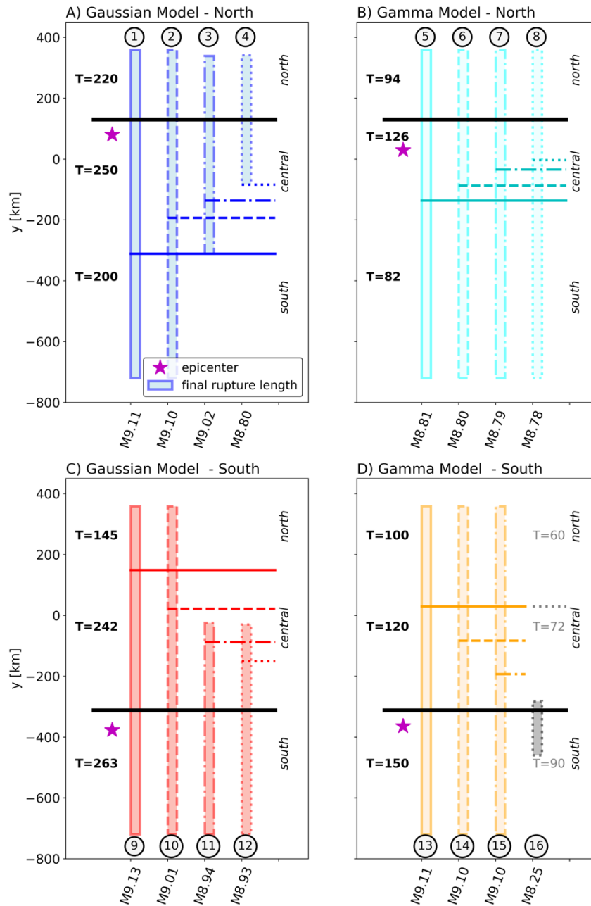
Figure 5. Gaussian and Gamma dynamic rupture simulations nucleated in northern or southern Cascadia (magenta star). In each plot, the colored rectangle corresponds to the along-strike rupture extent. The solid or dashed lines correspond to the segment location, of which one is allowed to vary. A) Gaussian ruptures where the width of the middle segment, containing the nucleation asperity, is varied until margin-wide rupture no longer occurs. The T levels (relative dynamic stress drop) remains constant for each simulation. B) Same idea as A but for Gamma rupture simulations. Moment-magnitude is plotted along the x-axis on all plots. C) and D) show Gaussian and Gamma ruptures nucleated in southern Cascadia, respectively. For each subfigure, the numbers refer to the model number, which are listed in Table 1.
