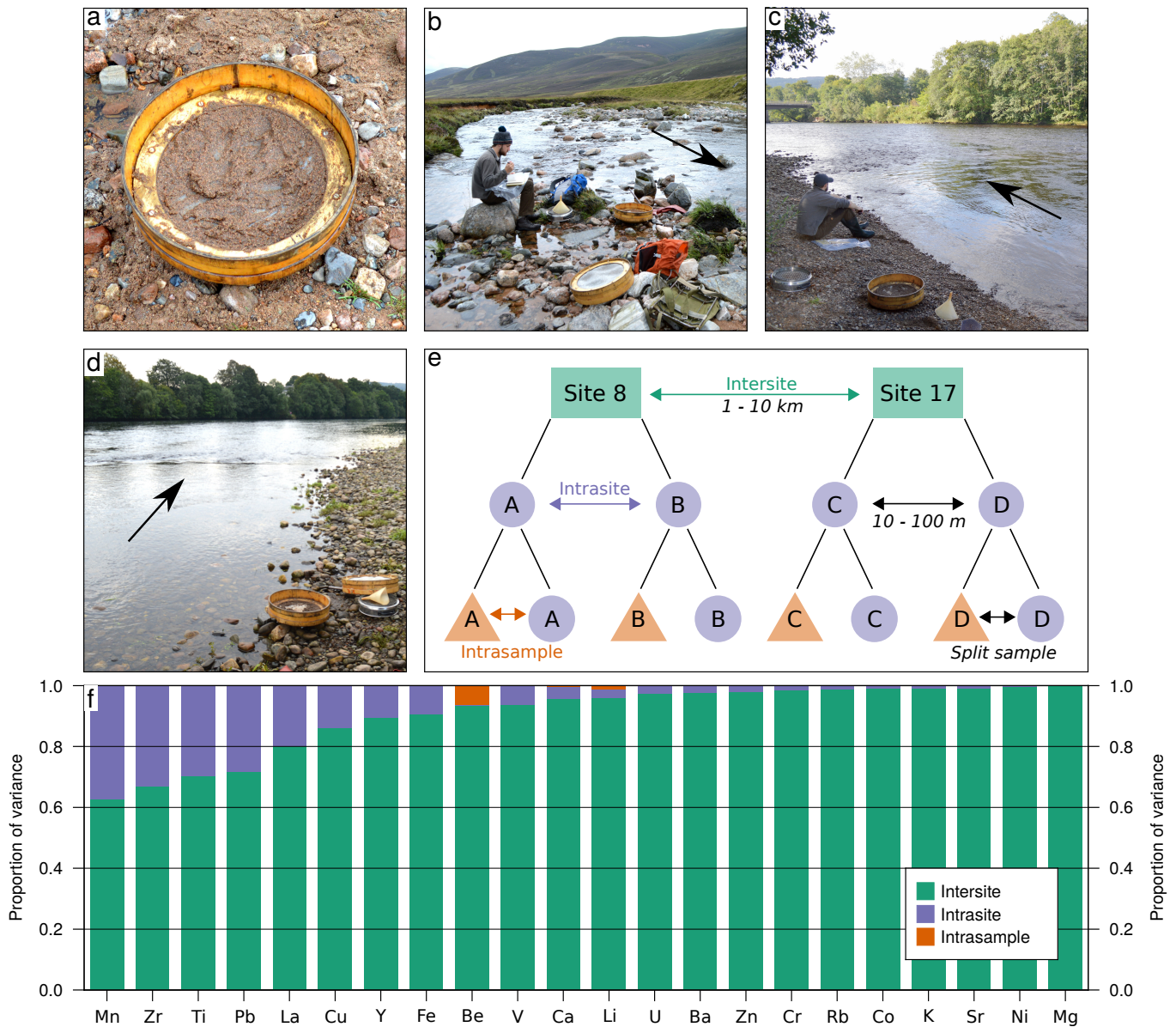
Figure 3. Sampling methodology and analysis of variance (ANOVA). (a) Nested sieve set used for sampling. Photograph shows sediment on top of 150 \mu\text{m} mesh atop collecting pan; apparatus has a 45 cm diameter. (b) Photograph shows Locality 29 (upper reaches of River Dee); arrow indicates flow direction. (c) Locality 48, River Tummel, a tributary of Tay. (d) Locality 55, close to mouth of River Tay at Perth. (e) Schematic of nested sampling procedure. Coloured text under Site 8 indicates the hierarchy of variance (see panel f). Black text under Site 17 indicates how sample hierarchy was created. (f) Results of nested ANOVA indicates that most variance lies between sites for all studied elements, thus large scale geochemical signals dominate over local heterogeneity. Intrasample variance is negligible in most cases.
