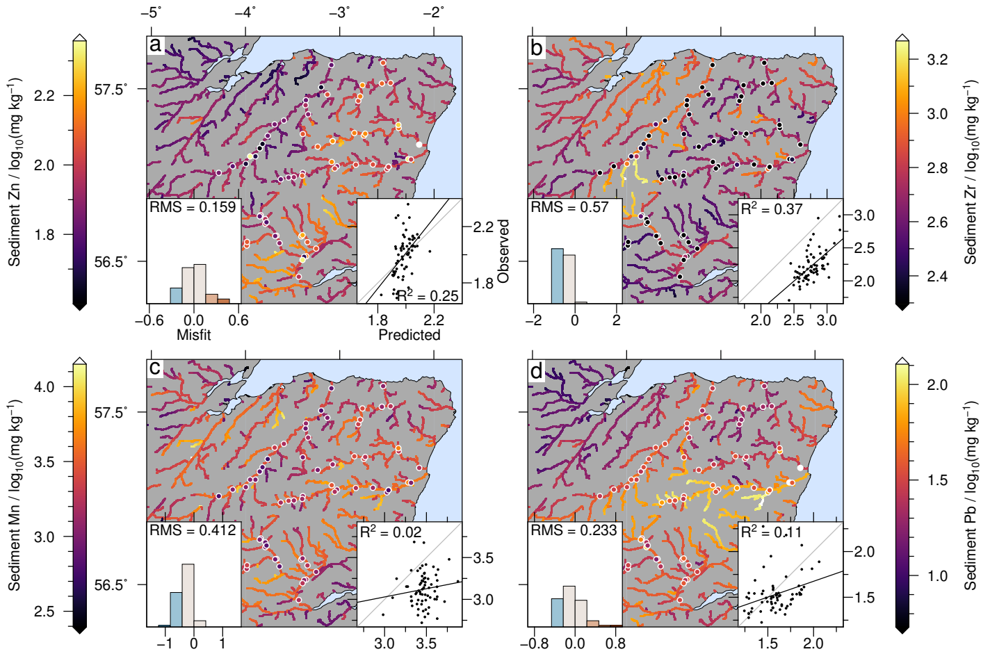
Figure 6. Comparison of observations and less accurate predictions. (a) Observed Zinc concentrations (coloured circles) overlain on predictions (coloured curves). Note logarithmic colour scale. Right inset shows cross plot of observations and predictions; grey line is 1:1 relationship; black line is linear fit to points; annotation shows R^2 value. Left inset shows histogram of misfit between observations and predictions; bin width is equal to RMS misfit; blue/red indicate over-/under-prediction. (b) Zirconium. (c) Manganese. (d) Lead. Results for elements with more accurately predicted concentrations are shown in Figure 5. Results for all other elements are shown in Figure 4 and Supporting Information (Figures S1, S2).
