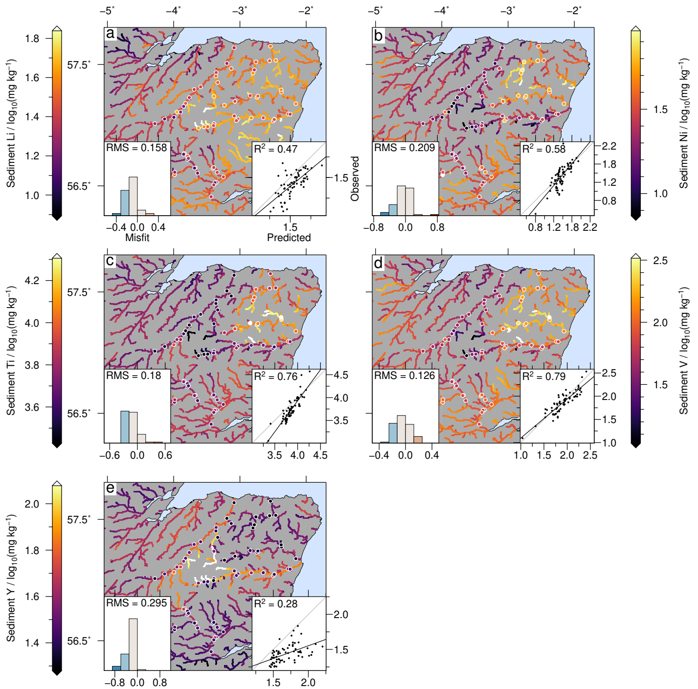
Figure S2. Results for other elements modelled by our approach. This figure is interpreted in the same way as Figures 5 and 6 in the main document
