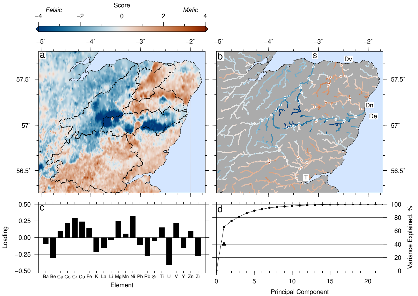
Figure 8. Principal Component Analysis (PCA) of geochemical data. PCA is applied to the higher-order river samples following centred log-ratio transformation and the loadings of the principal components were extracted. Observed compositions from the G-BASE data set and model predictions were projected onto these loadings. (a) G-BASE stream sediment data projected onto first principal component and interpolated using minimum curvature spline with tension factor of 0.25. Note the strong relationship to bedrock geology (Figure 1b). (b) Observed and predicted fluvial sediment composition projected onto first principal component. The Spey and Dee carry a more felsic signature whereas the Deveron and Don are more mafic. Rivers labelled: S = Spey, Dv = Deveron, Dn = Don, De = Dee, T = Tay. (c) Loadings on PC1 indicate the geological processes underlying the principal component. Elements with positive loadings are typically associated with mafic igneous rocks whereas negative loadings are associated with felsic rocks. (d) Variance contained on each principal component. Arrow indicates first principal component (displayed here; PC1), which contains 68% (i.e., the majority) of the total variance within the observed geochemical dataset.
