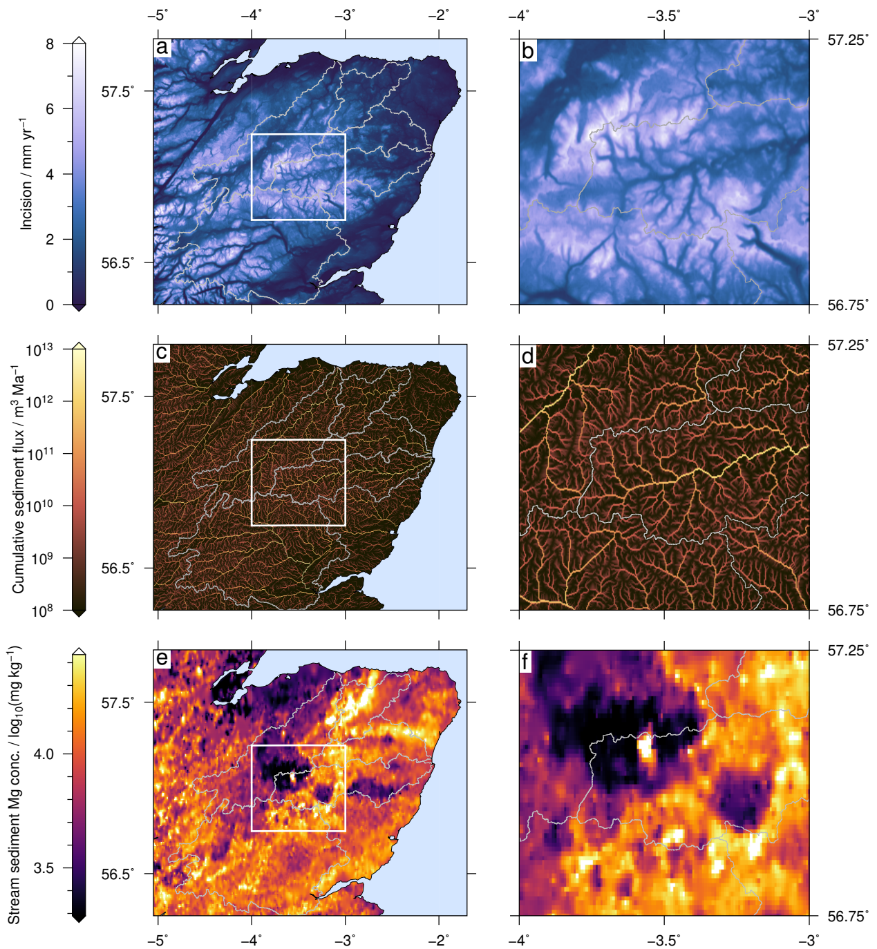
Figure 2. Inputs used in geochemical predictions. (a) Predicted incision, calculated using SRTM data set (Figure 1a) and Equation 3 with n = 1 , m = 0.35 , v = 3.62 \text{ m}^{0.3} \text{ Ma}^{-1} . (b) White box = panel (b), which shows upper portion of Dee catchment. Grey lines indicate catchment boundaries. (c-d) Predicted cumulative sediment flux calculated by integrating incision (panel a) along flow paths. (e-f) Mg composition of first order stream sediments interpolated from G-BASE localities using a continuous curvature spline with a tension factor of 0.25 (Figure 1c). Analogous maps were generated for all elements.
