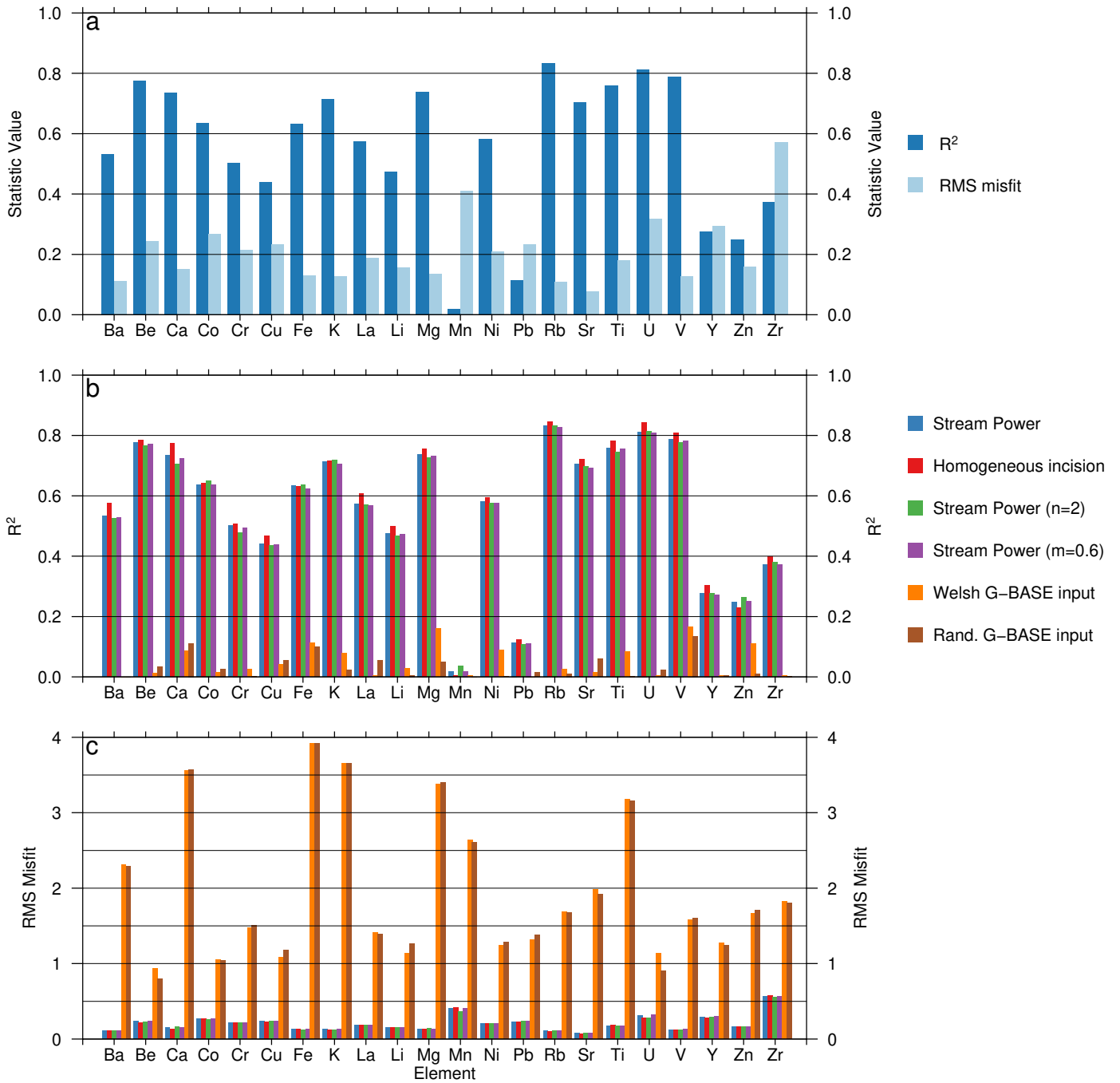
Figure 7. Evaluation of model predictions. (a) R^2 and RMS misfit between observed and predicted element concentrations for preferred Stream Power erosional model. (b) R^2 for different models and parameterisations; see key and Supporting Information for visualisation of substrate generated using Welsh G-BASE measurements and a random distribution (Figure S3). (c) RMS misfit for different models/parameterisations.
