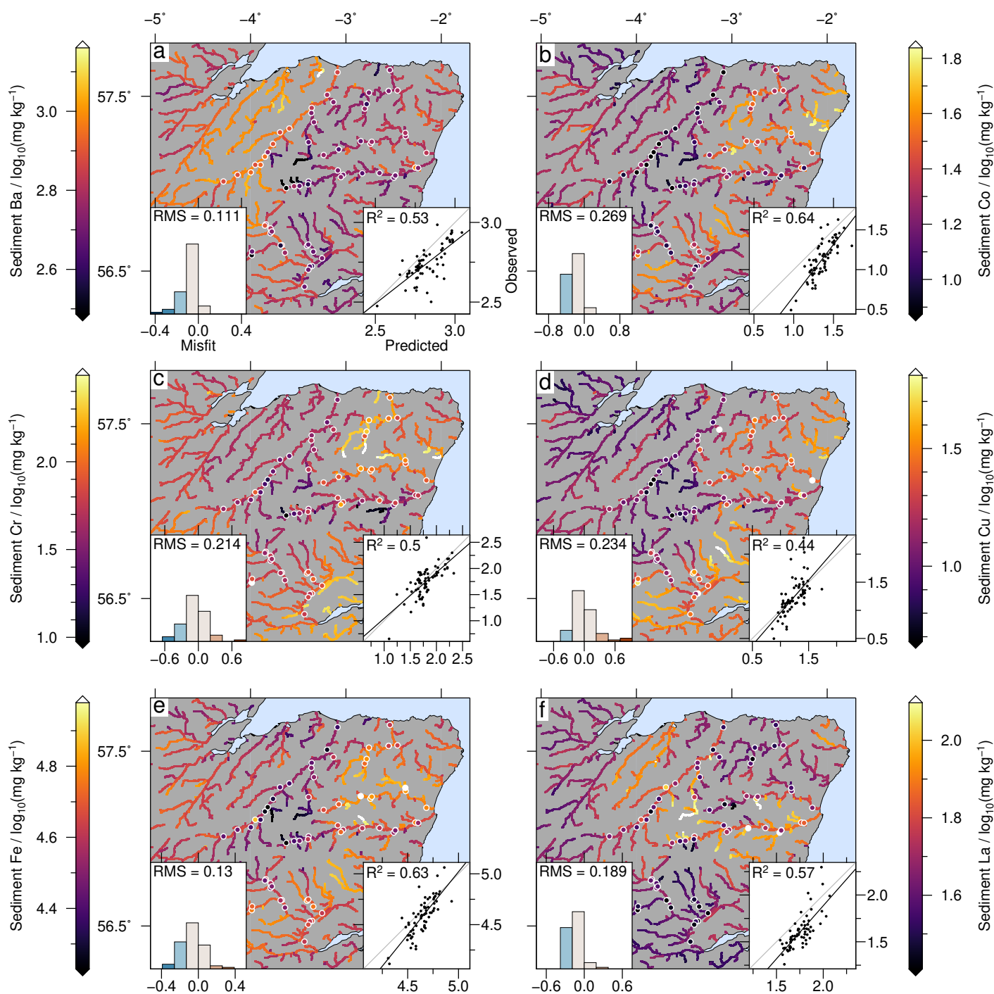
Figure S1. Results for other elements modelled by our approach. This figure is interpreted in the same way as Figures 5 and 6 in the main document
