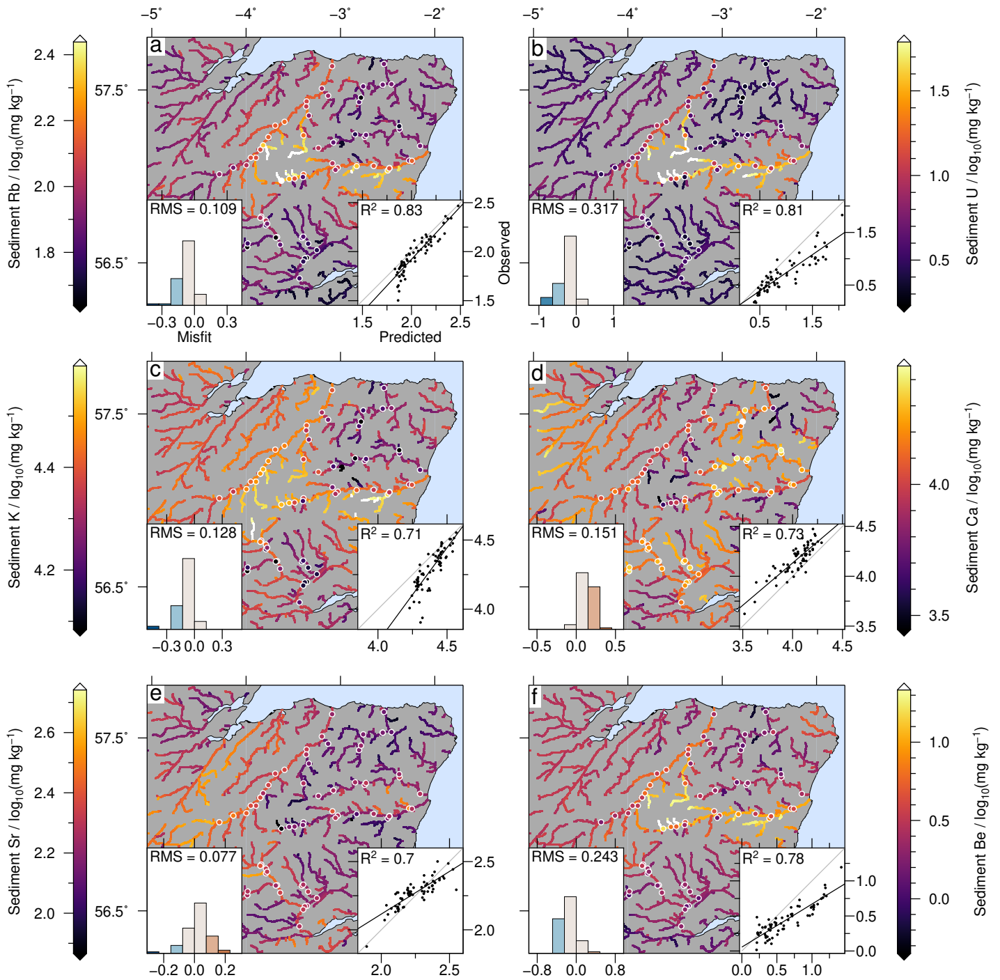
Figure 5. Comparison of observations and most accurate predictions. (a) Observed Rubidium concentrations (coloured circles) overlain on model predictions (coloured curves). Note logarithmic colour scale. Right inset shows cross plot of observations and predictions; grey line is 1:1 relationship; black line is linear fit to points; annotation shows R^2 value. Left inset is histogram of misfits; bin width is equal to RMS misfit; blue/red indicate over-/under-prediction. (b) Uranium. (c) Potassium. (d) Calcium. (e) Strontium. (f) Beryllium. Results for elements with less accurate predictions are shown in Figure 6. Results for all other elements are shown in Figure 4 and Supporting Information (Figures S1, S2).
