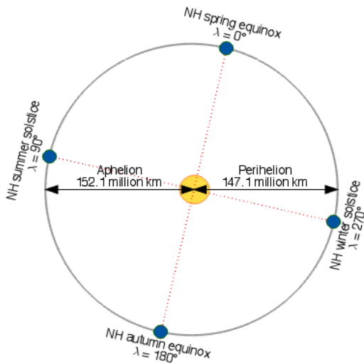
Figure 2. Graphical representation of the Earth's orbital configuration in the early 21 st century (eccentricity: 0.0167, geocentric longitude of perihelion: 283°). The orbital shape has been drawn to scale. The size of the Earth and Sun have been increased for visual clarity.
