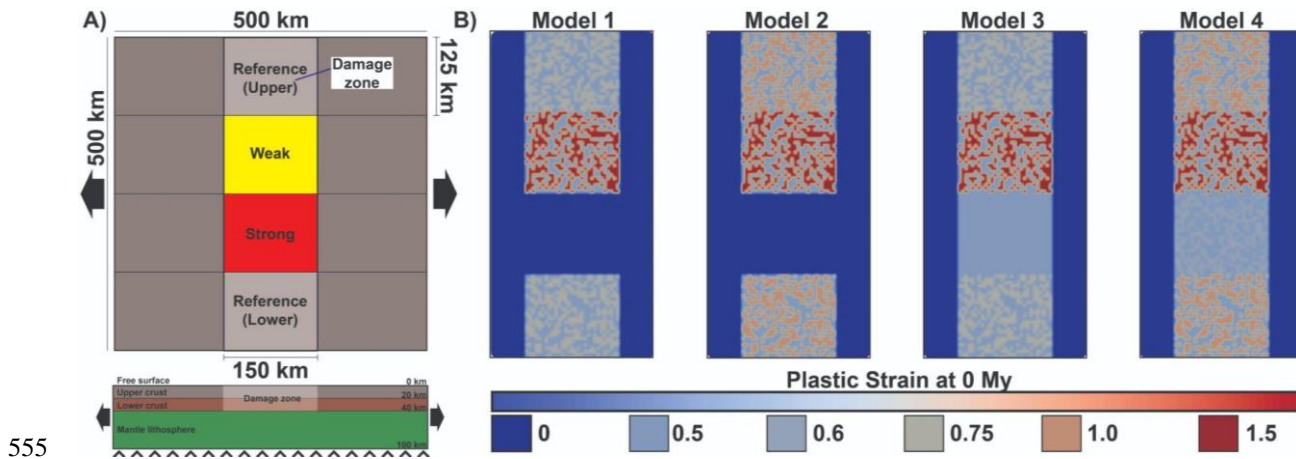
Figure 2: A) Diagram showing the map view and cross-sectional setups for the model. Strain is applied across a 500 km wide and 100 km deep area, with a 150 km wide ‘Damage Zone’ extending to 40 km depth across the centre of the model where IPS is assigned to unit blocks. B) Images of the IPS distribution applied to each model prior to extension at 0 My. Variations in IPS values between 5 km 3 Unit blocks define various strength terranes.
