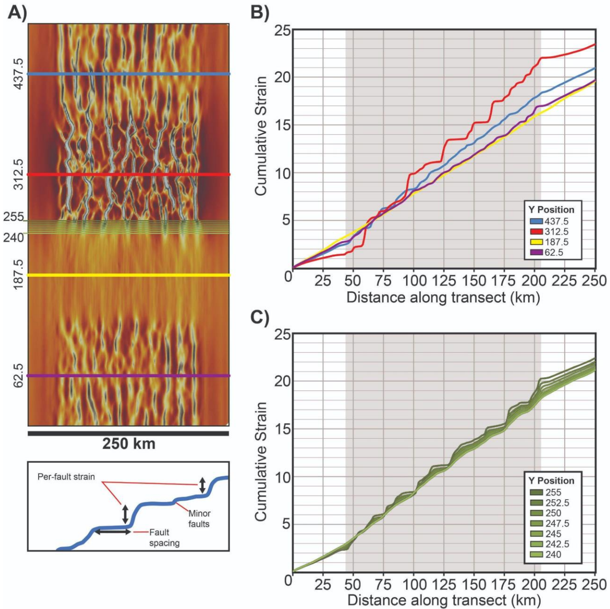
570 Figure 5: A) Map-view image of non-initial plastic strain at 10 My across the central 250 km of the model. B) Strain analysis of 575 multiple transects across the centre of each domain of the model, see A for location. The grey shaded area represents the location of the damage zone initially across the central 150 km of the model. Note how fault spacing and per-fault strain are greatest in the Weak domain whilst the Strong domain approximates uniform strain. C) Strain analysis of a series of model transects spanning the boundary between the Strong and Weak domains. Fault spacing and per-fault strain decrease across the boundary into the Strong domain.
