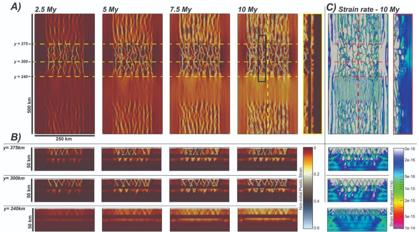
565 Figure 4: A) Left - Map view images highlighting the fault evolution across the model using the Non-initial plastic strain attribute at 2.5 My, 5 My, 7.5 My and 10 My. The Black box shown on the 10My model timestep shows the location of Figure 6. B) Cross-sectional views across the centre of the Weak domain ( y = 300\text{ km} ); the boundary between the upper Reference and Weak domains ( y = 375\text{ km} ); and within the Strong domain 10 km from the Weak domain boundary ( y = 240\text{ km} ). C) Map and cross-sectional views of the strain rate attribute highlighting the fault network at 10 My.
