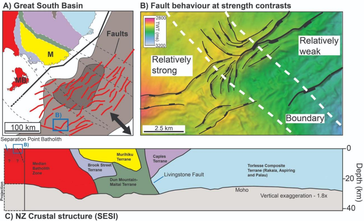
Figure 1: A) Map showing the basement terranes present beneath the South Island of New Zealand and their offshore projections beneath the Great South Basin. Offshore terrane projections after Ghisetti, 2010 and Mortimer et al., 2002. MB - Median Batholith; M - Murihiku Terrane. Main faults are shown after Sahoo et al., 2020. B) TWT structure map showing how faults splay and rotate along internal strength contrasts, after Phillips and McCaffrey, 2019. C) Generalised crustal structure offshore of the eastern coast of the South Island of New Zealand based on the SESI seismic survey, after Mortimer et al., (2002). The southern end of the line is projected to incorporate the Separation Point Batholith along the southern margin of the Median Batholith Zone, and the hypothesised location of panel B is also shown.
