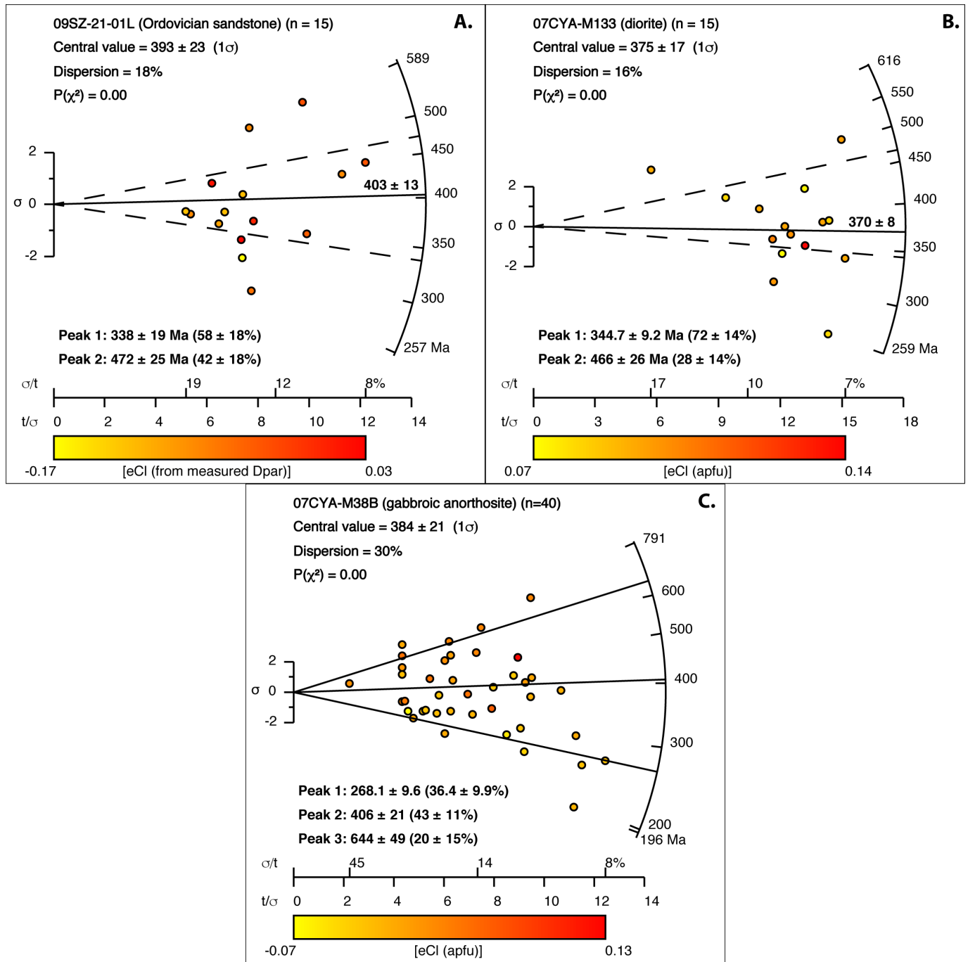
Figure 5: Radial plots for apatite fission-track samples from Southampton Island, Nunavut. (A) Ordovician sandstone sample 09SZ-21-01L is reported in Lavoie et al. [94], Pinet et al. [92]. (B) Diorite sample 07CYA-M133 and (C) gabbroic anorthosite sample 07CYA-M38B are samples from Precambrian basement. Radial plots [49] are a way to visualize single-grain ages and precision and are here coloured by eCl expressed in atoms per formula unit (apfu). Higher grain-age precision is denoted by greater distance from the origin. Grain ages that fall far outside of the 2\sigma bounds typically lead to \chi^2 failure. Age mixture modelling is done in DensityPlotter software v. 8.4 [63, 64] and results in the identified age populations, which are labelled as peaks 1, 2, and 3. Samples in panels (A) and (B) ‘auto’ pick two populations but, based on the overall age dispersion ( <20\% ) and the grain chemistry, those populations are unable to be verified with the available data, so only one population is selected for modelling.
