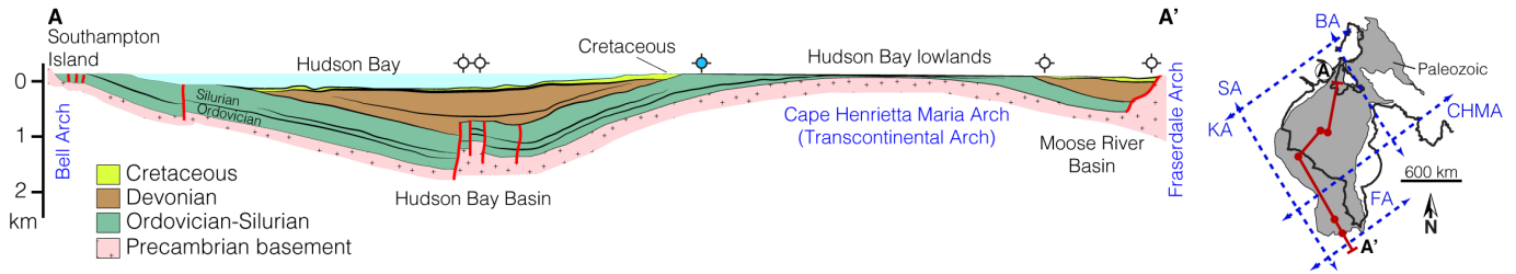
Figure 4: Geological cross-section across Hudson Bay Basin (modified from Norris et al. [112]). The Phanerozoic geology is simplified and coloured according to sequences in Sloss [113]. Red lines are intrabasin faults. Major regional arch structures are shown in the inset as dashed blue lines: Bell Arch (BA); Cape Henrietta Maria Arch (Transcontinental arch) (CHMA); Fraserdale Arch (FA); Keewatin Arch (KA); Severn Arch (SA; trending northwest). The dark red line (A–A' in the cross-section) extends from Southampton Island to the Moose River Basin and the points along the line correspond to drilled exploration wells in the Hudson Bay Basin (Comeault #1 well, in Manitoba, is third from right in the inset and blue dot on cross-section). Gray area in the inset outlines Paleozoic and younger rocks ( see Pinet et al. [100]).
