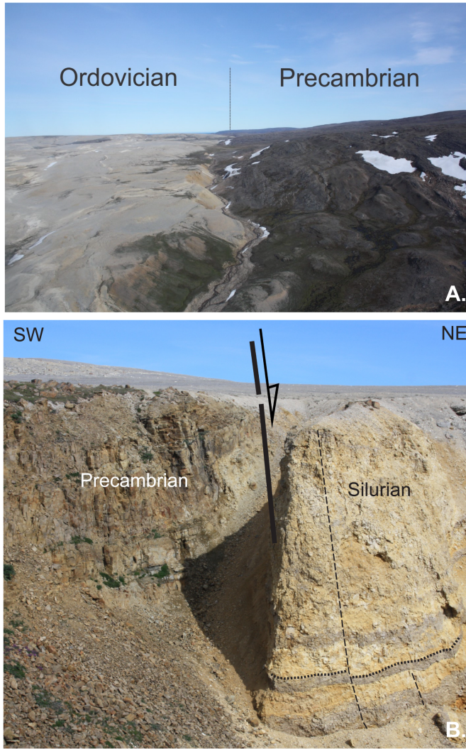
Figure 3: (A) Aerial view showing the shallow-dipping Precambrian–Paleozoic (Ordovician) contact on Southampton Island, Nunavut. Photograph by N. Pinet. NRCan photo 2019-530. (B) Steeply dipping fault juxtaposing Silurian rocks against Precambrian basement near Cape Donovan, on the northeastern shore of Southampton Island. Photograph by N. Pinet. NRCan photo 2019-529.
