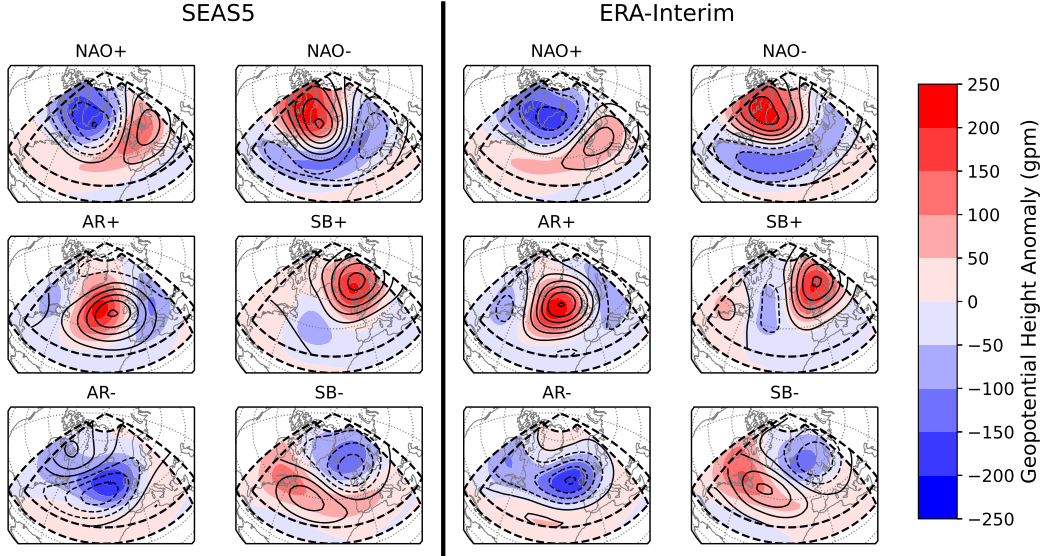
Figure 1: The regimes identified for the ECMWF SEAS5 hindcast ensemble members (left) and ERA-Interim (right) using standard k -means clustering for two slightly different domains (indicated by the dashed boxes). They are the positive and negative phase of the North Atlantic Oscillation (NAO), the Atlantic Ridge (AR+) and its negative counterpart (AR-), and the Scandinavian Blocking (SB+) and its negative counterpart (SB-). Regimes for domain A (20-80N, 90W-30E) are indicated by the colours and those for domain B (30-90N, 80W-40E) by the contours following the same 50 gpm difference between contour levels.
