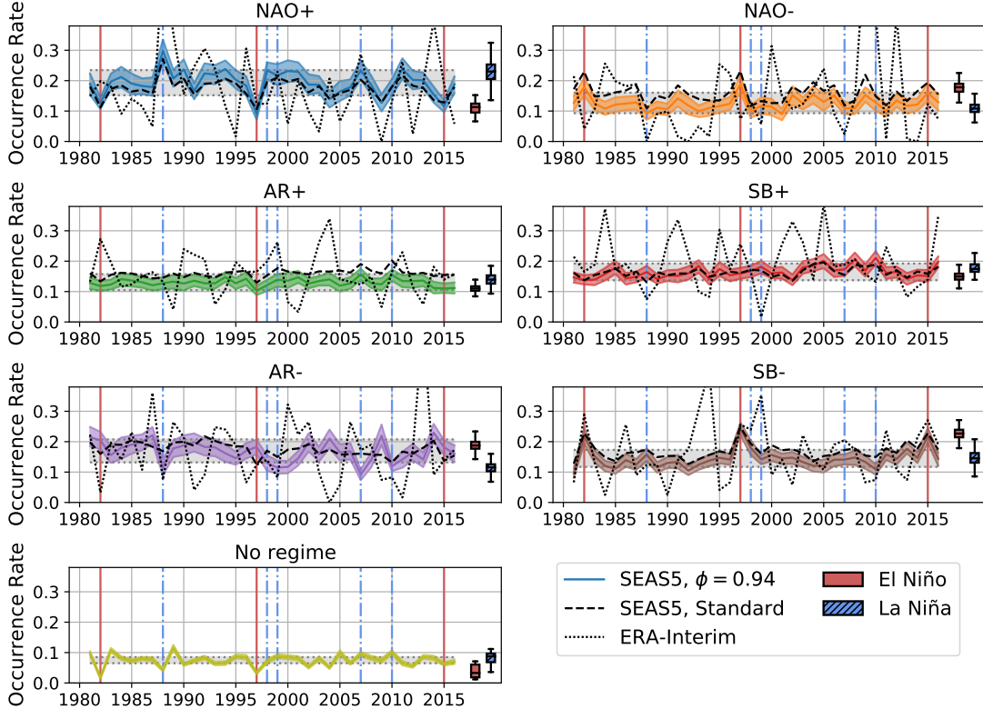
Figure 8: The yearly winter occurrence rates of the different regimes for the constrained results (colour). The grey bands give a noise level, the dashed black line shows the unconstrained SEAS5 results and the dotted black line the ERA-Interim occurrence rates. The bandwidth is given by the 2-standard-deviation range when using bootstrapping with 25 ensemble members, where for the noise level ensemble members for different (random) years are considered. On the right the average occurrence rates of very strong El Niño years (indicated by the solid red lines) and strong La Niña years (indicated by the dash-dotted blue lines) are shown.
