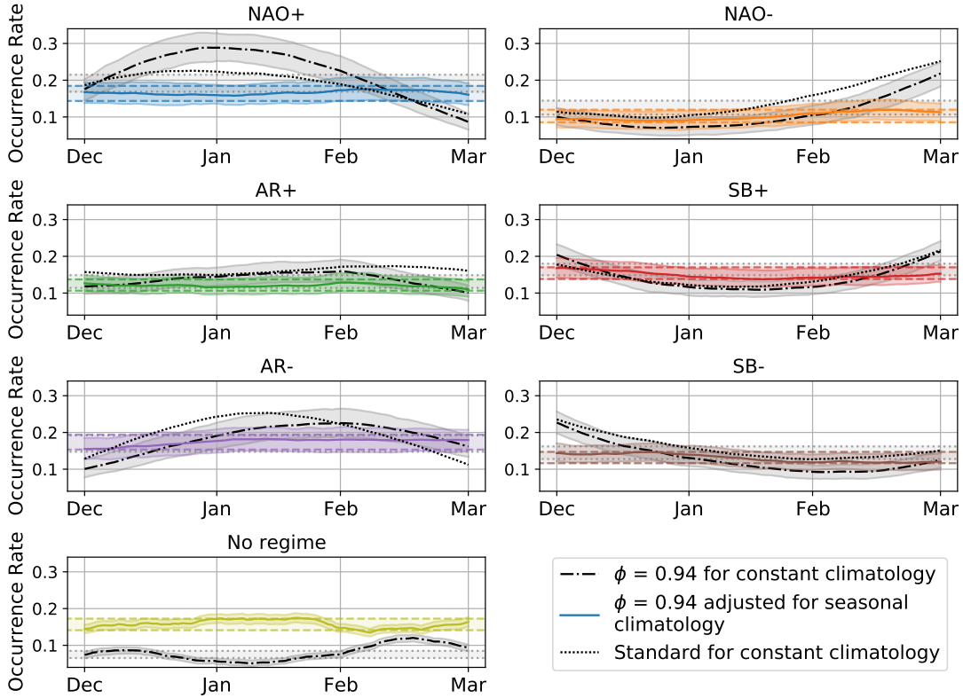
Figure 7: The sub-seasonal variation in occurrence rates (30-day running mean) of the different regimes for the constrained SEAS5 results with respect to a constant climatology (grey, dash-dotted black line) and corrected for a seasonally varying background state (colour, solid colour line) with the shaded area corresponding to the 2-standard deviation range. The shaded areas bounded by the dotted and dashed lines give the 2-standard deviation noise level for the constant and seasonal climatology results respectively. Error bounds are determined using bootstrapping with 3 members for every 30-day period in each year. In addition the sub-seasonal variation obtained using standard k -means clustering for SEAS5 is shown by the black dotted line.
