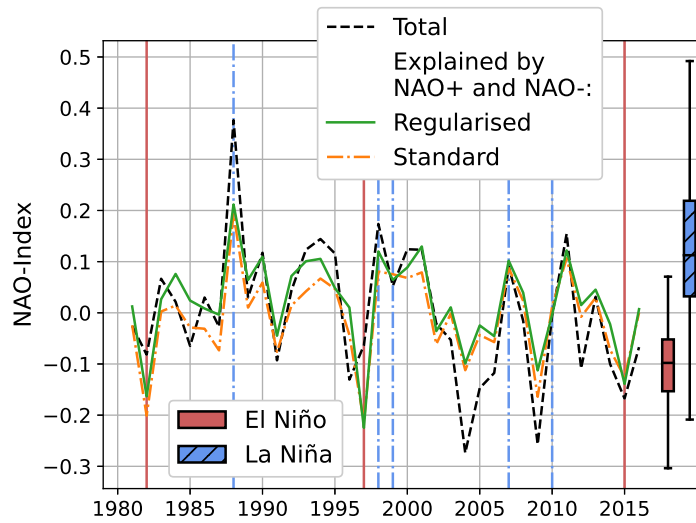
Figure 10: The SEAS5 NAO-index (black, dashed) and an approximation using the NAO+ and NAO- occurrence rates and projected NAO-indices for the regularised (green, solid) and standard (orange, dash-dotted) approach. On the right the average NAO-indices of very strong El Niño years (indicated by the solid red lines) and strong La Niña years (indicated by the dash-dotted blue lines) are shown.
