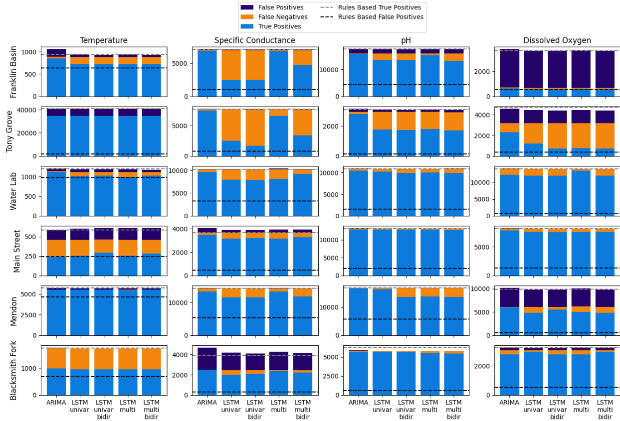
Figure 6: Detection confusion matrix values for all time series (panels) and models (bars). y-axis values represent the count of observations that fall within each category shown in the legend. Dashed lines differentiate the proportions of detections from the rules based detection and the model based detection.
