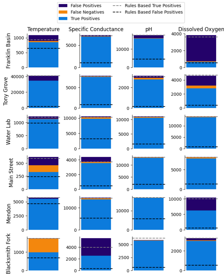
Figure 7: Detection confusion matrix values for aggregate results for all time series. Symbology is as described for Figure 6.
