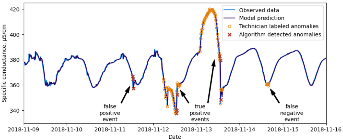
Figure 5: Examples of anomalies detected using an ARIMA model for specific conductance at Tony Grove.
