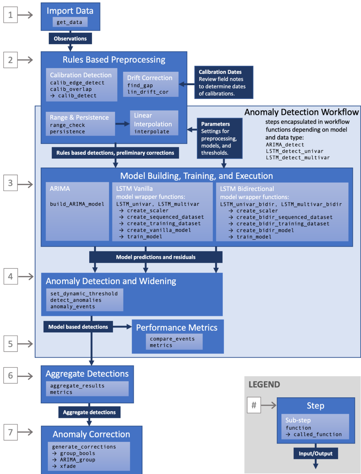
Figure 1. Workflow for steps and functions in PyHydroQC. Numbers on the left correspond to steps in the process listed in Section 2.1.
