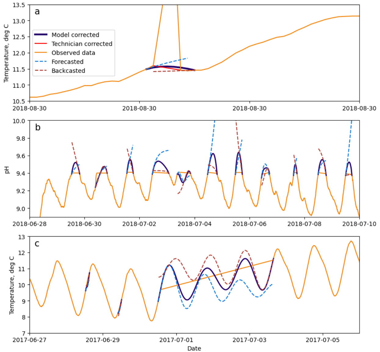
Figure 8: Examples of successful correction using piecewise ARIMA models and the cross-fade technique. 8a: temperature at Water Lab, 8b: pH at Main Street, 8c: temperature at Water Lab.
