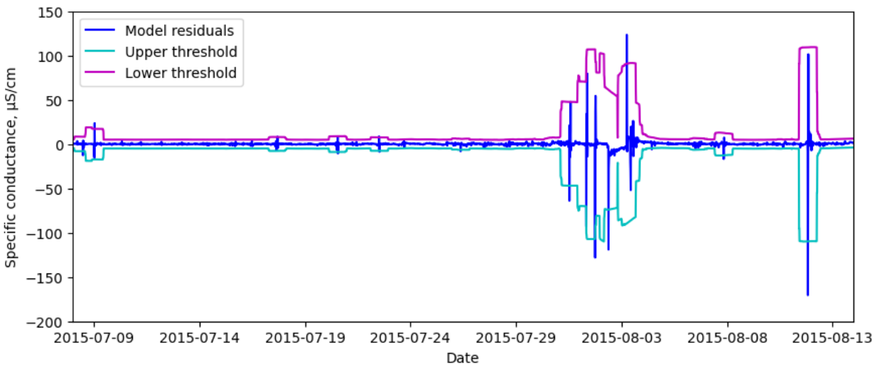
Figure 4: Example of model residuals and dynamic thresholds for specific conductance at Main Street.
