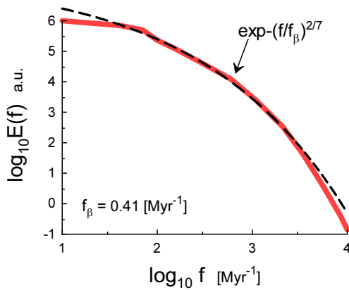
FIG. 15: Power spectrum of the axial dipole magnetic field (numerical simulation, Rm = 564 ).
