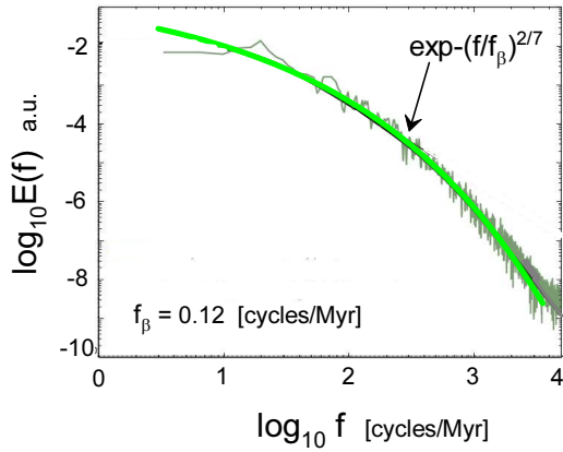
FIG. 14: Power spectrum of the axial dipole magnetic field (numerical simulation, Rm = 90 ).
