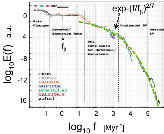
FIG. 17: Extended composite (with a modified composition) power spectrum of geomagnetic dipole moment variations for the time interval 0-160 Myr.
