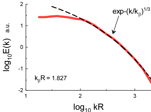
FIG. 13: Crustal magnetic power spectrum computed using the World Magnetic Anomaly Map.
