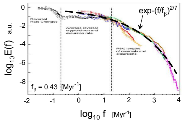
FIG. 16: Composite power spectrum of geomagnetic dipole moment variations for the time interval 0-160 Myr.
