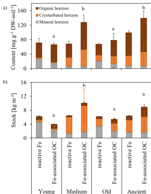
Figure 4 | Reactive Fe and associated OC a) content in \text{mg g}^{-1} \text{DW-soil}^{-1} and b) stock in \text{kg m}^{-2} of in distinct soil horizons (organic: brown, cryoturbated/buried: orange, grey: mineral) along the soil chronosequence. Distribution of reactive Fe and associated OC contents highlight the role of organic horizons, whereas cryoturbated horizons are more important regarding stocks along the soil chronosequence. Reactive Fe is dithionite-citrate extractable Fe corrected by NaCl control extraction and Fe-associated OC is dithionite-citrate extractable OC corrected by NaCl control extraction and citrate background. Error bars represent a combined range of duplicate extractions per horizon of replicate soil cores. Significant differences between age classes are highlighted with letters a and b.
