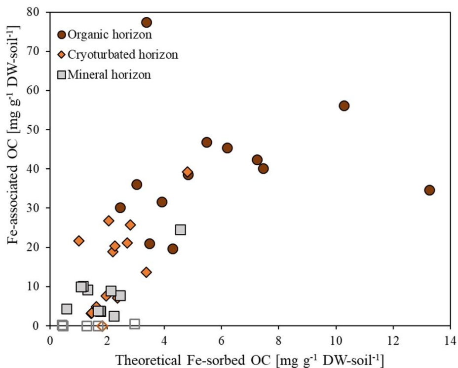
Figure SI 4 | Content of Fe-associated OC against theoretical maximum adsorption of OC to iron oxide surfaces, calculated as 0.22 times the reactive Fe content based on Wagai and Mayer (2007) following Herndon et al. (2017). Reactive Fe is dithionite-citrate extractable Fe corrected by NaCl control extraction and Fe-associated OC is dithionite-citrate extractable OC corrected by NaCl control extraction and citrate background, presented as mg g -1 DW-soil -1 . Filled symbols represent samples with OC:Fe mass ratios >0.22 and framed symbols are below a ratio of 0.22.
