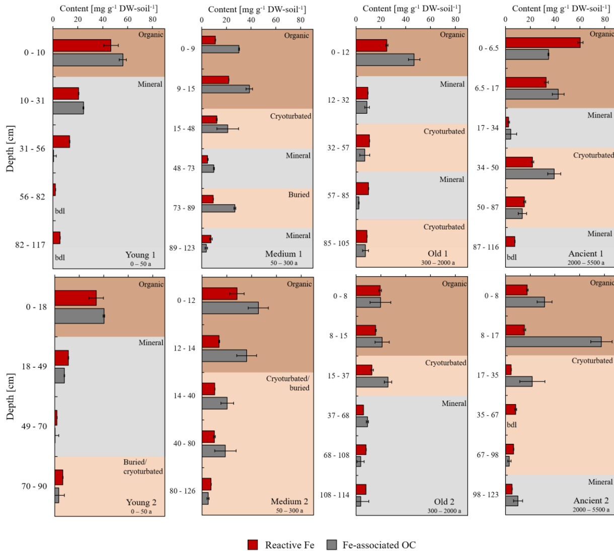
Figure 2 | Soil horizons determine the content of reactive Fe (red) and Fe-associated OC (grey) along the soil profile of replicate cores (1, 2) from four age classes (young, medium, old, ancient) of drained thaw lake basins from Alaska. Reactive Fe is dithionite-citrate extractable Fe corrected by NaCl control extraction and Fe-associated OC is dithionite-citrate extractable OC corrected by NaCl control extraction and citrate background, presented as \text{mg g}^{-1}\text{DW-soil}^{-1} . Soil horizons are highlighted by color shading (brown: organic, beige: cryoturbated/buried, grey: mineral). Error bars represent a combined range of duplicate extractions per horizon of replicate soil cores.
