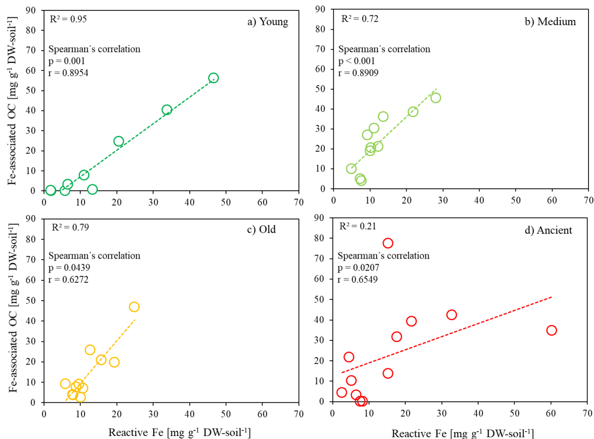
Figure SI 3 | Age dependent correlation of reactive Fe and Fe-associated OC of soil profiles of replicate cores (1, 2) from four age classes (young, medium, old, ancient) of drained thaw lake basins from Alaska. ( n = 43 ). Divided into (a) young (dark green, n = 9 ), (b) medium (light green, n = 11 ), (c) old (yellow, n = 11 ) and (d) ancient (red, n = 12 ) illustrating increasing heterogeneity with age. Reactive Fe is dithionite-citrate extractable Fe corrected by NaCl control extraction and Fe-associated OC is dithionite-citrate extractable OC corrected by NaCl control extraction and citrate background, presented as \text{mg g}^{-1} \text{DW-soil}^{-1} . Data points represent average from duplicate extraction with linear trendlines highlighted in respective colors. R squared of linear regression and Spearman correlation coefficients are given within the figure.
