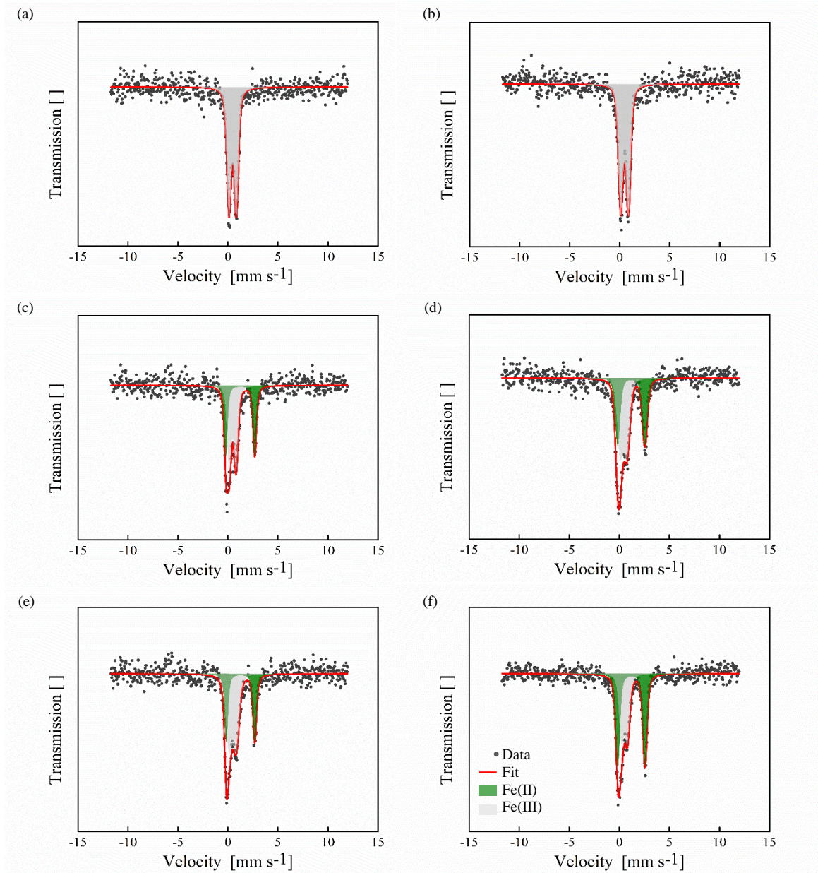
Figure SI 5 / Mössbauer transmission spectra collected at 77 K for (a) Young 1 – organic, (b) Ancient 1 – organic, (c) Young 2 – cryoturbated, (d) Ancient 1 – cryoturbated, (e) Young 1 – mineral and (f) Ancient 1 – mineral horizons of young and ancient soil cores along a permafrost soil chronosequence in northern Alaska.
