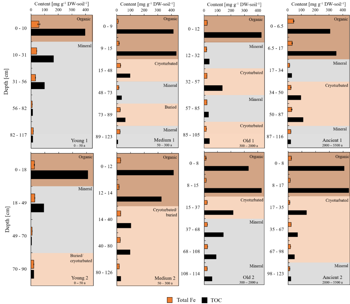
Figure SI 2 | Content of total Fe (orange, 6 M HCl extractable) and TOC (black) in \text{mg g}^{-1} \text{DW-soil}^{-1} along the soil profile of replicate cores (1, 2) from four age classes (young, medium, old, ancient) of drained thaw lake basins from Alaska. Soil horizons are highlighted by color shading (brown: organic, beige: cryoturbated/buried, grey: mineral). Error bars of total Fe represent the range from duplicate extractions per each soil horizon. TOC data was obtained by Mueller et al. (2015).
