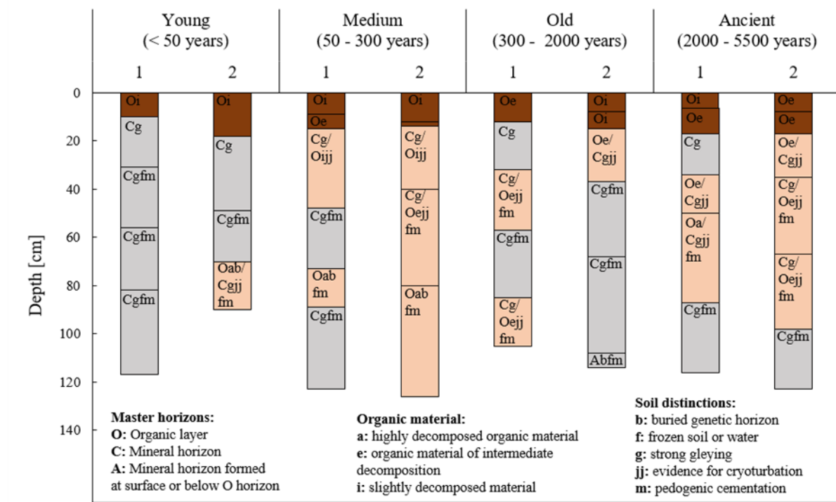
Figure 1 | Classification according to Mueller et al. (2015) and description of soil horizons of replicate soil cores of the four different age classes. Abbreviations assigned to the distinct soil horizons are described below the figure. Colors indicate organic horizons (brown), cryoturbated/buried horizons (beige) and mineral horizons (grey).
