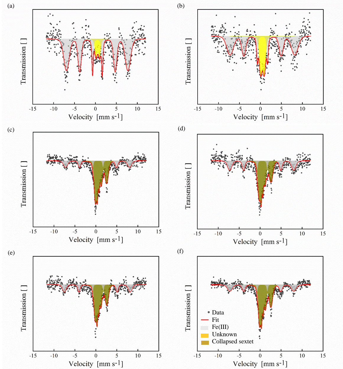
Figure SI 6 | Mössbauer transmission spectra collected at 5 K for (a) Young 1 – organic, (b) Ancient 1 – organic, (c) Young 2 – cryoturbated, (d) Ancient 1 – cryoturbated, (e) Young 1 – mineral and (f) Ancient 1 – mineral horizons of young and ancient soil cores along a permafrost soil chronosequence in northern Alaska.
