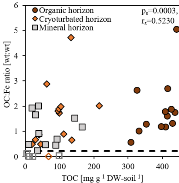
Figure 5 | OC:Fe mass ratios in relation to the TOC content in \text{mg g}^{-1} DW-soil -1 separated into organic horizons (brown circle), cryoturbated/buried horizons (orange diamond) and mineral horizons (grey square) of replicate cores (1, 2) from four age classes (young, medium, old, ancient) of drained thaw lake basins from Alaska. OC:Fe mass ratios were calculated using reactive Fe and Fe-associated OC contents. Reactive Fe is dithionite-citrate extractable Fe corrected by NaCl control extraction and Fe-associated OC is dithionite-citrate extractable OC corrected by NaCl control extraction and citrate background. The dashed line represents the presumed threshold for sorption of reactive Fe minerals on natural organic matter (Wagai and Mayer, 2007). OC:Fe mass ratios largely
