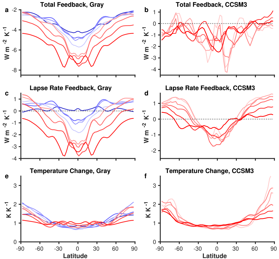
FIG. 5. Total feedback parameter for the (a) gray radiation GCM and (b) CCSM3. Lapse rate feedback parameter for the (c) gray radiation GCM and (d) CCSM3. Normalized surface air temperature change ( \Delta T_s(\phi) \times \langle \Delta T_s \rangle^{-1} ) for the (e) gray radiation GCM and (f) CCSM3. Colors are proportional to the global-mean temperature, with darker blues coldest and darker reds warmest, and similar colors indicate similar global-mean surface temperature across the two GCMs. Note that the vertical axes change from left to right and the idealized GCM panels show eight of the sixteen simulations for clarity.
