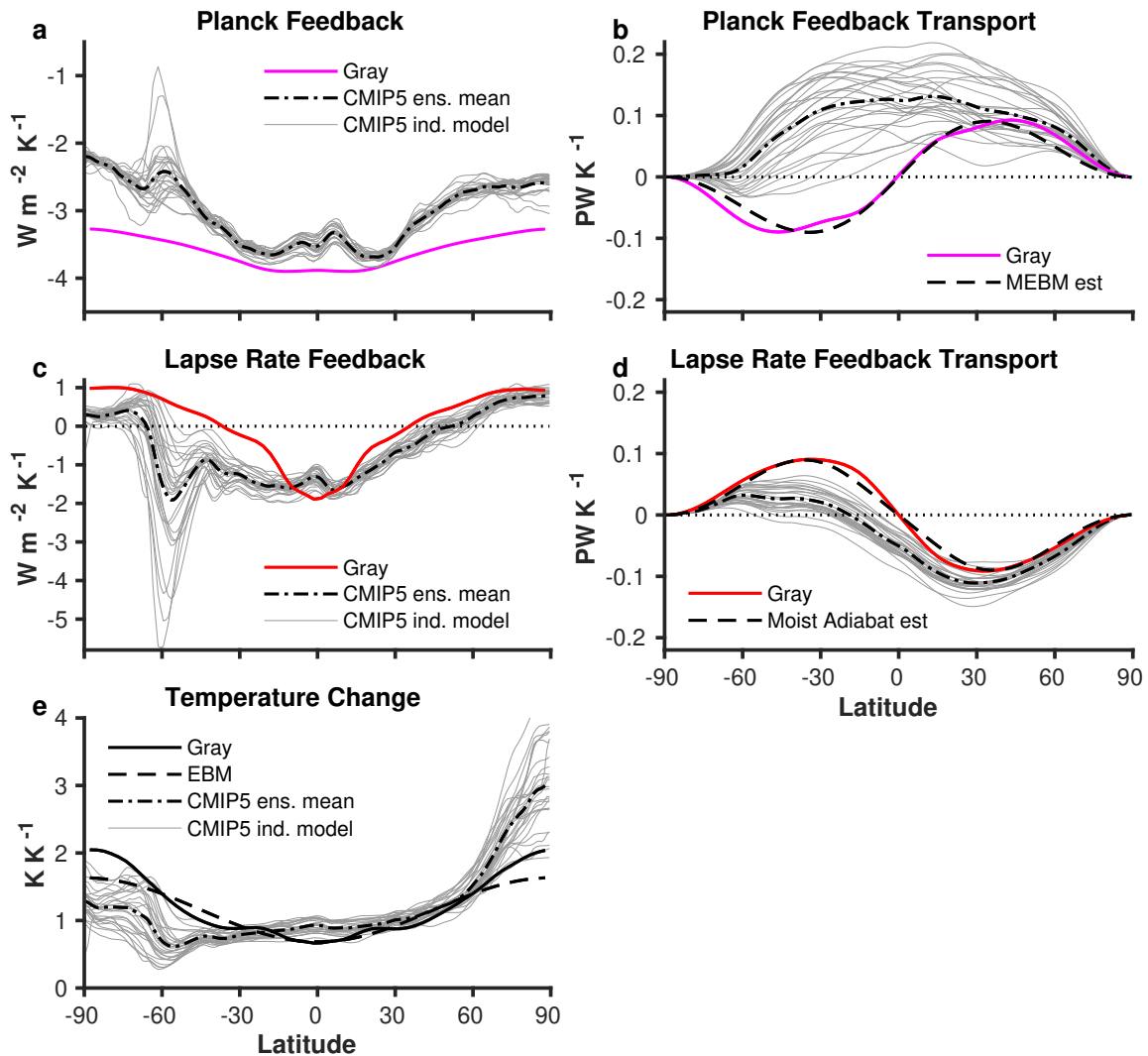
Fig. 3. Planck feedback (a) parameter and (b) the associated energy transport for the gray radiation GCM (magenta line), CMIP5 ensemble mean (black dot-dashed line), individual CMIP5 models (thin gray lines), and the moist energy balance model estimate for the transport (black dashed line). Lapse rate feedback (c) parameter and (d) the associated energy transport for the gray radiation GCM (red line), CMIP5 ensemble mean (black dot-dashed line), individual CMIP5 models (thin gray lines), and the moist adiabat estimate for the transport (black dashed line). (e) Normalized surface air temperature change ( \Delta T_s(\phi) \times (\Delta T_s)^{-1} ) for the gray radiation GCM (black solid), moist energy balance model theory (black dashed) CMIP5 ensemble mean (black dashed dotted), individual CMIP5 models (thin gray lines). All gray radiation GCM simulations are evaluated between the control and one that is 6.1 K warmer in the global mean. All CMIP5 results use the 4\times CO_2 scenario.
