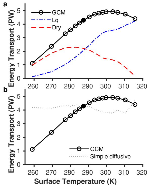
FIG. 1. (a) Vertically integrated northward energy transport at 50° N for GCM simulations (black) indicated by their global-mean surface temperature, with (blue) latent energy and (red) dry static energy transport components. (b) Evaluation of the simple diffusive closure (5) at 50° N using the mean moist static energy gradients at the lowest atmospheric level.
