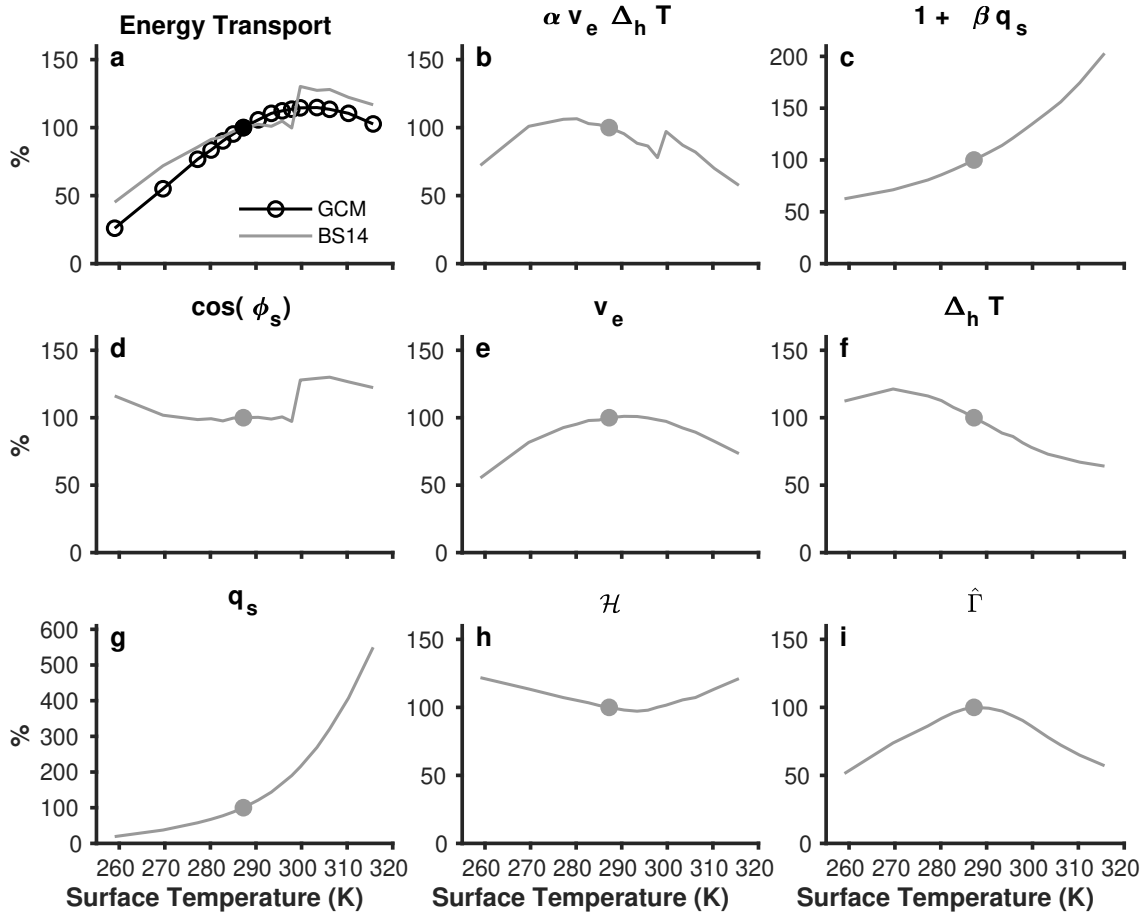
FIG. 6. (a) Percentage change in vertically integrated northward energy transport at 50^\circ N for GCM simulations (black circles) and Bischoff and Schneider (2014) diffusive scaling (6) (gray) relative to the control simulation. (b) Dry component \alpha v_{eddy} \Delta_h T and (c) latent energy modification 1 + \beta q_s of the diffusive closure. (d,e,f,g,h,i) Cosine of storm track latitude \cos(\phi_s) , eddy velocity v_{eddy} , horizontal temperature contrast \Delta_h T , saturation specific humidity q_s , relative humidity \mathcal{H} , and inverse dry static stability parameter \hat{\Gamma} . The control simulation is indicated by the filled symbols, and the GCM averaging conventions are described in section 3. Note that the vertical scales differ in panels c and g.
