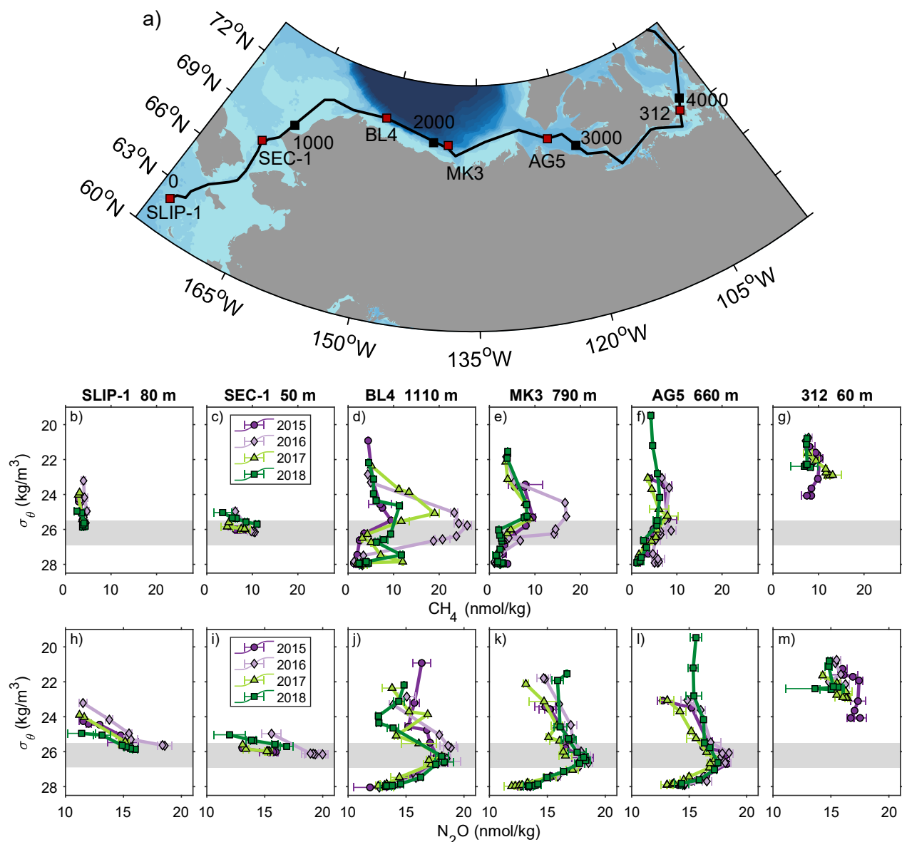
Figure 5. Depth profiles of \text{N}_2\text{O} and \text{CH}_4 concentrations at selected stations sampled in all four years. (a) Map showing station locations and distance along transect (black line, equivalent to the transect shown in Figure 1). Profiles of \text{CH}_4 (b–g) and \text{N}_2\text{O} (h–m) concentrations as a function of potential density anomaly ( \sigma_\theta ); station names and bottom depths are indicated above each column. The grey bar highlights the density surface \sigma_\theta = 25.5\text{--}26.9 , which represents dense waters of the BCSW/BCWW that are transported into the Beaufort Sea. The black numbers represent distance along the transect in km.
