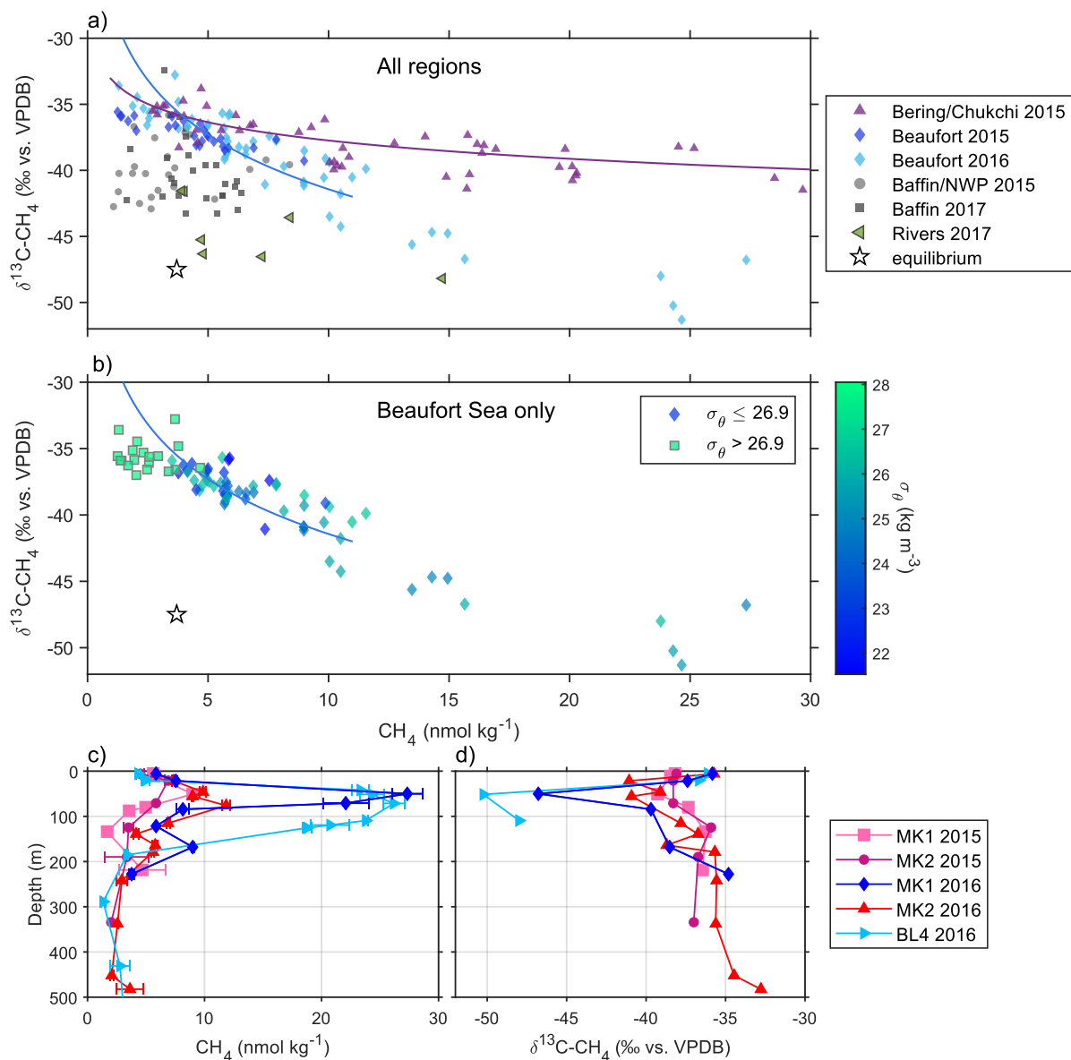
Figure 8. \text{CH}_4 isotope data from 2015–2017. Relationship between \text{CH}_4 and \delta^{13}\text{C-CH}_4 for (a) all data and (b) Beaufort Sea data only. The white star represents \text{CH}_4 at equilibrium with the
