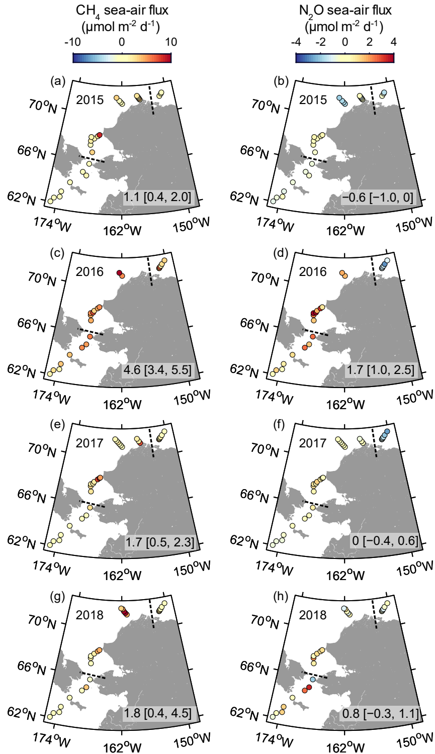
Figure 9. Map of short-term sea-air fluxes ( \mu\text{mol m}^{-2} \text{d}^{-1} ) of CH 4 (left column) and N 2 O (right column) at stations in the Bering, Chukchi and eastern Beaufort Seas from 2015–2018 integrated over the residence time of each gas in the mixed layer prior to the sampling date. Dashed lines indicate boundaries between the Bering, Chukchi and Beaufort Seas. The median [interquartile range] fluxes for each year for the Bering and Chukchi Seas are reported in the lower right corner of each panel. Positive values represent a flux from the sea to the air.
