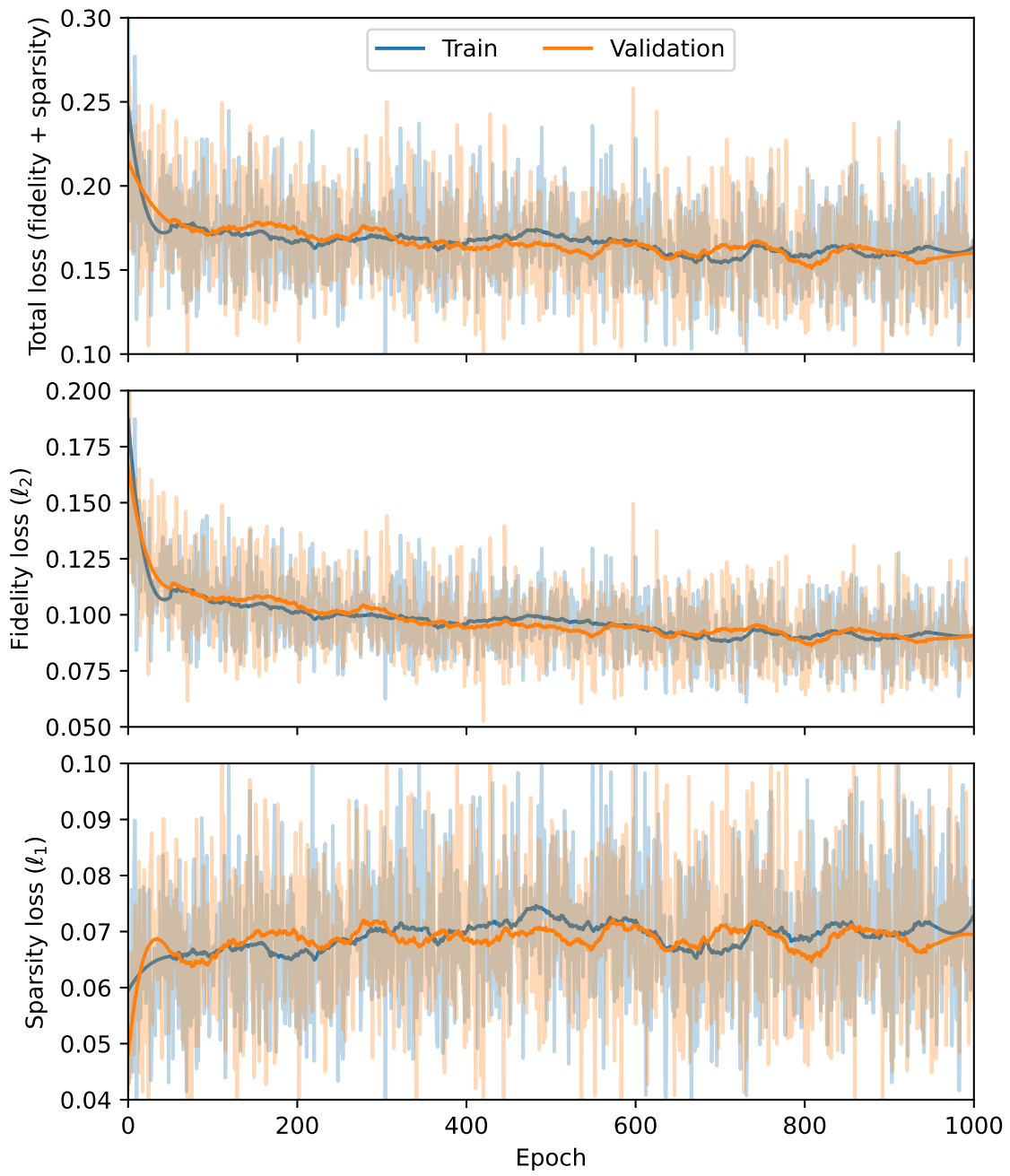
Fig. S1: Evolution of the training and validation loss during the training of the Deep Learning model, over the total period of 1000 epochs.
