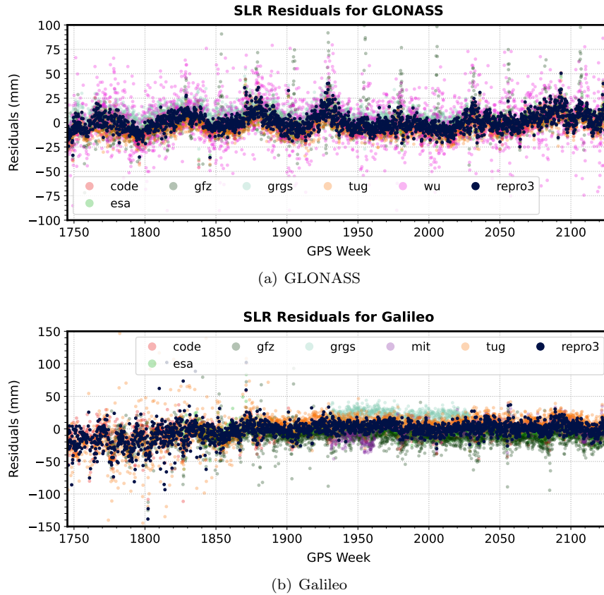
Fig. 3 Average SLR Residuals per constellation for each AC solution and the combination
