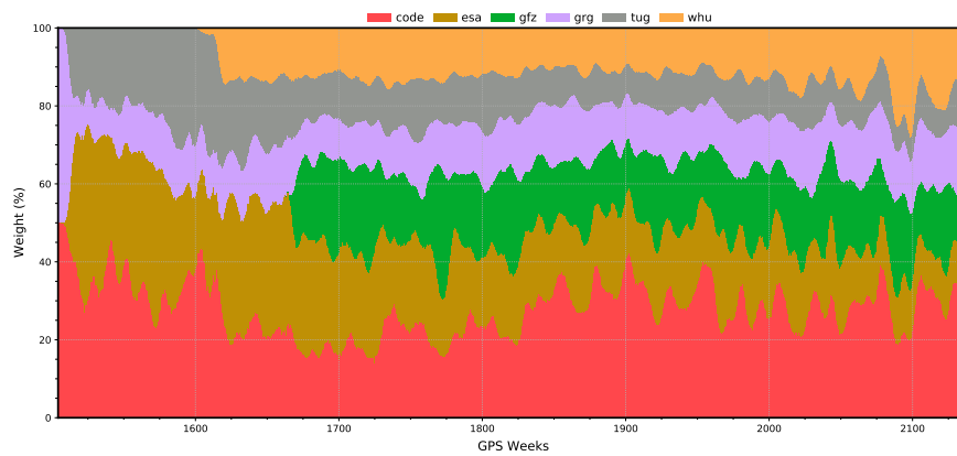
(b) GLONASS
