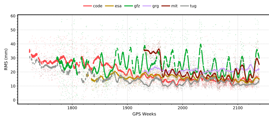
(c) Galileo
