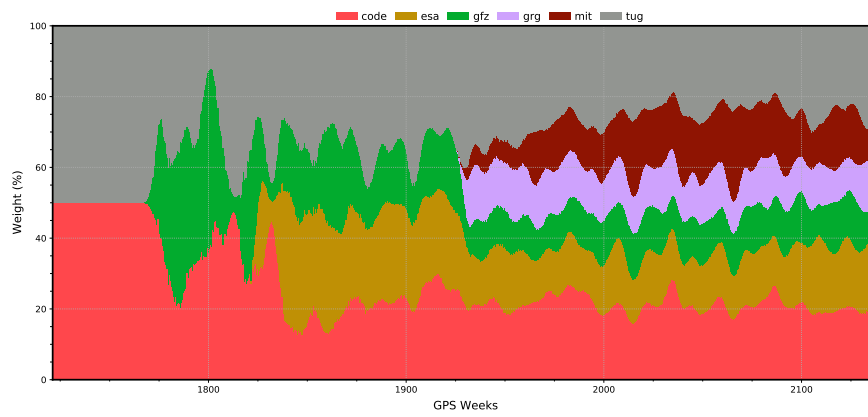
(c) Galileo
