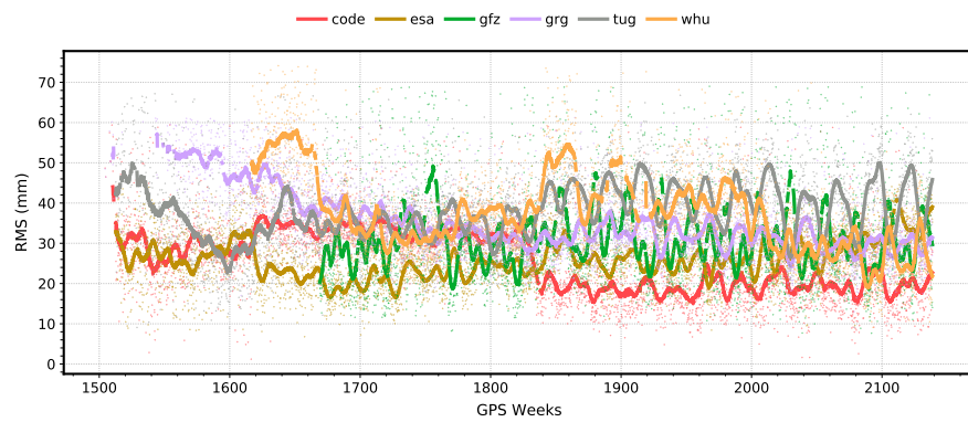
(b) GLONASS
