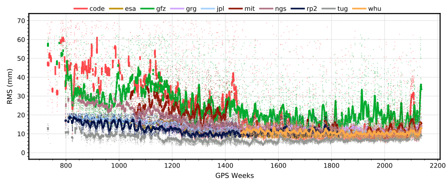
(a) GPS
