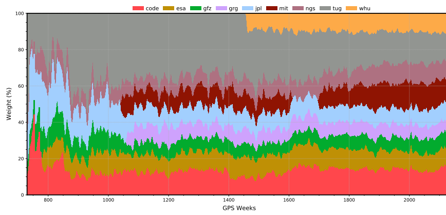
(a) GPS
