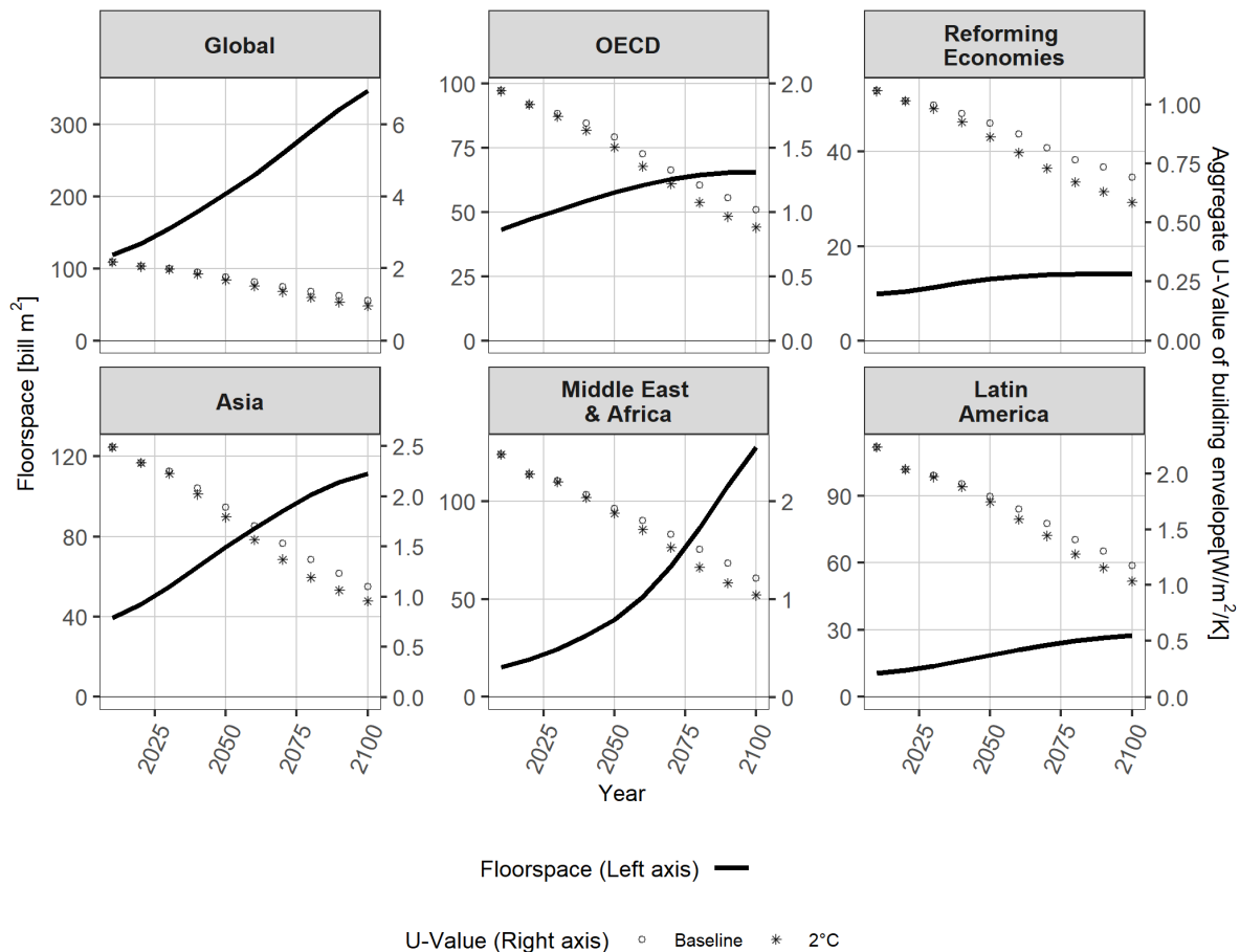
Figure 1. Changes in residential floorspace over the projection period (left axis), and changes in building envelope efficiency (U-value, right axis) in Baseline and 2°C scenarios. Note different scales.
