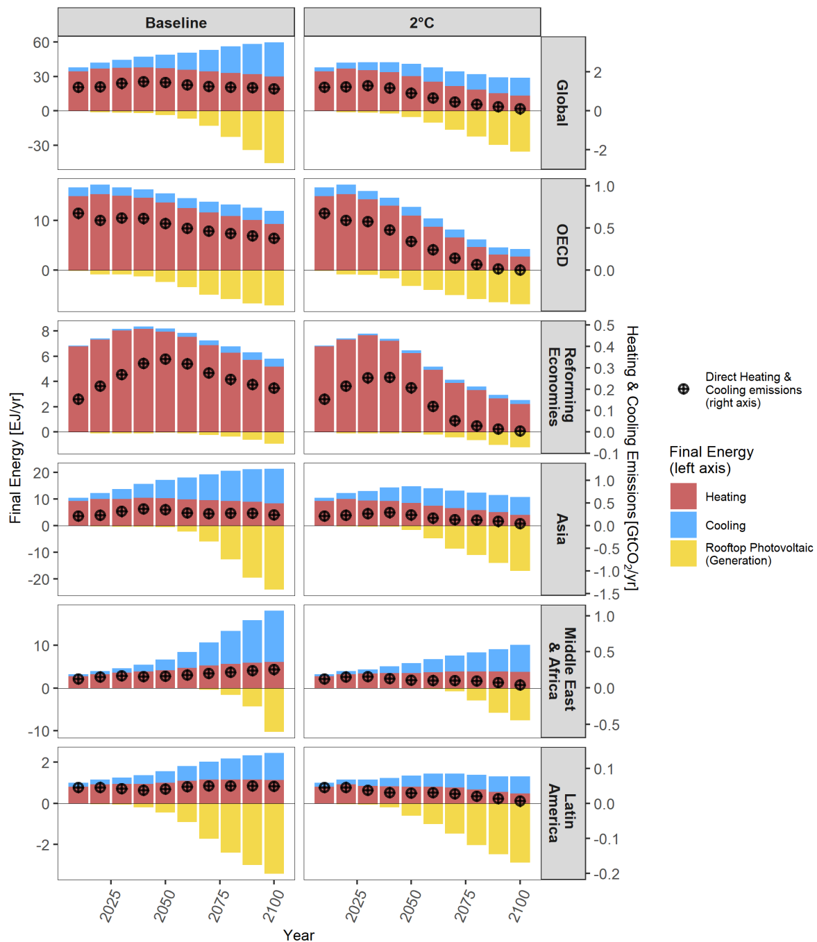
Figure 2. Final energy for residential heating and cooling (coloured bars, left axis), and direct residential emissions (points, right axis). Rooftop PV electricity generation shown as negative demand (left axis). Baseline and 2°C scenarios.
