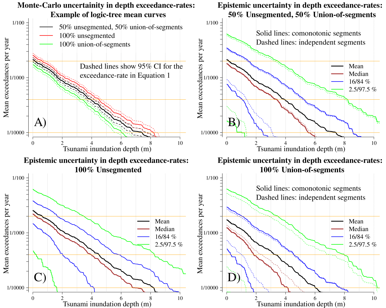
Figure 11: Monte-Carlo and epistemic uncertainties in inundation depth exceedance-rates at Site Q (lon,lat = 184.8017,-21.13305). The background sea-level is 0 m and only Kermadec-Tonga trench thrust scenarios are included. A) Logic-tree-mean curves for 3 different scenario-frequency representations, with 95% confidence-intervals (computed via Equation 25) for the exceedance-rate in Equation 1. B) Epistemic uncertainties in the inundation-depth exceedance-rates. Percentiles vary slightly if the segments are treated as comonotonic (solid lines) or independent (dashed lines). C) Same as panel B but with 100% weight on the unsegmented source representation. D) Same as panel B but with 100% weight on the union-of-segments source representation.
