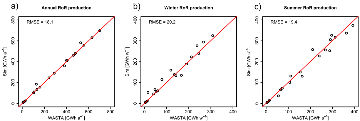
Figure 5. Comparison of the mean simulated production with production reported in WASTA for the 21 RoR plants: a) annual production, b) winter production (Oct-Mar) and c) summer production (Apr-Sep).
