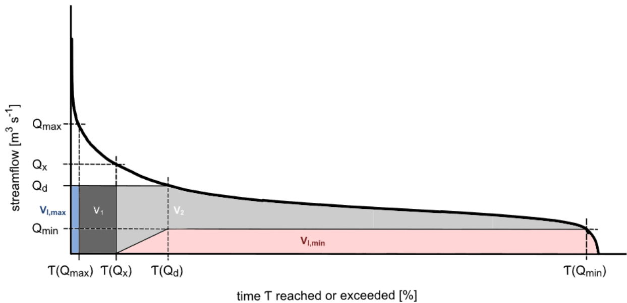
Figure 4. Illustration of the estimation of the hydrologic production potential based on the Flow Duration Curve (FDC), characterised by the parameters Q_{max} [ m^3 s^{-1} ], Q_d [ m^3 s^{-1} ] and Q_{min} [ m^3 s^{-1} ]. \tau(Q_x) [%] designates the duration during which the streamflow reaches Q_d + Q_{min} , adapted from the work of (Hänggi and Weingartner 2012). V_{l,max} and V_{l,min} indicate the loss due to Q_{max} or Q_{min} .
