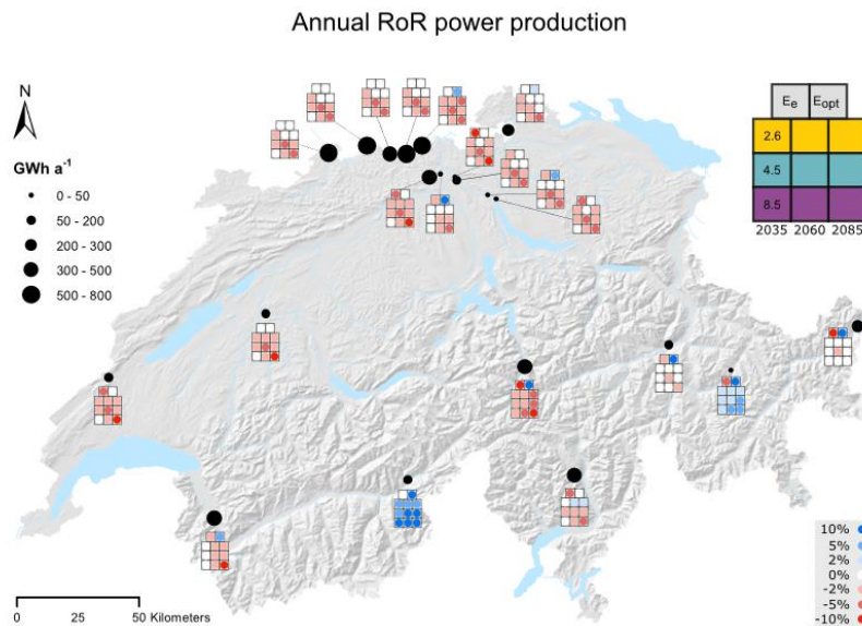
Figure 8. Simulated production changes of the 21 RoR power plants; the size of the power plants represents the annual production in GWh a -1 , the colored dots represent the loss due to environmental flow requirements ( E_e ), the increase potential due to the optimisation of the design discharge ( E_{opt} ) and the climate change impact for the periods 2035 (near future, 2020–2049), 2060 (mid-century, 2045–2074) and 2085 (end of century, 2070–2099) under the three emission scenarios RCP2.6 (yellow), RCP4.5 (blue) and RCP8.5 (purple).
