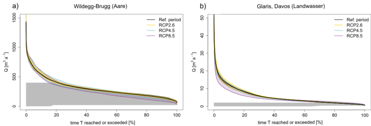
Figure 7. Flow Duration Curves (FDCs) for the power plants a) Wildegg-Brugg and b) Glaris, Davos. The black line represents the reference period (1981–2010), the grey shaded area represents the expected available streamflow ( V_{exp} ), and the areas bounded by yellow (RCP2.6), blue (RCP4.5) and purple (RCP8.5) curves represent the range of FDCs for the projected model ensembles within the three emission scenarios for the end of the century.
