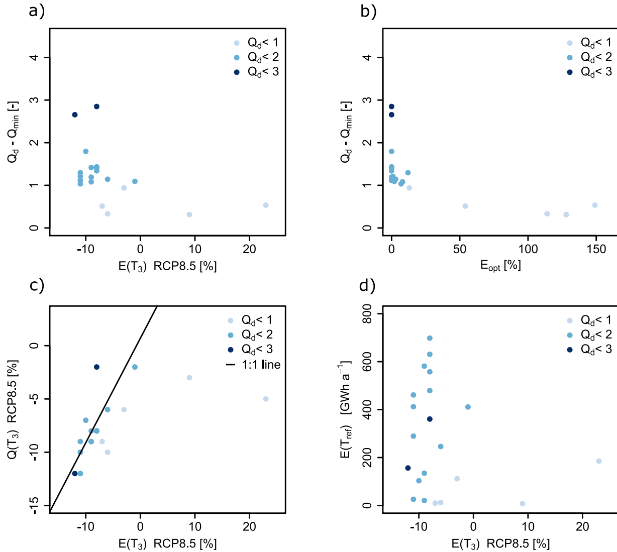
Figure 11. Negative spearman correlation between a) future ( T_3 under the emission scenario RCP8.5) annual production changes and the range [-] of usable streamflow volume (the difference between normalised design discharge Q_d and normalised environmental flow Q_{min} ) and b) between the production increase potential [%] and the range [-] of usable streamflow volume. And a comparison of c) streamflow changes [%] and production changes [%] ( T_3 , RCP8.5) complemented with a linear line and d) the annual production [ GWh a^{-1} ] during the reference period ( T_{ref} ) compared to the projected production changes [%] by the end of the century ( T_3 , RCP8.5). The colors of the dots represent the normalised (by the mean streamflow) design discharge ( Q_d ) of the 21 RoR power plants; the darker the dot, the more streamflow is used for production.
