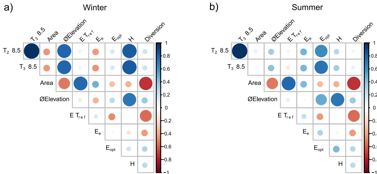
Figure 10. Correlation matrix for a) winter (Oct-Mar) and b) summer (Apr-Sep) Run-of-River (RoR) power production: the simulated production changes of the emission scenario RCP8.5 for the two future periods: T_2/2060 [%] and T_3/2085 [%], catchment Area [ km^2 ], mean Elevation of the catchment [ m a.s.l.], the mean annual production of the reference period ( E T_{ref} [ GWh a^{-1} ]), the loss due to environmental flow requirements ( E_e [%]), the increase potential due to optimising the design discharge ( E_{opt} [%]), the hydraulic head H [ m ] and if streamflow is diverted (Diversion [Yes;No]). The blue dots indicate a positive, the red dots a negative correlation. The larger the dots are, the stronger the correlation is.
