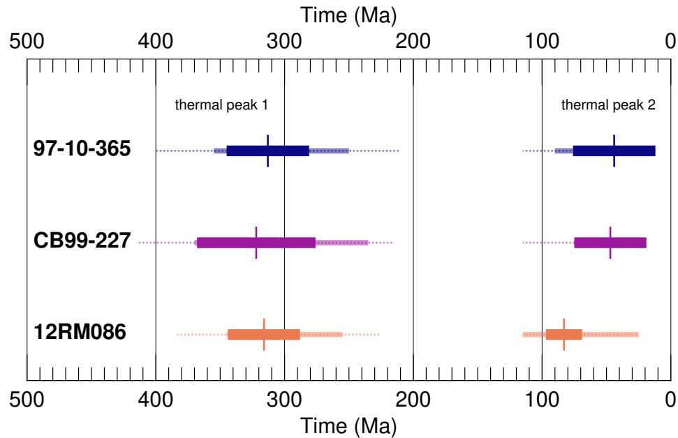
Fig. 9. Thermal episode summary for the AFTINV inverse thermal history models exhibiting two thermal peaks. Dotted line shows the minimum-maximum time range at the 0.05 significance level for each thermal peak for each sample. Thick transparent line represents the minimum-maximum time range at the 0.5 significance level. The vertical bar and opaque heavy lines show the mean \pm 2\sigma time for each thermal peak at the 0.5 level. Refer to table 4 for tabulated information.
