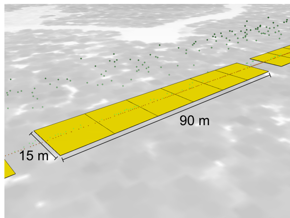
Figure 5: ICESat-2 track segmentation scheme: one 90 m x 15 m track segment consists of six 15 m x 15 m cells for which the reference AGBs were predicted using ALS and Sentinel-2 data. ATL03 photons are colored by classification.
