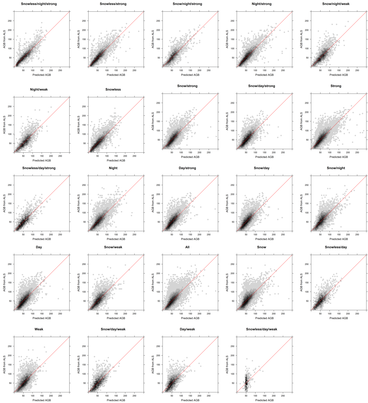
Figure 7: Density scatter plots of the submodels, in the same order as in Table 1.
