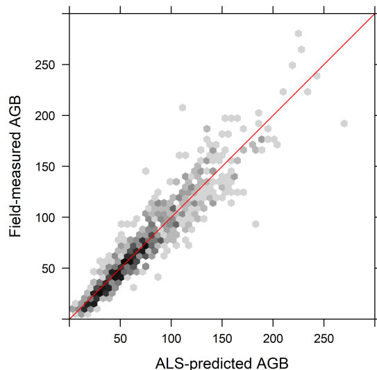
Figure 6: Scatter density plot of the field-plot AGB vs. AGB predicted from ALS using model 5.
