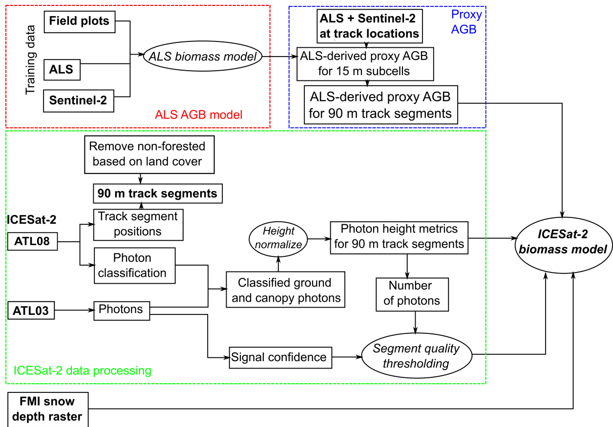
Figure 1: Workflow for the ICESat-2 AGB modeling.
