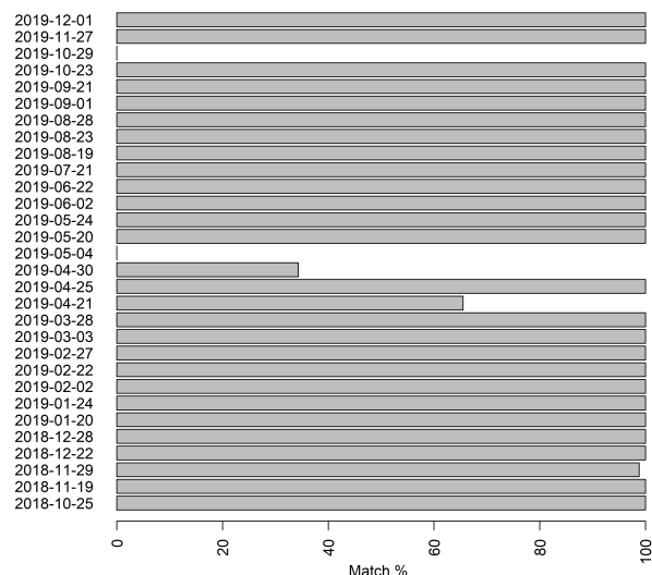
Figure 4: Comparison of ATL08 and FMI snow cover data by imaging date. Match % is the percentage of track segments with a similar snow status in ATL08 and the FMI snow rasters by date.
