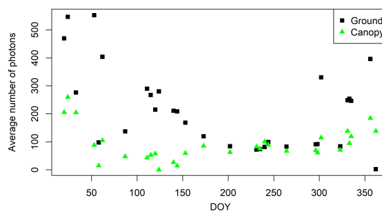
Figure 8: Average number of ground (black square) and canopy (green triangle) photons per segment versus day of the year.
