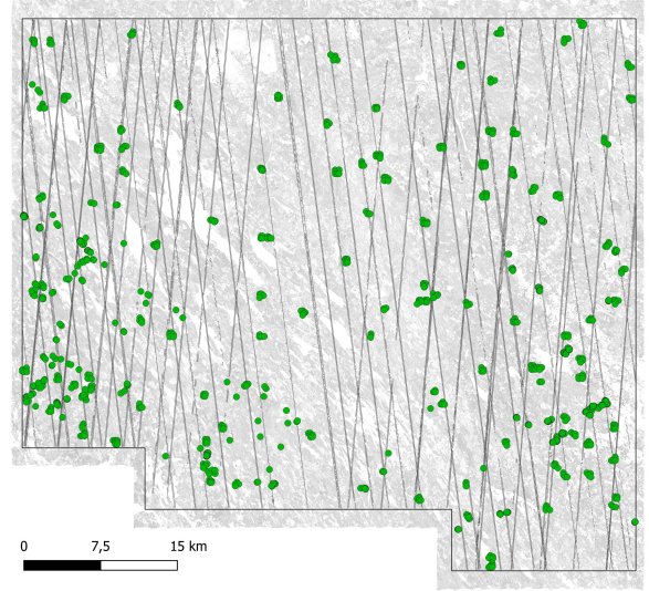
Figure 3: Locations of field plots (green dots) and ICESat-2 tracks in the study area, superimposed on canopy height model raster.
