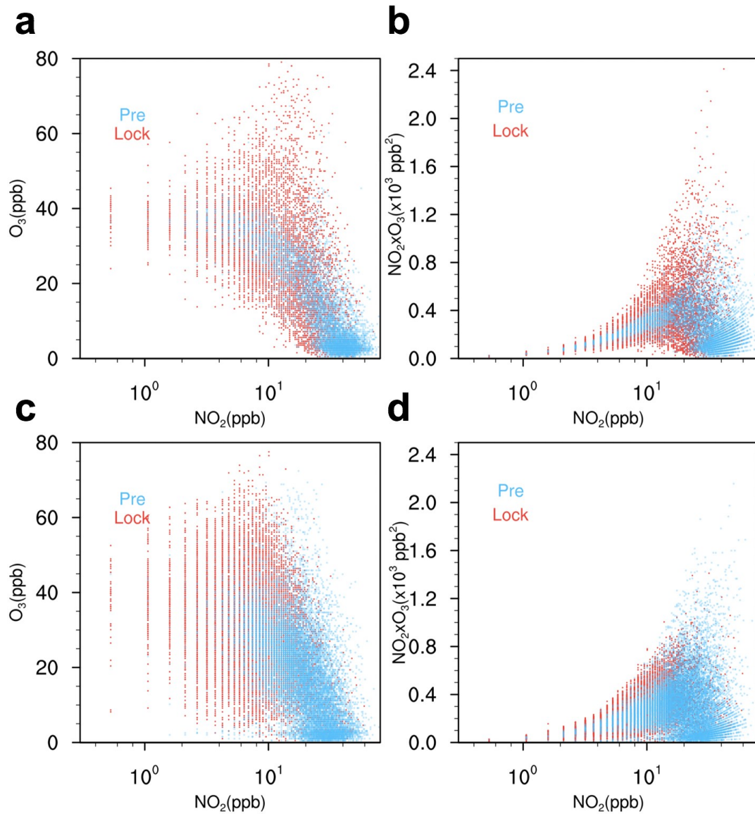
Extended Data Fig. 11 | Observed non-linear relationship between main oxidants and \text{NO}_2 caused by the COVID-19 lockdown in China. a, b, Scatter plots of \text{O}_3 and proxy of \text{NO}_3 radical ( \text{NO}_2 \times \text{O}_3 ) versus \text{NO}_2 between the COVID-lock and pre-COVID periods in BTH of China. c, d, Same as a and b but for the YRD region.
