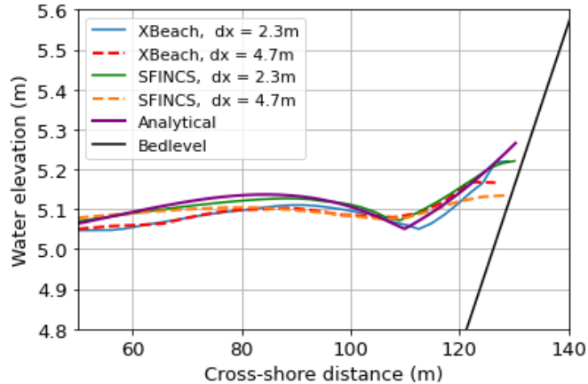
Figure 12. Comparing the maximum elevation height achieved at every point in the domain over the entire simulation when using SFINCS and XBeach at dx = 2.3\text{m} and dx = 4.7\text{m} (corresponding to 64 and 32 mesh cells in the x -direction respectively) with the analytical result for the Carrier-Greenspan test case. A slope of 0.041 is used in all simulations. Note that the water elevation height does not always meet the bedlevel because the bedlevel is slightly differently defined at the different resolutions.
