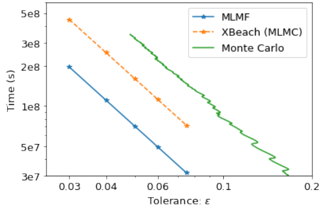
Figure 30. Comparing the computational cost required to achieve tolerance \epsilon at all locations using MLMF, XBeach with MLMC and Monte Carlo for the Myrtle Beach test case
