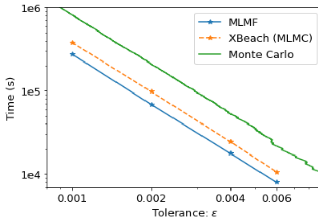
Figure 19. Comparing the computational cost required to achieve tolerance \epsilon using MLMF, XBeach with MLMC and the Monte Carlo method for the Carrier-Greenspan test case.
