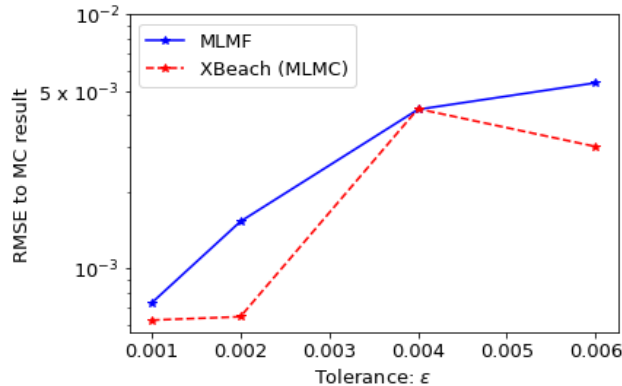
Figure 15. Error (RMSE) between the MLMF result and the Monte Carlo (MC) result for the Carrier-Greenspan test case as the tolerance value \epsilon in (Eq. 26) is varied. This is compared to the error when varying \epsilon in (Eq. 14) for MLMC with XBeach.
