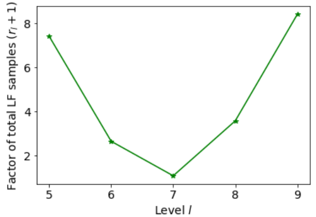
Figure 17. Factor of total LF samples ( r_l + 1 ) required by MLMF compared to number of HF samples for the Carrier-Greenspan test case, where r_l is (Eq. 25).
