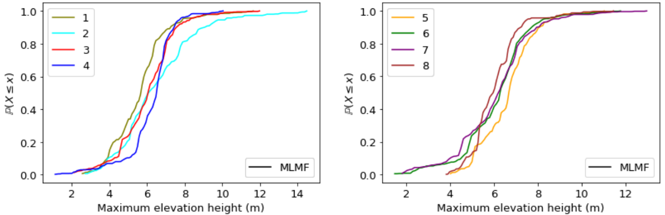
Figure 29. CDFs generated from MLMF outputs using the modified inverse transform sampling method (Eq. 29).
