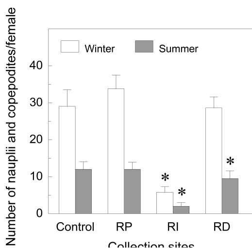
Figure 2. Chronic toxicity effects on copepod ( Nitokra sp.) reproduction, using sediments collected from the Rio Picinguaba (RP), Rio Itapanhaú (RI) and Rio Diana (RD) during the southern winter and summer of 2013. Data are the mean ( \pm SEM, N = 4) hatching rates (total number of nauplii and copepodites divided by total number of females). * P < 0.05 compared to the respective control group (sediment from Praia Engenho d'Água, São Sebastião Island).
