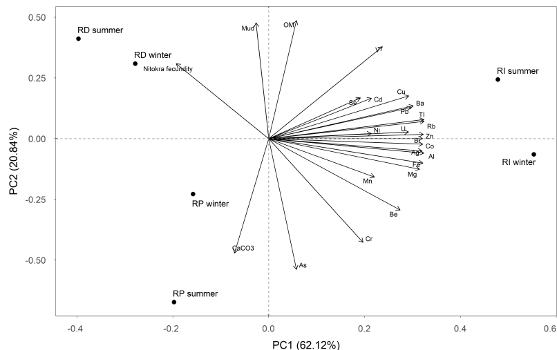
Figure 3. Principal components analysis of composition, elements and toxicity for sediment samples collected from Rio Diana (RD, severely contaminated site), Santos, Rio Itapanhaú (RI, moderately contaminated site), Bertioga, and Rio Picinguaba (RP, pristine site), Ubatuba, during the southern winter and summer of 2013.
