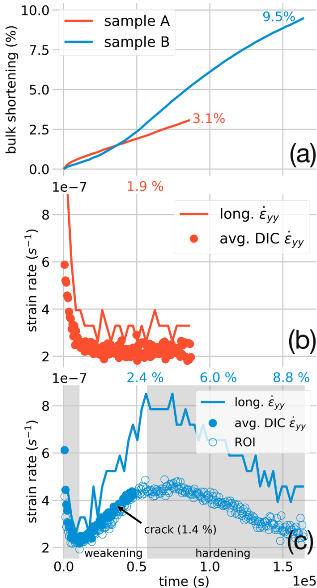
Figure 3. Evolution of strain and strain rate over time. For comparison, the time scale is the same in all plots. (a) Creep curves for samples A and B. Bulk shortening represents the finite longitudinal (engineering) strain parallel to the shortening axis. (b) Strain rate evolution of sample A determined via evolution with time of the finite longitudinal strain (line) and digital image correlation using the variation of the average (median) strain in the vertical direction \sigma_{yy} (markers). After a short primary creep, \sim 0.9\% , sample A experienced steady-state creep up to 3.1%. (c) Strain rate evolution of sample B. Due to the degradation of the speckle pattern quality with time, DIC-derived strain rates were estimated over the whole area only up to 2.4%. Focusing on a region of interest (ROI) where the speckle pattern preserved a good quality (this ROI corresponds to the one shown in figure 4), we also determined the strain rates to completion (hollow markers). After a short primary creep ( \sim 0.4\% ), sample B underwent an accelerated creep stage (weakening) up to \sim 2.9\% and a deceleration creep stage (hardening) to completion at 9.5%. The different creep stages are highlighted by shaded areas. The equivalence between time and finite longitudinal strain is given at selected points for both samples at the top (in colour). The time at which the crack occurs in sample B is also indicated.
