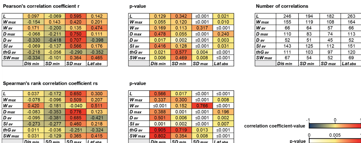
Figure 5: Heat maps for correlations of canyon morphometrics with the physiographic setting displaying values of Pearson's correlation coefficient r and Spearman's rank correlation coefficient r_s , and their respective p-values. L = canyon length; W_{max} = maximum canyon
