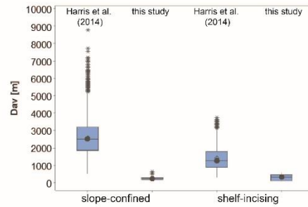
J. Average depth (Harris et al., 2014)
