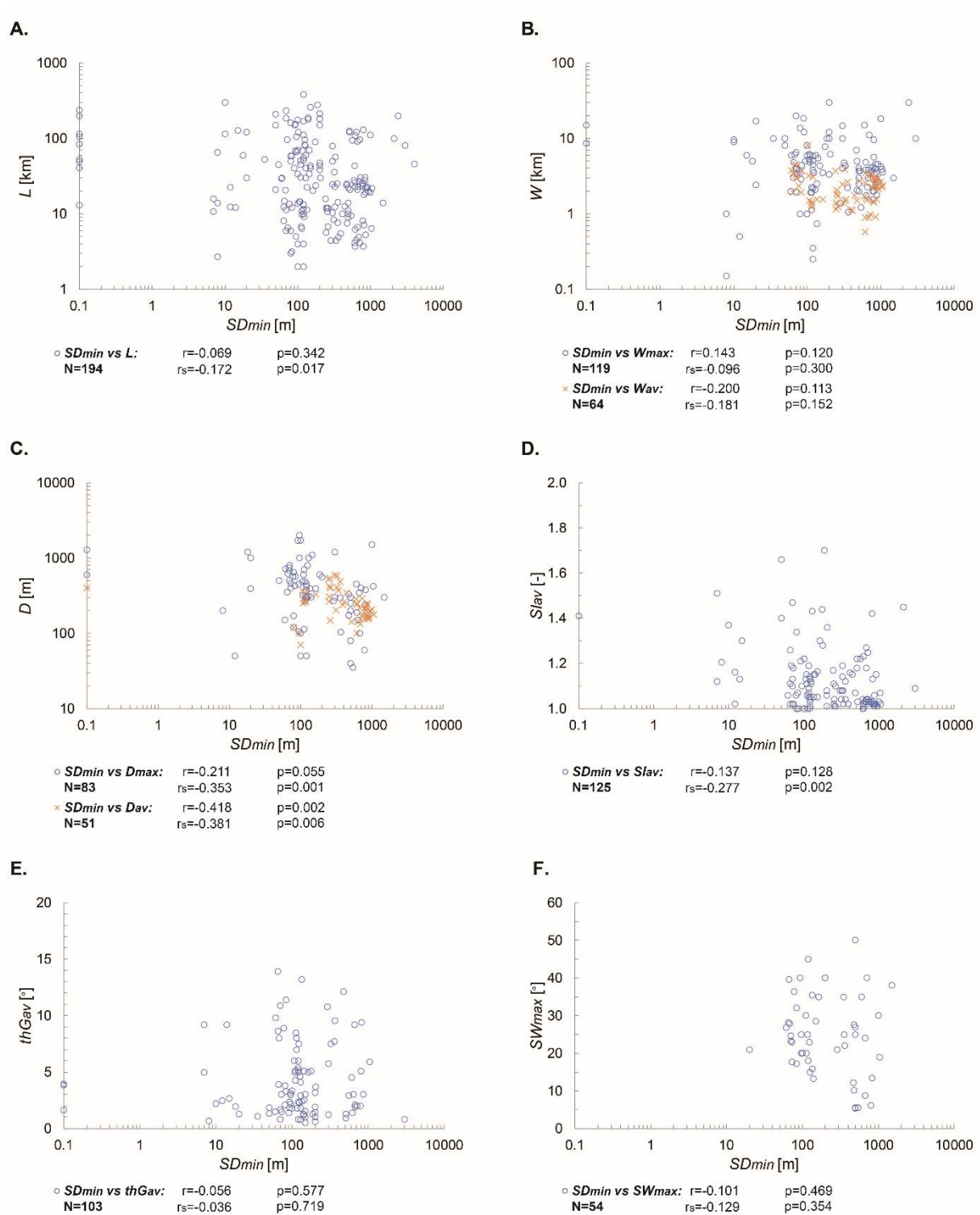
Fig. 7a-f: Scatterplots of seafloor depth at the top of the canyon and canyon morphometric parameters. N = number of correlations; r = Pearson's correlation coefficient; r_s = Spearman's rank correlation coefficient.
