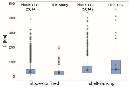
I. Length (Harris et al., 2014)
