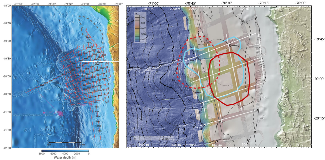
Figure S11. (left) Map showing location of seismic lines acquired during cruise MGL1610 (Tréhu et al., 2017). Numbers indicate positions of ocean bottom seismometers. Thick grey dashed line is the outline of the Arica/Iquique basin of Moberly et al. (1982) [also called the Tarapaca Basin by Gonzalez, 1989]. White box outlines the region shown on the right. (right) Detailed bathymetric map from swath bathymetry acquired during cruise MGL1610 overlain on the GMRT global elevation model. Note the narrowing of the swath as water depth decreases. Depth contours are shown at 500 m intervals and are dotted where interpolated between the swaths. White lines are the locations of seismic reflection profiles shown in Figure S12. Light blue line is the outline of the gravity low in the center of the ‘Mogi Doughnut’. Dashed red line is the 4 m slip contour from Duputel et al. (2015). Solid red line is the approximate outline of a distinct sub-basin located within the region interpreted to be by the much larger Arica/Iquique/Tarapaca basin. Subhorizontal, underformed reflections within a topographic basin suggest continuing basin formation subsidence within this sub-basin.
