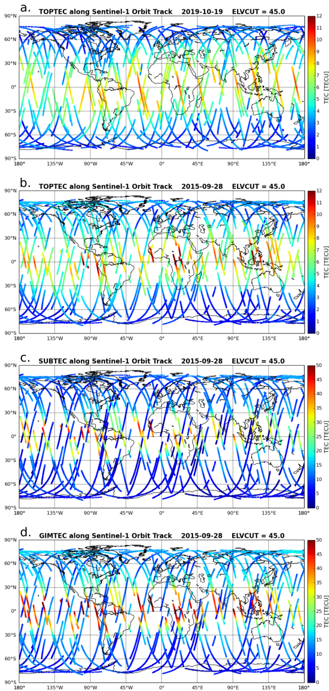
Figure 9. GNSS-based vertical TEC along Sentinel-1A/B orbits on 19 October 2019 (close to solar minimum) and 28 September 2015 (close to the last solar maximum). (a-b) Topside TEC (from SAR orbits to GNSS orbits). (c) Sub-orbital TEC (from the ground to SAR orbits). (d) Total TEC (from the ground to GNSS orbits). ELVCUT: elevation cutoff angle in degrees. The 10-min window culling is not applied. The data discontinuity at some locations and/or times may be caused by the elevation angle cutoff, inadequate amount of data for averaging or fitting, and possible removal of noisy data.
