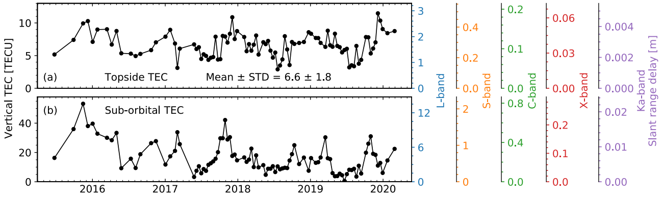
Figure 16. Impact of topside TEC on the geolocation of L (1.257 GHz, NISAR), S (3.2 GHz, NISAR), C (5.405 GHz, Sentinel-1), X (9.65 GHz, TerraSAR-X) and Ka-band (35.75 GHz, SWOT) SAR at \sim 6 pm local solar time. (a) Estimated topside TEC time series using GPS receivers onboard Sentinel-1 platforms for the ascending track 149 at \sim 6 pm local solar time. (b) Estimated sub-orbital TEC as the difference between the total TEC from JHR GIM and topside TEC. Axes on the right: predicted range delay for different radar carrier frequencies assuming an incidence angle of 42^\circ of the line-of-sight vector on the ground following equation (6-11).
