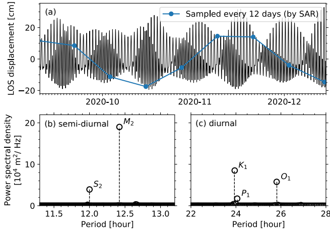
Figure 4. Solid Earth tides at Los Angeles, California [N34°, W118°]. (a) LOS displacement time series assuming an incidence angle of 42° and an azimuth angle of 100°. Blue dots represent displacement sampled by SAR sensor with a re-visit time of 12 days. (b-c) Power spectral density of (a) in the semi-diurnal and diurnal frequency ranges, respectively. K_1 , M_2 , O_1 , P_1 , S_2 are the Darwin symbol of the tidal constituents.
