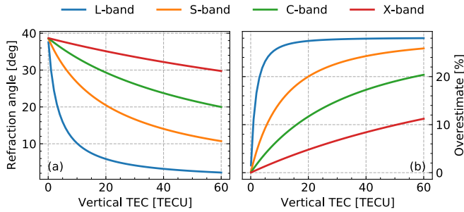
Figure 8. Impact of refraction on ionospheric range delay as a function of the vertical TEC for a constant incidence angle of 42^\circ on the ground. (a) Refraction angle of the LOS vector at IPP based on equation (8-11). (b) Percentage of overestimated ionospheric range delay for ignoring the refraction effect. Lines are color-coded for different radar frequencies.
