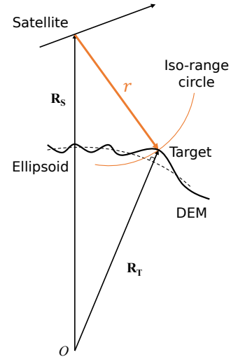
Figure 2. Geometry of the Doppler centroid plane for SAR geolocation. \mathbf{R}_S is the position vector of the SAR platform. \mathbf{R}_T is the position vector of the target on the ground. r is the slant range distance.
