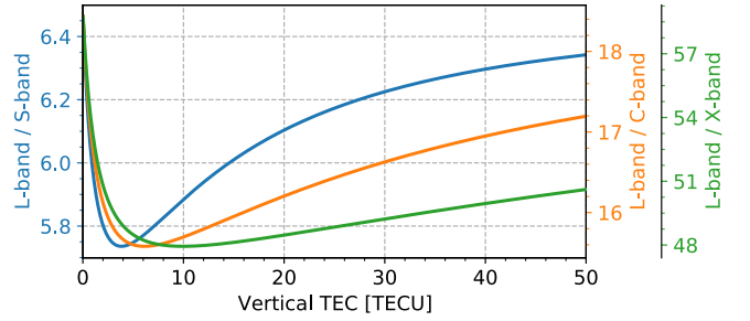
Figure 7. Ionospheric range delay as a function of vertical TEC. (a) Ionospheric delay for different radar frequencies and different range bandwidths. (b) Ratio of the ionospheric sensitivity between L-band and S, C, X-band. Calculations are based on equation (6-11) assuming a constant incidence angle of 42^\circ of the LOS vector on the ground.
