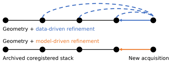
Figure 1. Updating strategies for the stack coregistration of SAR big-data. Solid arrows represent the mis-registration refinement of the new acquisition. Dashed lines represent the redundant pairs of data-driven mis-registrations used to estimate the refinement of the new acquisition.
