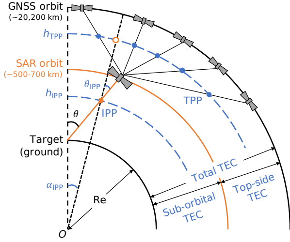
Figure 5. Mapping geometry of GNSS-based TEC products. R_e is the Earth radius, IPP for ionospheric piercing point, TPP for topside ionospheric piercing point. \theta and \theta_{IPP} are the incidence angle of the radar LOS vector on the ground and at IPP, respectively. \alpha_{IPP} is the geocentric angle distance between the target and IPP.
