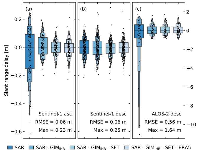
Figure 15. Distribution of the relative range delay time series after routine geolocation error corrections. The letter-value plot [53] showing up to 95% of the data overlaid by the scatter plot showing all the data. Labels describe the relative geolocation accuracy in range direction in terms of RMSE and maximum magnitude. For Sentinel-1 in (a and b) the S1A/B range bias has been removed. For Sentinel-1 descending track in (b), outlier acquisition at 2015-04-02 is excluded.
