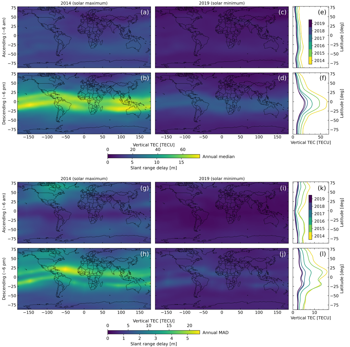
Figure 10. Global distribution of ionospheric range delays during the last half solar cycle (from 2014 to 2019) based on the expected science orbits of NISAR (6 am ascending and 6 pm descending nodal times) using JLR GIM. Top and bottom panels: the annual median and median absolute deviation (MAD) of vertical TEC, respectively. Profiles on the right: the average vertical TEC variation along the latitude for each year. The corresponding slant range delay (range geolocation error) is calculated based on NISAR L-band frequency with an incidence angle of 42^\circ of the line-of-sight vector on the ground. For NISAR S-band SAR, the range delay will be \sim 6 times smaller in magnitude. For Sentinel-1 with the similar dusk/dawn acquisition strategy, the ionospheric impact will be similar but with relatively stronger effects on its ascending orbits and with \sim 17 times smaller magnitude in range delay.
