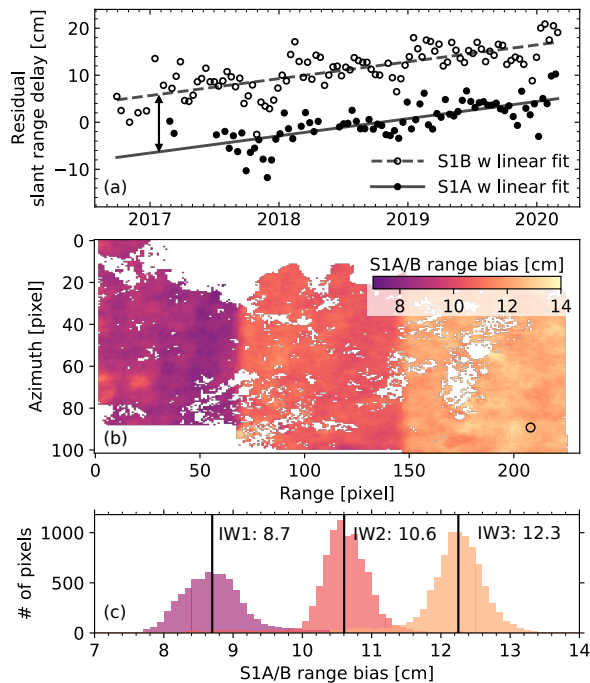
Figure 14. Range bias between S1A and S1B. (a) Residual range delay time series after correcting for SET and troposphere for one pixel (black circle in (b)) in Sentinel-1 descending track 156 in Chile. Only the time period with both platforms regularly acquiring images (from 2016-09-29 to 2020-02-29; 77 and 97 images from S1A and S1B, respectively) is shown and used for the bias estimation. (b) Map of the estimated range bias. (c) Histogram of (b) for each subswath with black vertical line for the median value.
