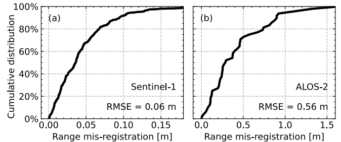
Figure 19. Cumulative distribution of range mis-registration for geometrical coregistration with model-driven refinement from ionosphere (JHR GIM), troposphere (ERA5) and SET. (a) Sentinel-1 with 304 acquisitions from ascending and descending orbits, excluding the outlier acquisition at 2015-04-02. (b) ALOS-2 with 49 acquisitions from descending orbit.
