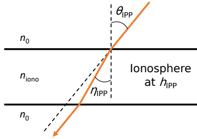
Figure 6. Refraction geometry of microwave signal traveling through the ionospheric layer with refractive index of n_{iono} . n_0 is the refractive index of the vacuum. \theta_{IPP} and \eta_{IPP} are the incidence and refraction angle of the radar LOS vector at IPP, respectively.
