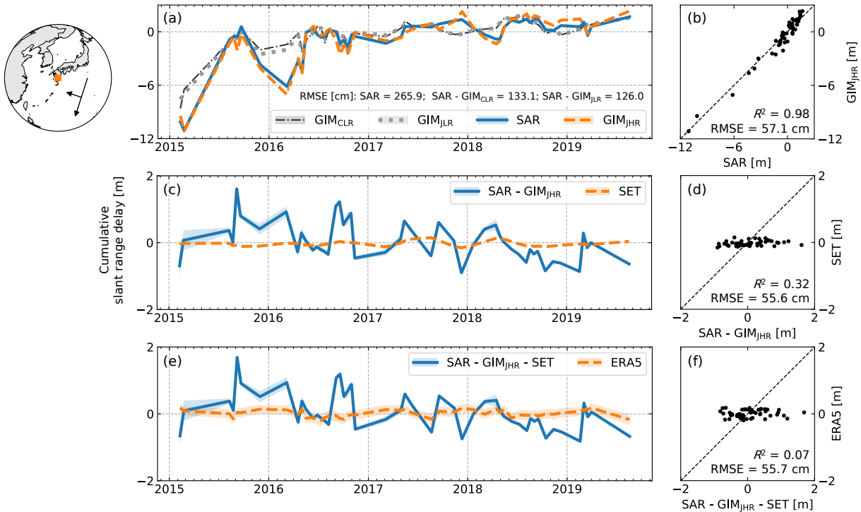
Figure 13. Similar to Fig. 11, but for the L-band ALOS-2 descending track 23 in Japan with SAR acquisition at 03:19 UTC ( \sim 12 pm noon local solar time). The median and MAD values from the whole image are used.
