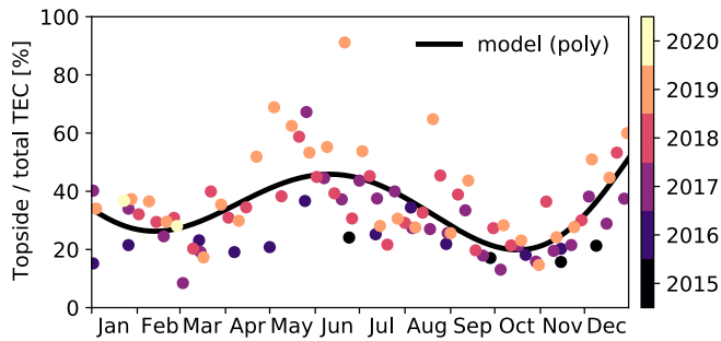
Figure 17. Ratio of topside TEC to total TEC for the C-band Sentinel-1 ascending track 149 in Chile ( \sim 6 pm local solar time). Median value: 31%. Solid line: polynomial fit as a function of the day of the year.
