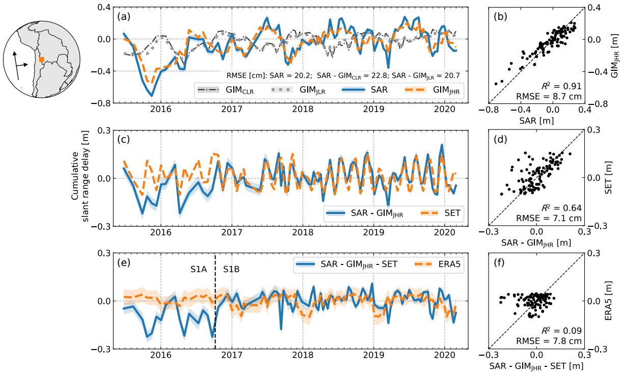
Figure 11. Progressive comparisons between the observed and predicted relative range geolocation errors for the C-band Sentinel-1 ascending track 149 in Chile. Upper left inset: dataset location. Top panel: the observed range delay (observation) from SAR image cross correlation (solid blue line) versus the predicted range delay from ionosphere (model prediction) using JHR GIM (dashed orange line), JLR GIM (dotted gray line) and CLR GIM (dash-dotted black line). Central panel: the observation after correcting for ionosphere using JHR GIM versus the model prediction from SET. Bottom panel: the observation after correcting for ionosphere and SET versus the model prediction from troposphere using ERA5. For each panel, the observation time series is shifted by its median value, the model prediction time series is shifted by its median difference with the observation. The median value and the three times median absolute deviation (MAD) range within a window of 20 by 20 pixels centered at [S21.30°, W67.39°] are used. SAR acquisition at 23:07 UTC ( \sim 6 pm local solar time).
