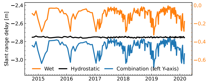
Figure 3. Single path absolute tropospheric delay time series in LOS direction at the acquisition time for Sentinel-1 descending track 156 at [S21.29°, W69.22°] in Chile using ERA5. Orange, black and blue lines present contributions from the wet air, dry air (hydrostatic) and the combination of both, respectively. The denser sampling from September 2016 onward is due to the addition of Sentinel-1B.
