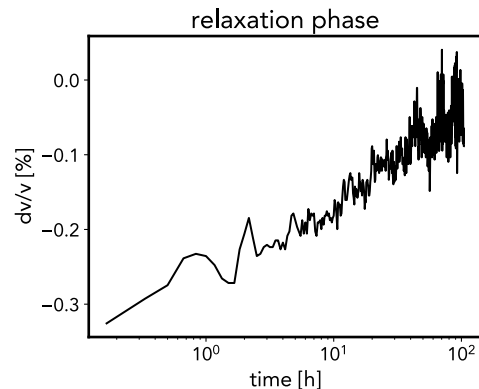
Figure 8. Relaxation phase recorded by the PESO array. The recovery phase shown in Fig. 4 using all the combinations is here plotted in a log-linear plot to emphasize the characteristic slow dynamics recovery.
