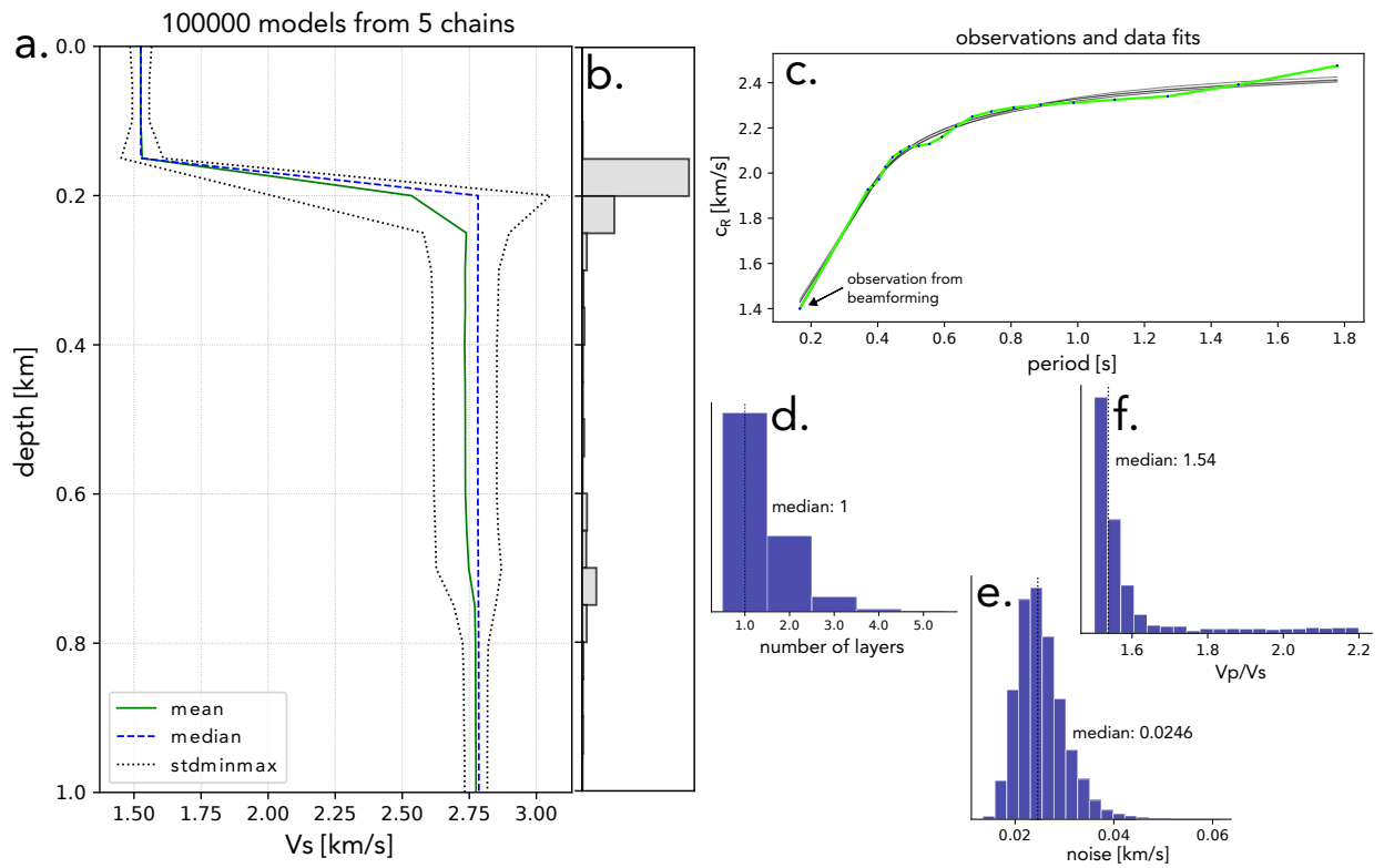
Figure 5. Inversion results when adding the observation from the beamforming method. a. Inferred shear velocity profile interpolated at a 50 m resolution. Green and blue lines shows the mean and the median value of the best retained models. Dashed black lines indicated the standard deviation. b. Histogram of the depth of the inferred layer structures c. The green line shows the dispersion curve that we use for the inversion, the other curves showing the best fit obtained for each chains. Histograms corresponding to the other inverted parameters are shown in d. for the number of layers, in e. for the noise level in the measurements and in f. for the V_p/V_s ratio.
