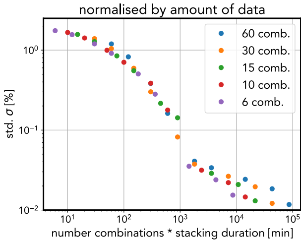
Figure 6. Noise in the seismic velocity time-series normalised by the total amount of used seismic data. Data are the same than in Figure 5a but normalised by the total length of the seismic traces.
