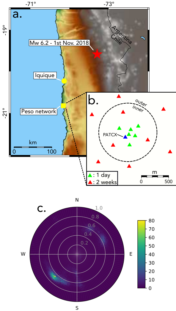
Figure 1. Map of the study area and beamforming analysis. a. Location of the PEsO array relative to Chile. The red star indicates the epicenter of the 1st of November 2018 earthquake. b. Geometric setting of the PEsO array. The blue triangle stands for the permanent PATCX station. The circle indicates our convention for the inner ring and the outer ring for this study. c. Results of the beamforming analysis. Colorbar indicates the relative energy level that is reported on the azimuthal plot.
