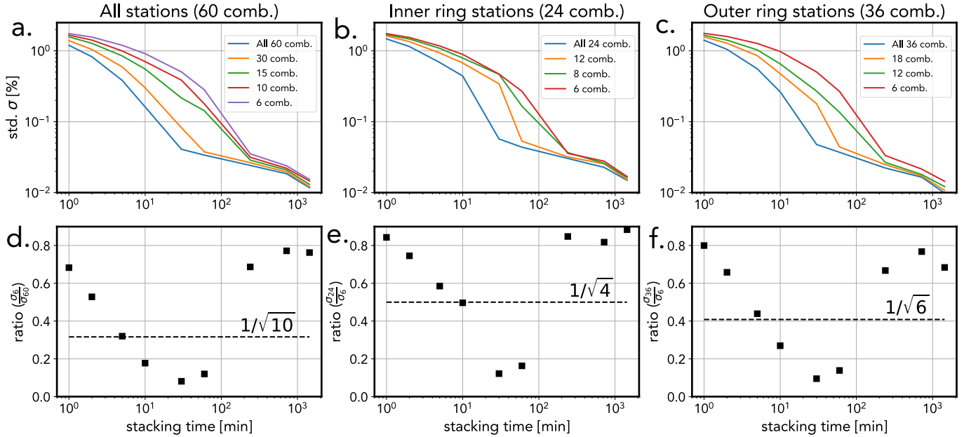
Figure 5. Standard deviations of the dv/v changes prior to the earthquake (from the 22nd of October to the 1st of November) obtained using different stacking durations and number of combinations a. Curves obtained using all single-combinations in the network. For each stacking duration, the mean of the standard deviation of the respective combination subset. The subsets are characterised by a number of combination shown as an inset label. We show on b. and c. the same plot but using only the inner ring stations and the outer ring stations respectively. The subplots d. , e. and f. show the corresponding ratio between the standard deviation using all considered combinations and when using only six. The dashed line shows the theoretical reduction of the standard deviation for independent variables with the same mean and variance.
