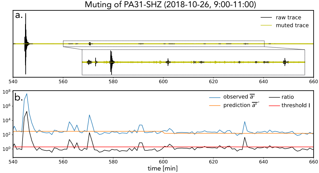
Figure 2. Muting of the seismic trace, an example. a. The black trace shows two hours of vertical data at the station PA31. The other trace stands for the muted version with a close-up for clarity. b. The blue line indicates the estimates of \beta_2 based on the average squared envelope of the raw trace shown in a at a 1-minute resolution. Orange line shows the prediction of \beta_1 based on the squared envelope predicted by the log-Rayleigh distribution at each hour. The ratio of the observation and the prediction is shown in black with the red line indicating the threshold used for muting the raw trace.
