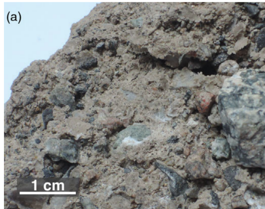
Figure 6. Geological media observed in the field. The geology hints at clasts embedded in a matrix containing large amounts of evaporites (likely gypsum and halite). The picture is taken from the study of Sens-Schönfelder & Eulenfeld (2019) .
