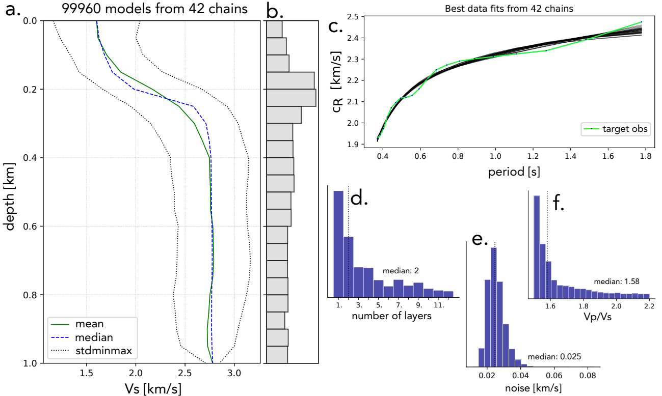
Figure 7. Inversion of the 1D shear velocity profile and corresponding target dispersion curve. a. Inferred shear velocity profile interpolated at a 50 m resolution. Green and blue lines shows the mean and the median value of the best retained models. Dashed black lines indicated the standard deviation. b. Histogram of the depth of the inferred layer structures. c. The green line shows the dispersion curve that we use for the inversion, the other curves showing the best fit obtained for each chains. Histograms corresponding to the other inverted parameters are shown in d. for the number of layers, in e. for the noise level in the measurements and in f. for the V_p/V_s ratio.
