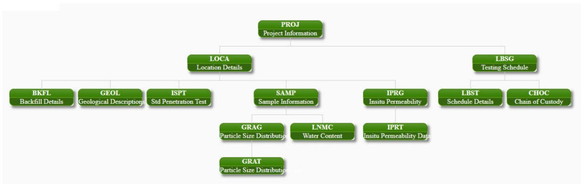
Figure 1: Simplified schematic of AGS4 data structure
