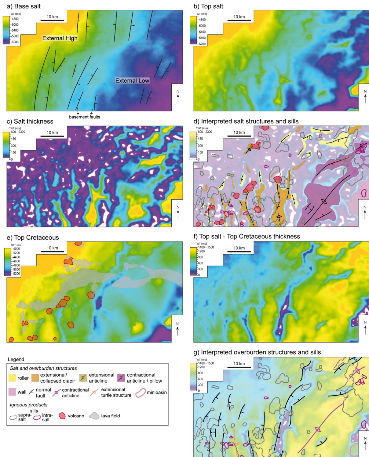
Figure 12. Time maps of the 3D volume. a) Base-salt surface map, which vary from -3900 to -6400 ms (TWT), with the underlying basement faults and structures (External High and External Low; Guardado et al., 2000). b) Top-salt surface map, ranging from -4500 and -6300 ms (TWT). c) and d) show salt isochron thickness map, with values ranging from 0 to 2500 ms (TWT) defining salt welds and salt structures, interpreted in (d). e) Top Cretaceous surface map, varying from -3600 and -5500 ms (TWT), with the interpreted volcanoes and lava flows (see figure 4c). f) and g) show the isochron thickness map between the top salt and top Cretaceous, which varies from 0 to 1500 ms (TWT), defining overburden structures interpreted in (g).
