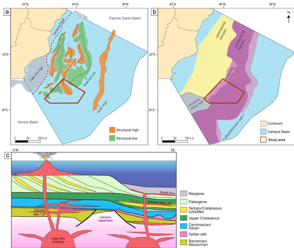
Figure 2. (A) Rift-related structural framework of Campos Basin, redrawn from Guardado et al. (2000) ; Outer High and Cabo Frio High locations from Fetter (2009) . (B) Salt-related structural provinces, modified from Davison et al. (2012) and Amarante et al. (2021) ; the location of the volcanics above salt (or Cabo Frio Volcanic Province, according to Mohriak et al., 2020 ) is from Meisling et al. (2001) . (C) Schematic cross section showing the Late Cretaceous to Paleogene magmatic events in the Campos Basin (redrawn from Mohriak et al., 2020 ).
