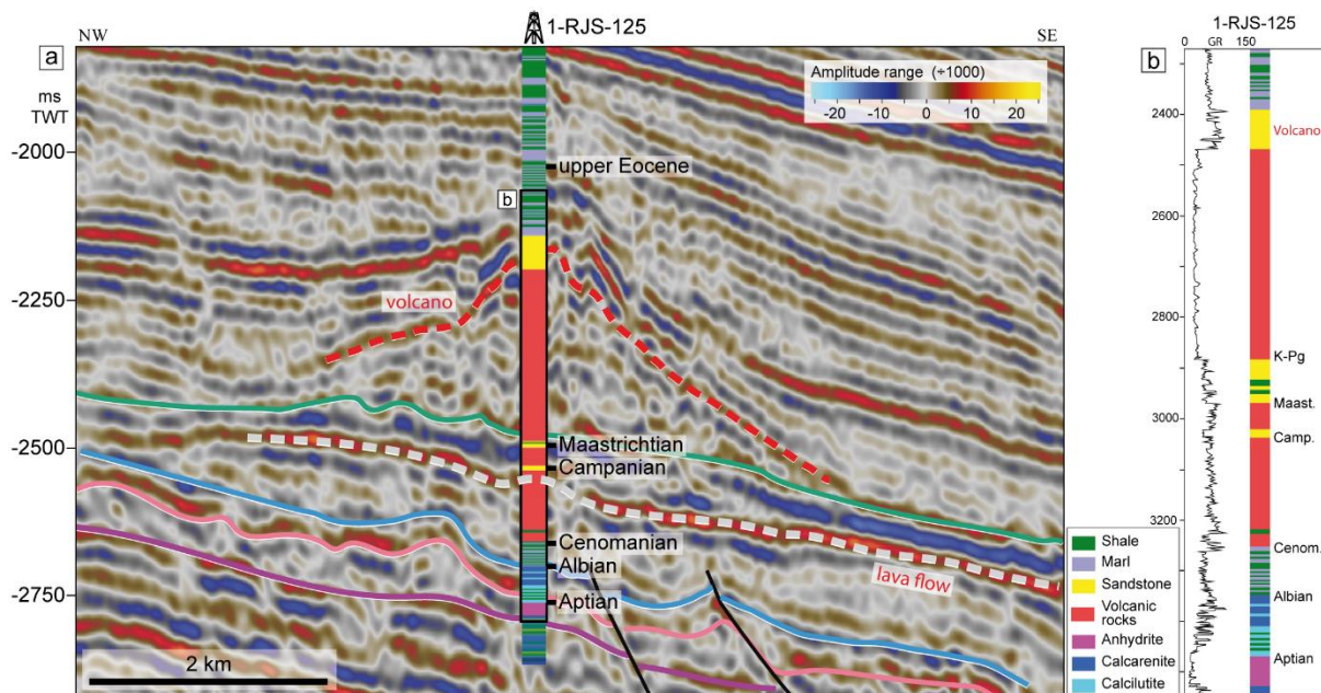
Figure 9. (a) Seismic line showing the well 1-RJS-125 drilled through a volcano, with the positions of the ages Aptian, Albian, Cenomanian, Campanian, Maastrichtian (top Cretaceous) and upper Eocene; the top of the volcano is indicated by a red dashed line. (b) Lithology and gamma ray curves of the well 1-RJS-125. These are also shown in Mohriak et al., 2021 (see their figure 20).
