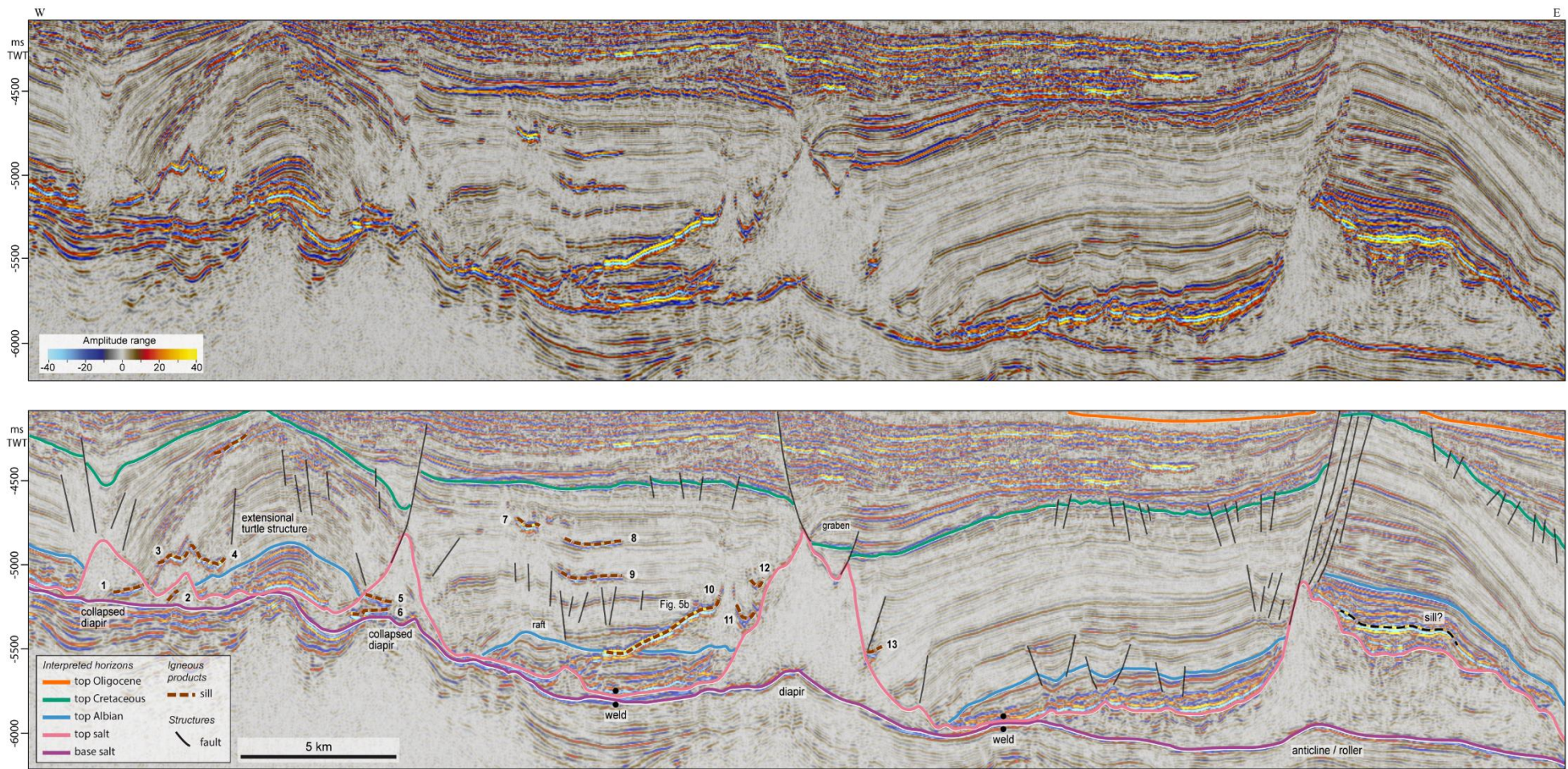
Figure 6. Inline seismic section (W-E). The lower section shows the interpreted seismic horizons, sills and faults. The sills are numbered to facilitate indications in the text. The main salt and overburden structures are labeled. See figure 3 for location. Seismic data supplied by ANP.
