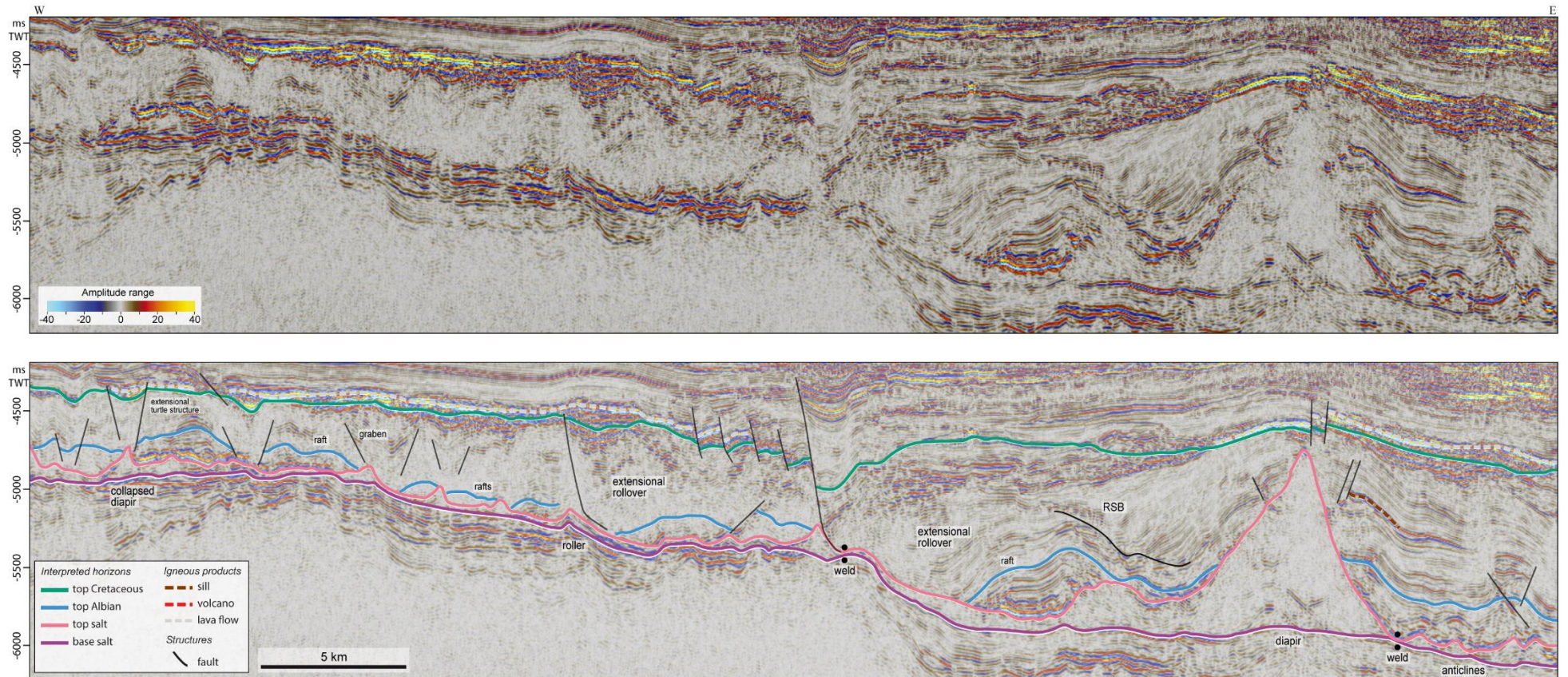
Figure 10. Inline seismic section (W-E). The lower section shows the interpreted seismic horizons, igneous products and faults. The sills are numbered to facilitate indications in the text. The main salt and overburden structures are labeled. See figure 3 for location. Seismic data supplied by ANP.
