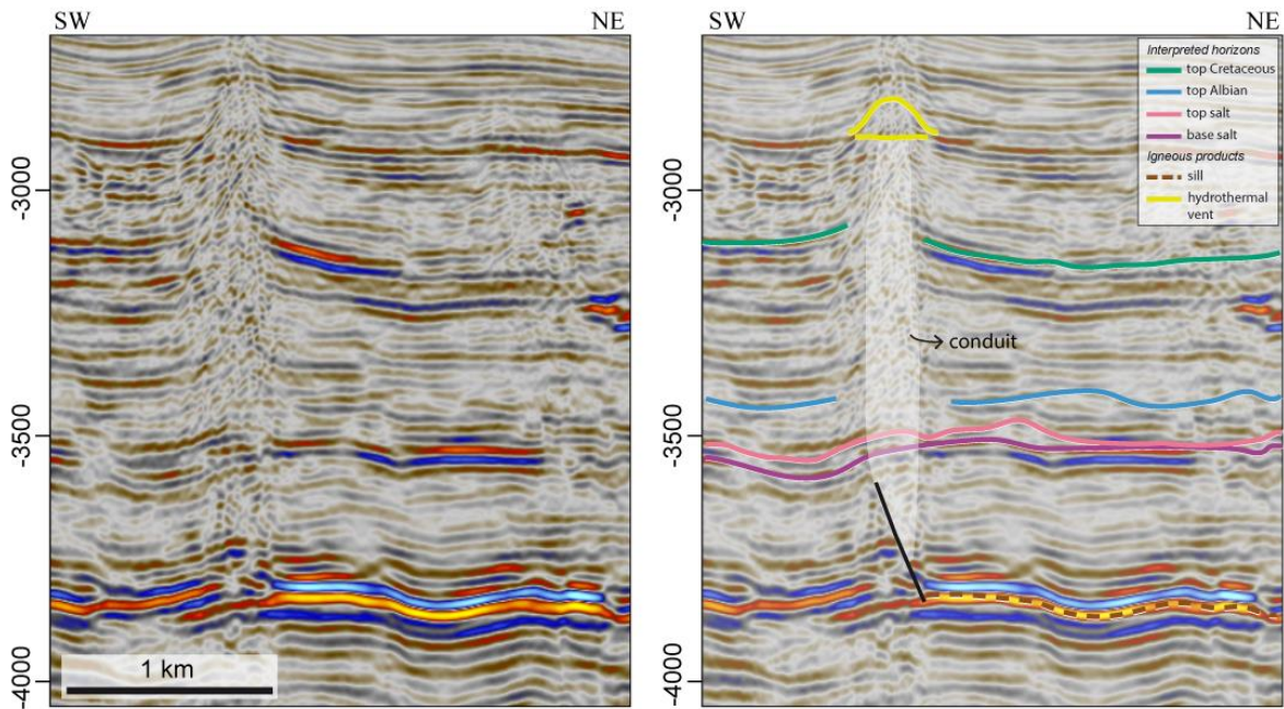
Figure 11. Uninterpreted (left) and interpreted (right) seismic section, showing the interpreted seismic horizons, sill and hydrothermal vent.
