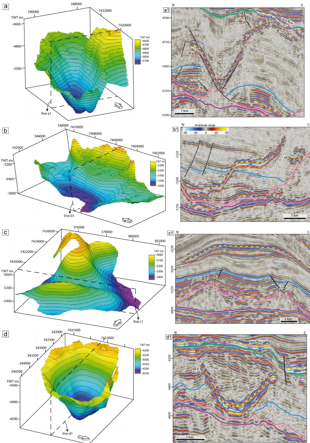
Figure 5. (a) 3D view of a saucer-shaped (locally fault block, see Figure 5a1 ) (b) 3D view of a planar transgressive sill; (c) 3D view of a layer parallel sill; (d) 3D view of a saucer-shaped sill. a1, b1, c1 and d1 show inlines seismic sections (W-E) highlighting the geometries of the selected sills. See figure 4d for their location.
