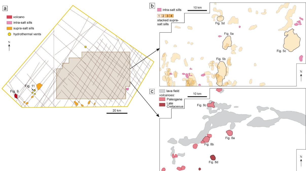
Figure 4. (a) Interpreted volcanic field, hydrothermal vents, intra-salt sill and supra-salt sills on the 2D seismic data; (b) interpreted intra-salt and supra-salt sills on the 3D volume; (c) interpreted volcanoes and lava field on the 3D volume. The igneous products shown in figures 5, 8, 9 and 11 are labelled.
