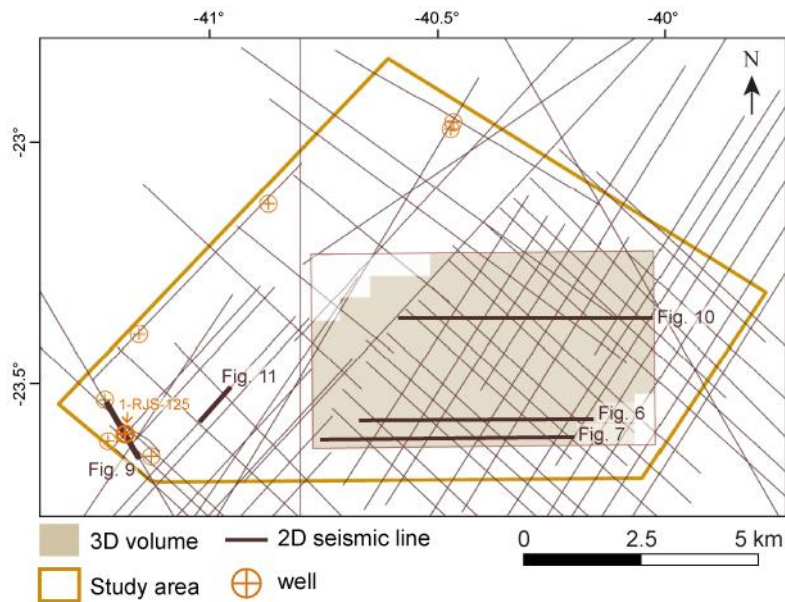
Figure 3. Dataset used in this study: 60 2D seismic lines (or lines segments), one 3D volume and 8 boreholes from the ANP data library. The seismic lines shown in figures 6, 7 and 10 are labelled, and also the well 1-RJS-125 shown in figure 9.
