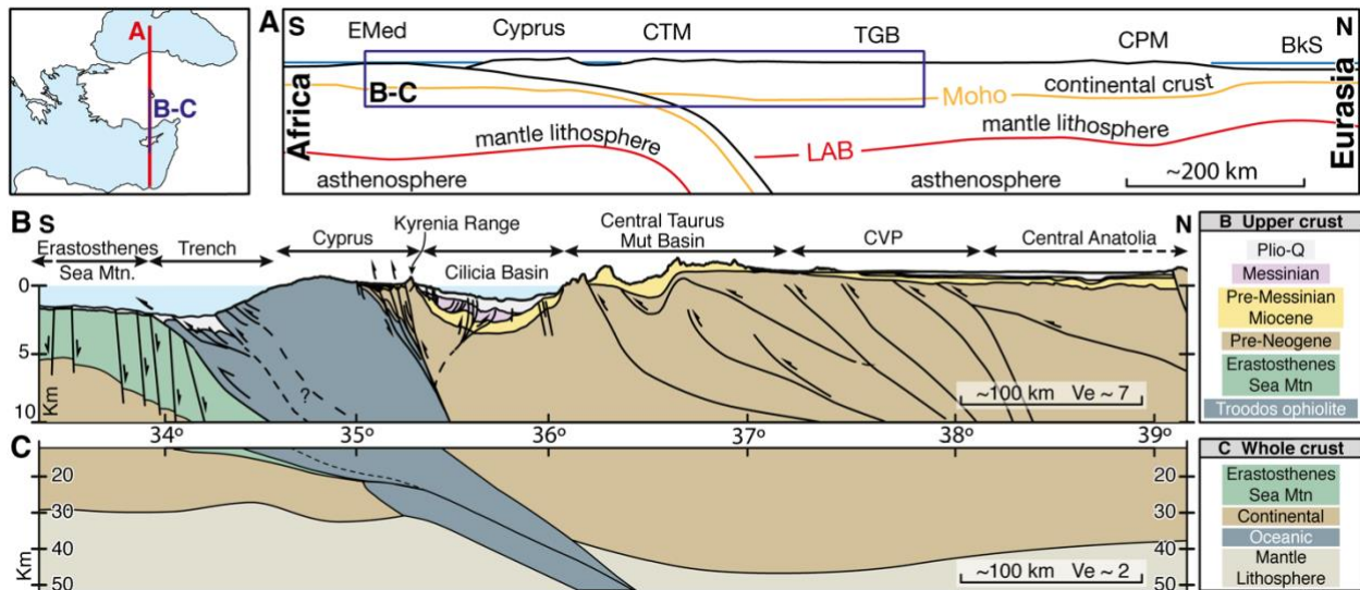
Figure 3. Transects along the Anatolian margin in Central Cyprus. Upper-crust and crustal-scale geological transects running N-S (650 km at around 33°30' E). The transects stretch from the Levantine Basin to the Tuz Gölü Basin across the Cyprus arc-trench, the island of Cyprus, the Cilicia Basin, the Central Taurus Mountains, and the Central Anatolian interior. The upper-left panel is a location map. Panel A is a transect across Central Cyprus and Anatolia, simplified from Stephenson et al. (2004), that has a topo-bathymetry with 3 times vertical exaggeration. EMed = East Mediterranean; CTM = Central Taurus Mountains; TGB = Tuz Golu Basin; CPM = Central Pontides Mountains; BkS = Black Sea. Panel B is the upper sector of the transect (up to 10 km depth), shown with ~7 km of vertical exaggeration, and Panel C is the crustal cross-section for the area. These transects integrate upper crustal studies (Robertson, 1998; Stephenson et al. , 2004; Calon et al. , 2005a, 2005b; Çiner et al. , 2008; McCay, 2010; Fernández-Blanco et al. , 2013) with the interpretation of several geophysical studies (Ates et al. , 1999; Mart & Ryan, 2002; Ergün et al. , 2005; Koulakov & Sobolev, 2006; Özeren & Holt, 2010; Mutlu & Karabulut, 2011; Abgarmi et al. , 2017; Delph et al. , 2017), as detailed in Fernández-Blanco (2014). CVP = Central Volcanic Province.
