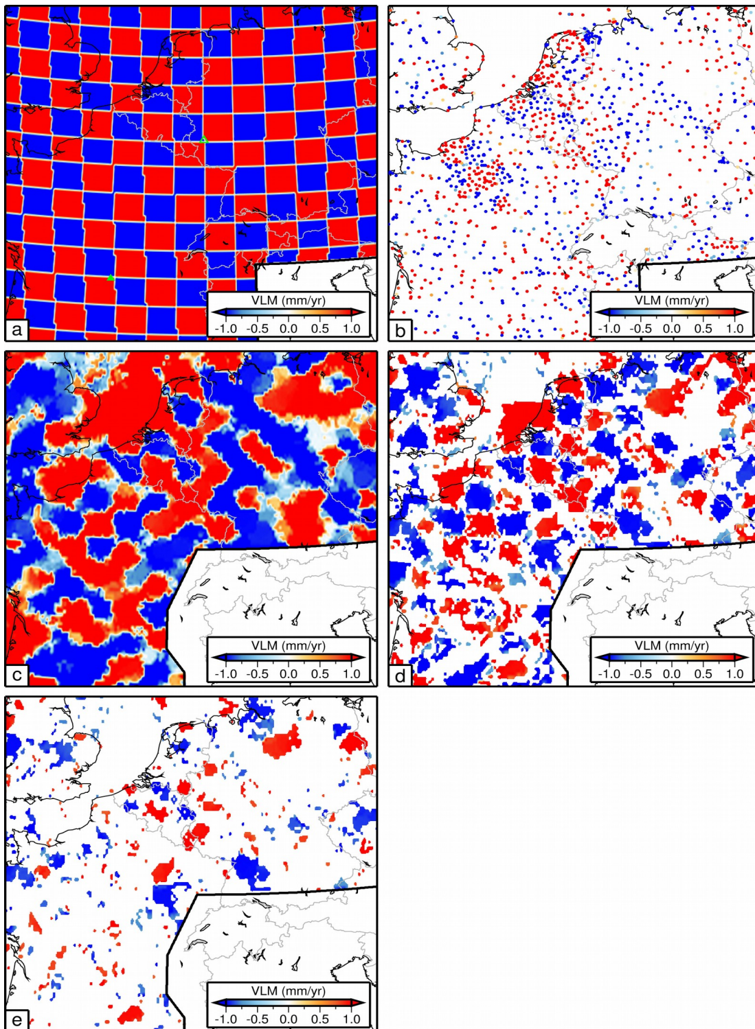
Supplementary Figure S1. a) Input chequerboard with alternating +1 and -1 \text{ mm yr}^{-1} VLM in 100 \times 100 \text{ km} cells. Open/closed triangle is location of Eifel and Massif Central, b) Imaged value at GPS locations using, c) Imaged VLM at 0.1^\circ grid, d) Imaged VLM where absolute value is \geq 1\sigma of imaged VLM, e) Imaged VLM where absolute value is \geq 2\sigma of imaged VLM.
