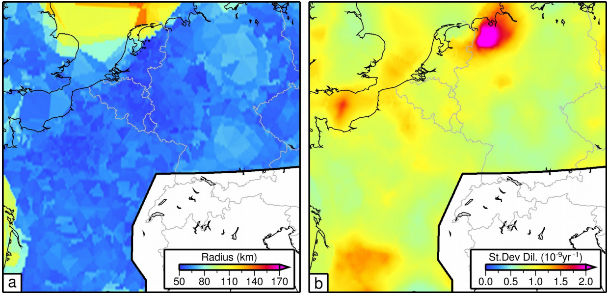
Supplementary Figure S4. a) Spatial scale of strain rate estimate expressed as the radius of a circle whose area is the median area of all triangles considered in the strain rate estimation. b) Standard deviation in the dilatation rate.
