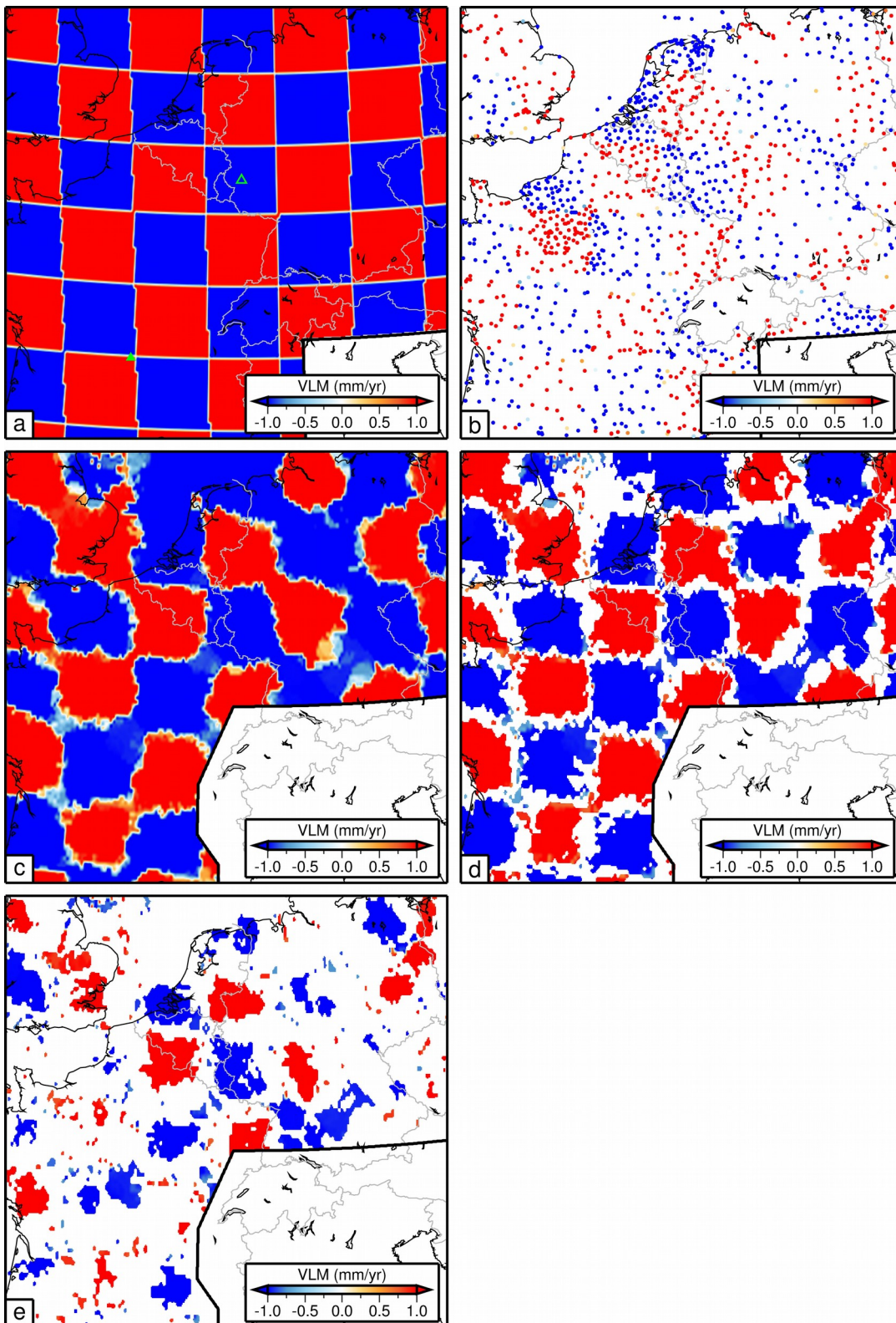
Figure 4. a) Input chequerboard with alternating +1 and -1 mm yr -1 VLM in 200x200 km cells. Open/closed triangle is location of Eifel and Massif Central, b) Imaged value at GPS locations using, c) Imaged VLM at 0.1° grid, d) Imaged VLM where absolute value is \geq 1\sigma of imaged VLM, e) Imaged VLM where absolute value is \geq 2\sigma of imaged VLM.
