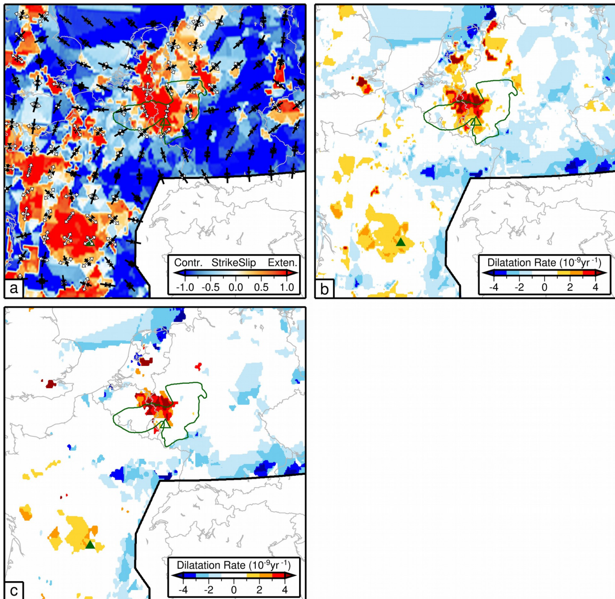
Supplementary Figure S9. This result is based on the MELD algorithm as originally presented (Kreemer et al. 2018).
