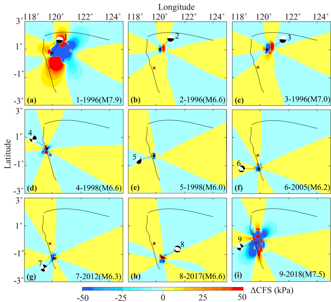
Figure S1: \Delta\text{CFS} Map at a depth of 13 km prior to and in 2018. The \Delta\text{CFS} Map prior to 2018 was a result of: (a) the 1996 earthquake ( M_w = 7.9 ); (b) the 1996 earthquake ( M_w = 6.6 ); (c) the 1996 earthquake ( M_w = 7.0 ); (d) the 1998 earthquake ( M = 6.6 ); (e) the 1998 earthquake ( M = 6.0 ); (f) the 2005 earthquake ( M = 6.2 ); (g) the 2012 earthquake ( M = 6.3 ); and (h) the 2017 earthquake ( M = 6.6 ). (i) The 2018 earthquake-induced co-seismic \Delta\text{CFS} ( M_w = 7.5 ). The faults are represented by black lines. The epicenters of the earthquakes Nos. 1–8 were marked with black stars. The epicenter of the 2018 Palu earthquake (No. 9) was marked with red star.
