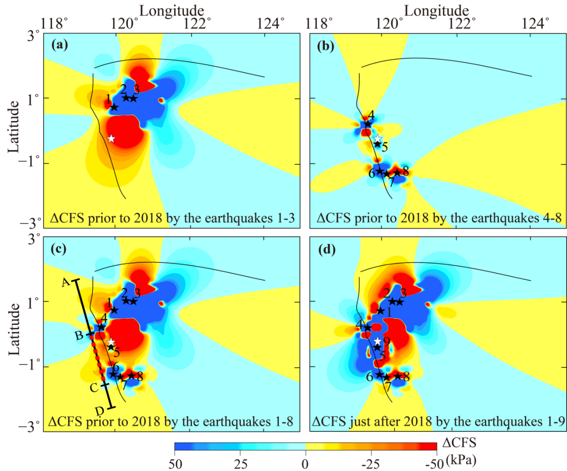
Figure 2: \Delta\text{CFS} map at a depth of 13 km prior to and after 2018. (a) The cumulative \Delta\text{CFS} map following the three earthquakes (Nos. 1–3) on the Minahassa thrust. (b) The cumulative \Delta\text{CFS} map following the five earthquakes (Nos. 4–8) on the Palu-Koro fault and the Poso fault. (c) The cumulative \Delta\text{CFS} map following eight earthquakes (Nos. 1–8) prior to the 2018 Palu earthquake. (d) The total \Delta\text{CFS} map following the nine earthquakes (Nos. 1–9) just after the 2018 Palu earthquake. The epicenters of the earthquakes (Nos. 1–8) are marked with black stars. The epicenter of the 2018 Palu earthquake (No. 9) is marked by red star.
