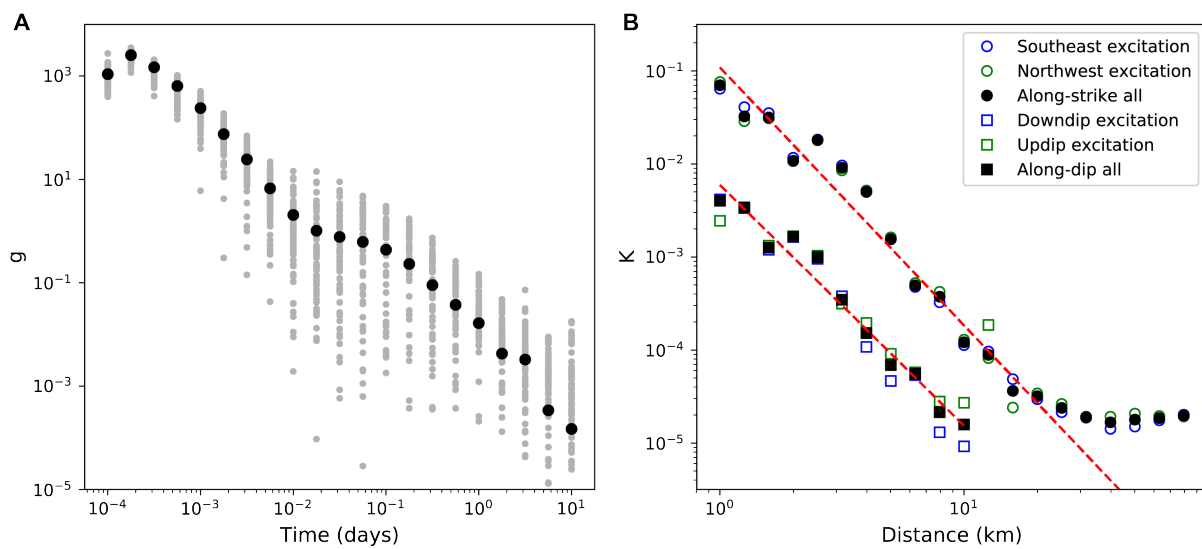
Figure S2: Obtained g and K when g is allowed to vary for different LFE families (see Materials and Methods). (A) g as a function of time. Gray dots show g for different LFE families. Black dots show the same g as in Fig. 2A for comparison. (B) K as a function of distance. Red dashed lines show least-squares fits giving K \propto d^{-2.8} and K \propto d^{-2.6} for along-strike and along-dip distances, respectively.
