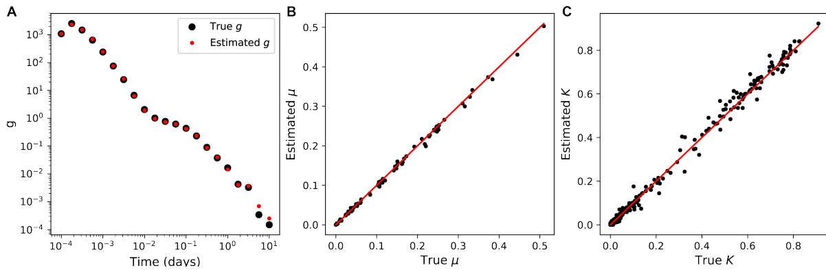
Figure S7: Comparison between true and estimated g , \mu , and K from synthetic catalog. Red lines have slope of 1.
