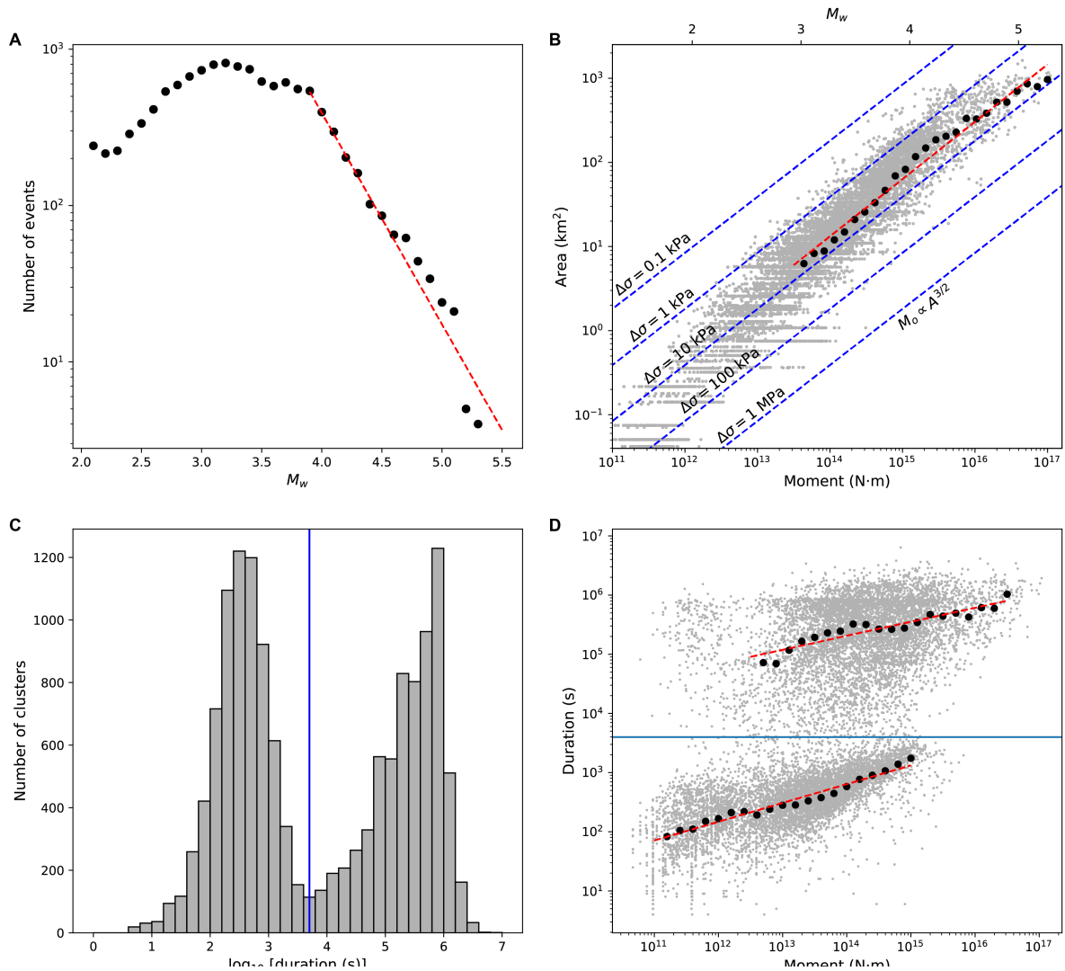
Figure S8: Obtained SSE scaling properties when g is allowed to vary for different LFE families (see Materials and Methods). (A) Noncumulative magnitude-frequency distribution of SSEs. Red dashed line shows maximum-likelihood fit giving a b value of 1.35 \pm 0.03 . (B) Relationship between seismic moment ( M_o ) and rupture area ( A ) of SSEs. Black circles show the median A for different M_o bins. Red dashed line shows least-squares fit giving M_o \propto A^{1.5} . Blue dashed lines show the M_o \propto A^{1.5} theoretical scaling relationships for circular cracks with different constant stress drops (38). (C) Histogram of SSE duration. Blue vertical line marks the local minimum ( 10^{3.7} seconds) used to separate the two populations of SSEs. (D) Relationship between M_o and duration ( T ) of SSEs. Blue horizontal line is the same duration boundary as in (C) that is used to separate the SSEs into two populations. For each SSE population, black circles show the median T for different M_o bins. Red dashed lines show least-squares fits giving M_o \propto T^{4.2} and M_o \propto T^{3.2} for the shorter and longer-duration SSE populations, respectively.
