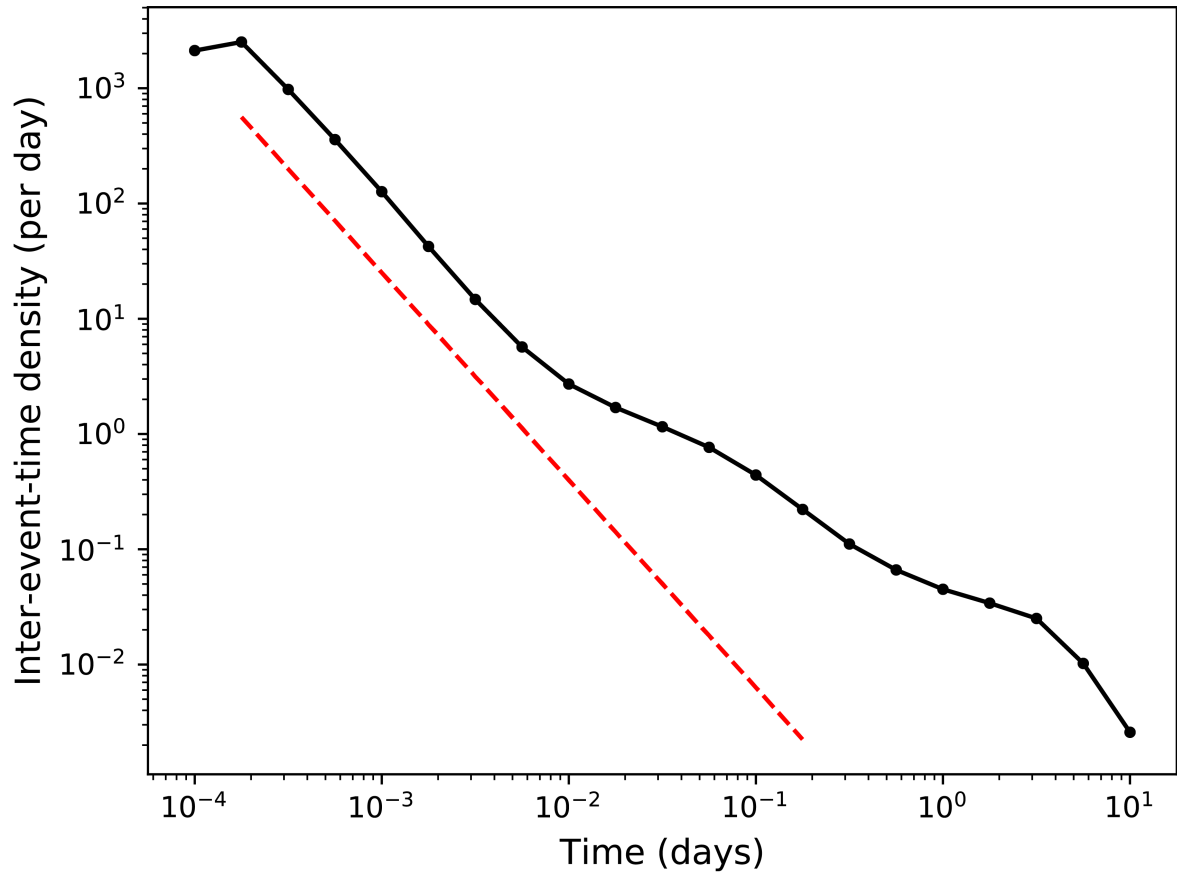
Figure S1: Stacked inter-event time distribution of all LFE families. Red dashed line has slope of -1.8.
