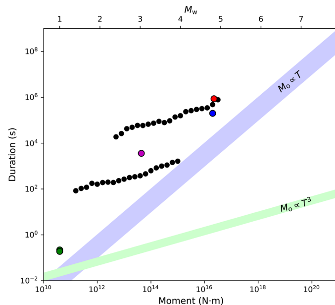
Fig. 4. Comparison between slow events on the San Andreas fault and proposed moment-duration scaling for regular (green bar) and slow (blue bar) earthquakes (12). Green circles, two LFE families (41); magenta circle, episodic creep events (45); blue circle, slow earthquake (46); red circle, average of 20 SSEs (7); black circles, SSEs in this study (same as in Fig. 3D).
